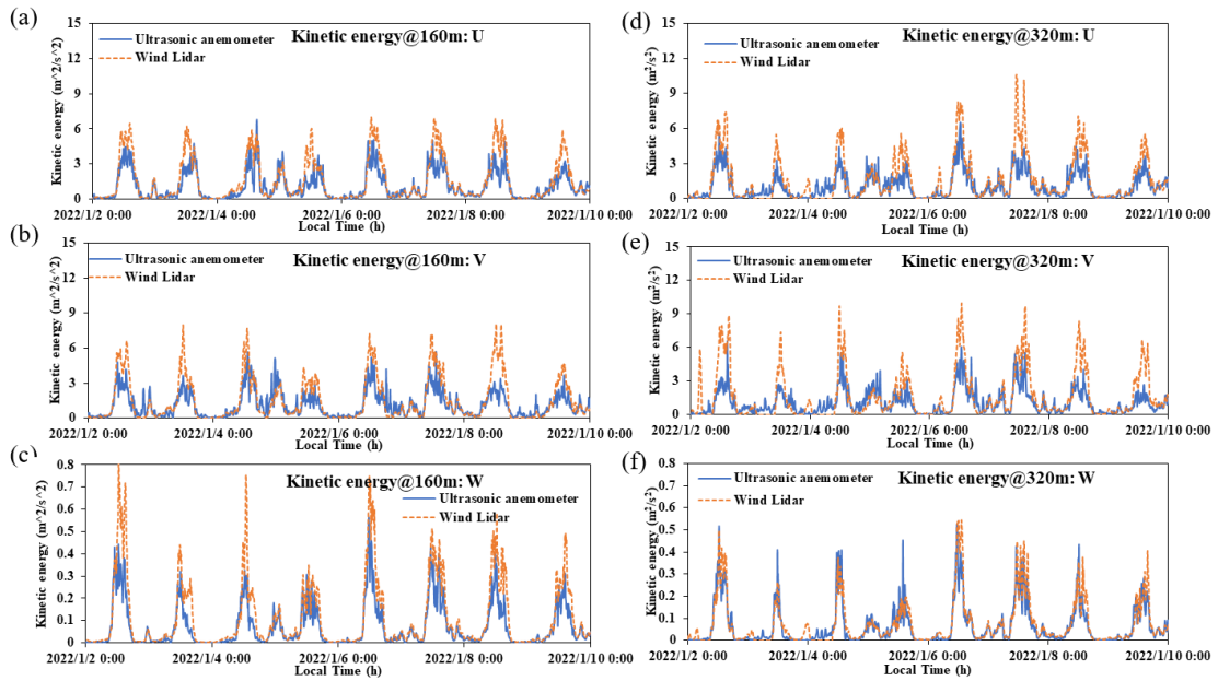
Figure 10. Comparison of the turbulent kinetic energy obtained from the wind lidar and three-dimensional ultrasonic anemometer from January 2nd to 10th, 2022 in the U , V , and W directions at the heights of 160 m (a)–(c) and 320 m (d)–(f).
