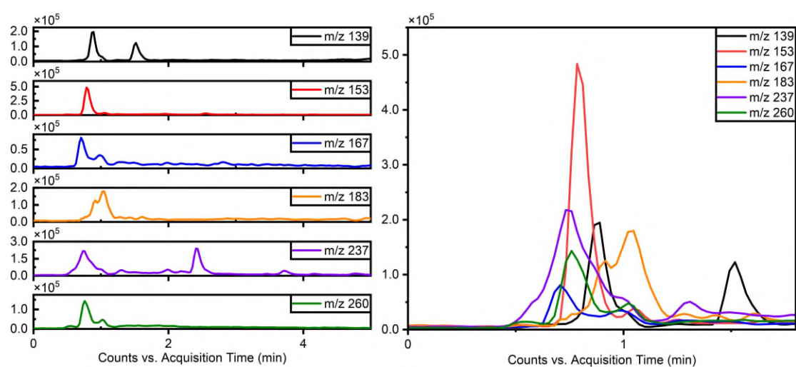
Figure 2. Chromatograms of iOSs with retention times less than 1 min.
