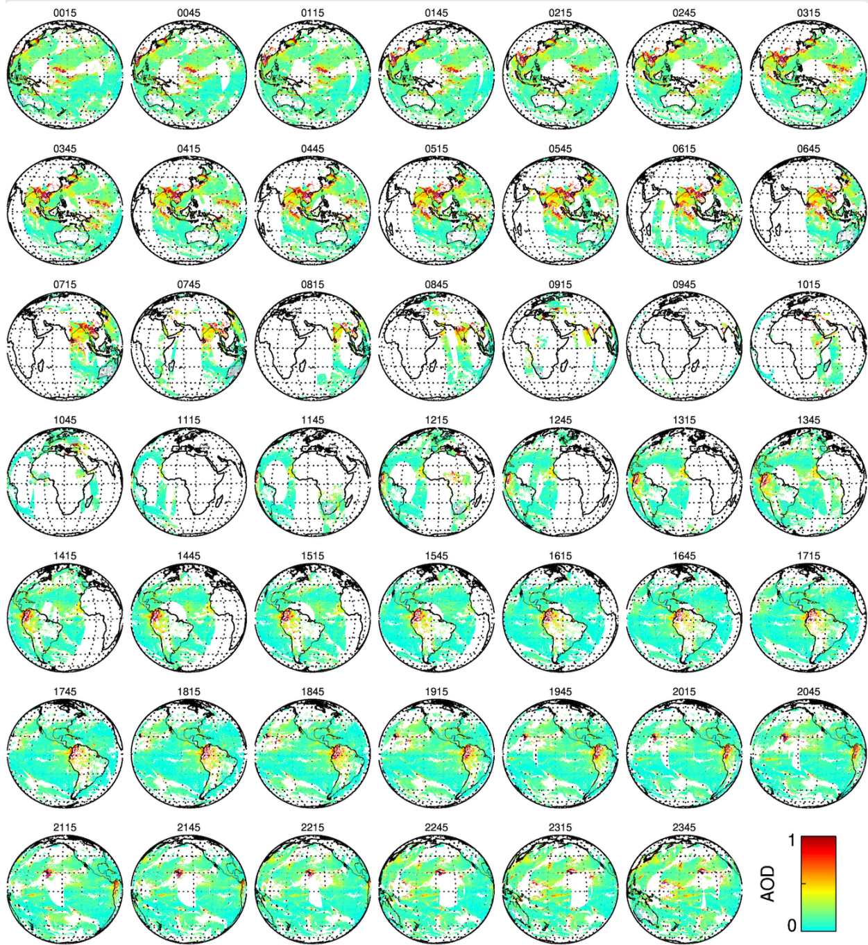
Figure 6. Example of 30 min coverage of merged aerosol data for one entire day (March 26, 2020, UTC). Each panel shows day light portion of earth at specific time (UTC) and available AOD retrieval from the six sensors merged product.
