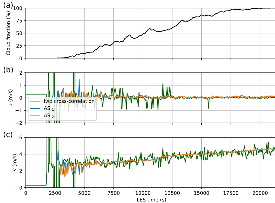
Figure 5. (a) cloud Cloud fraction from cloudmasks of ASI at P1 for LES times. Per timestep scene averaged cloud motion derived using cross-correlation of the lwp-field of the LES simulation and our cloud motion derivation based on feature matching for east to west motion u (b) and south to north motion v (c).
