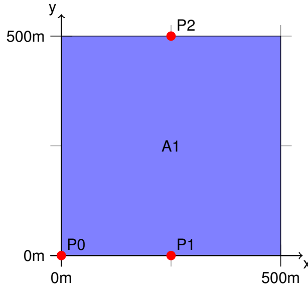
Figure 3. Measurement Spatial setup used within for the synthetic data-experiments with-conducted in this study. Shown are the ground coordinates within the LES domain. Synthetic all-sky images for-were generated at points P0, P1, and P2 as-well-as-DNI-references. Direct normal irradiance was simulated for point P1 and area A1. Nowcasts rely on images from P1 and P2 and predict values for point P1 and area A1.
