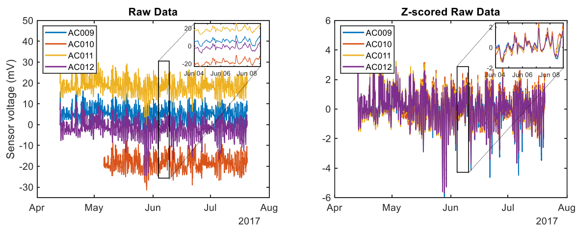
Figure 4. A comparison of raw NO 2 _A measurements before and after Z-score application, for each SU deployed at HAE.
