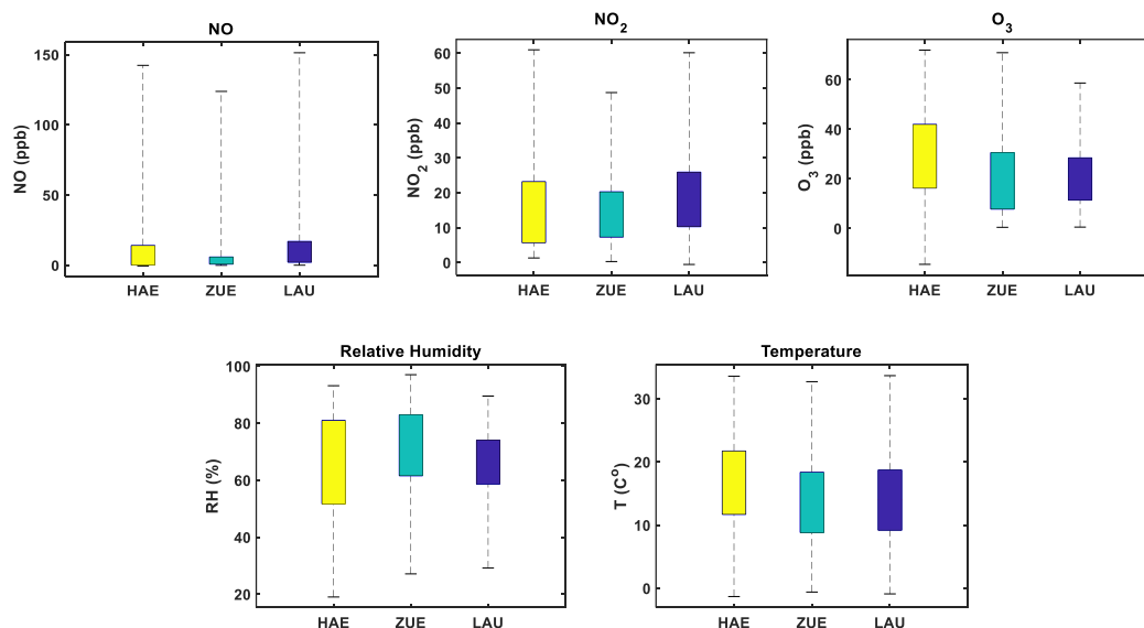
Figure 1. Box plots showing meteorological variables and pollutants concentrations at deployment sites using 10 min averaged data. The central line indicates the median, and the bottom and top edges of the box indicate the 25 th and 75 th percentiles of the data, respectively. The whiskers extend to the minimum and maximum values.
