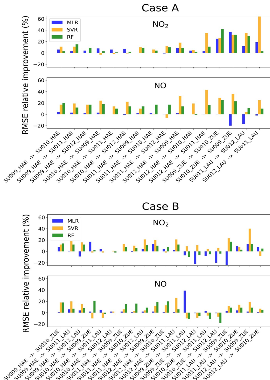
Figure 9. An illustration of the performance enhancement achieved by incorporating O 3 for both Cases A and B. X-axis represents (Primary SU → Secondary SU).
