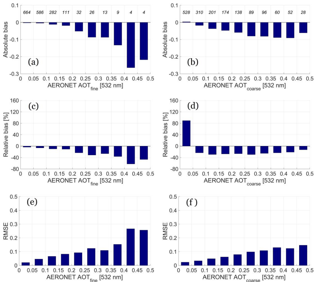
Figure 7: CALIPSO-based fine-mode (left column) and coarse-mode (right column) DOD at 532 nm absolute biases (Fig.7a/b), relative biases (Fig.7c/d), and Root Mean Square Errors - RMSE (Fig.7e/f) by AERONET fine-mode and coarse-mode AOT at 532 nm class of equal increment step of 0.05 for the AOT at 532 nm range extending between 0 and 0.5.
