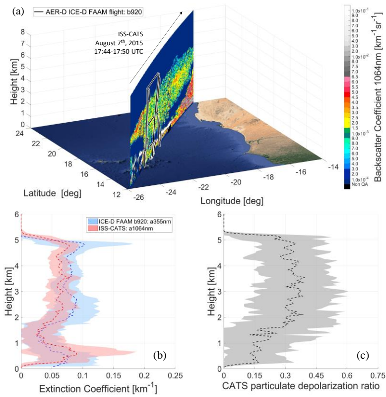
Figure 8: FAAM b920 – ISS-CATS underflight on the 7 th of August 2015 in the proximity of Praia-Cabo Verde (a), FAAM b920 lidar and ISS-CATS mean extinction coefficient profiles at 355nm and 1064nm respectively (b), and ISS-CATS mean particulate depolarization ratio profile at 1064nm (c). In panel (a) the aircraft track is shown in black.
