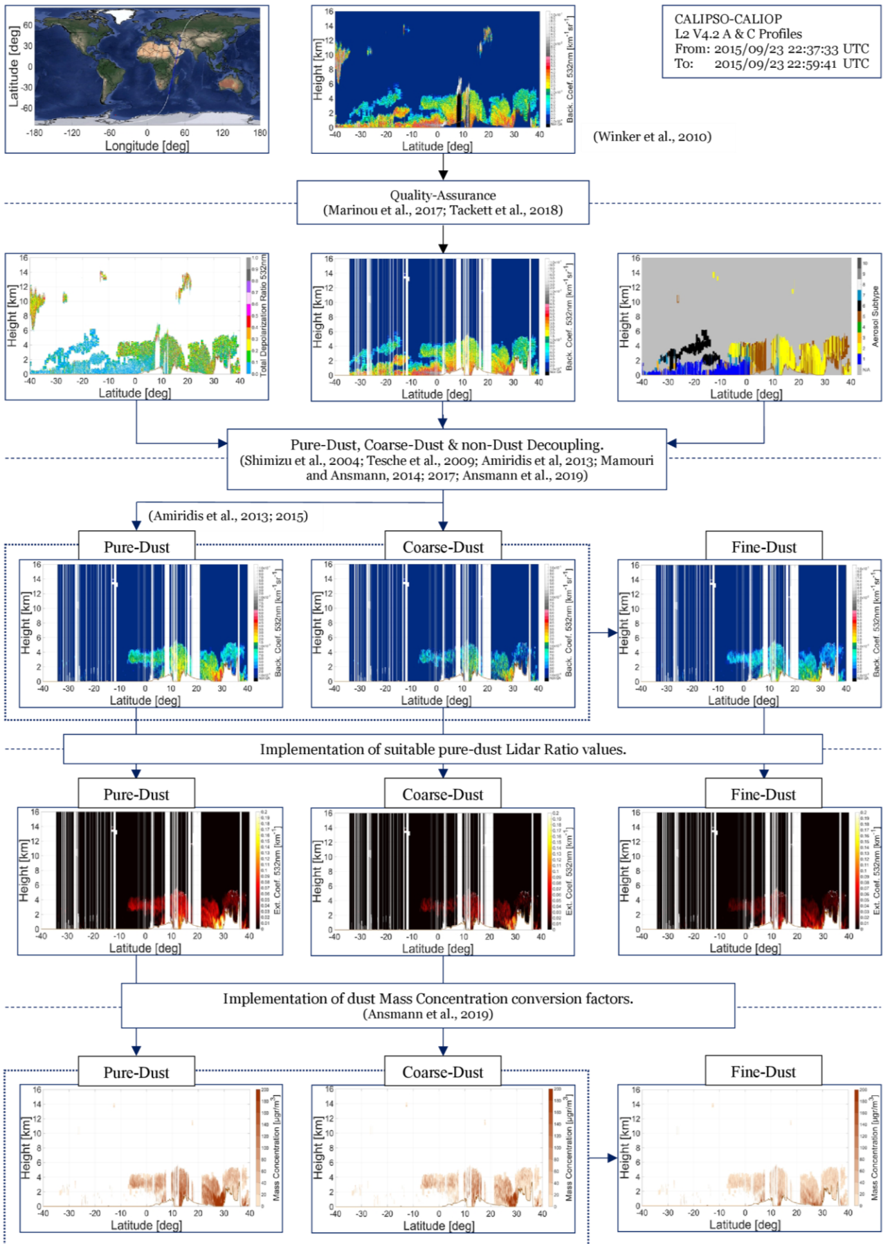
Figure 4: Illustration of the methodology, from quality assurance – to backscatter coefficient at 532 nm – to – extinction coefficient at 532 nm – to mass concentration separation and conversion steps of the fine-mode and coarse-mode components of atmospheric pure-dust, components of the total aerosol load, for an indicative CALIPSO-Middle East overpass case on the 23 rd of September, 2015.
