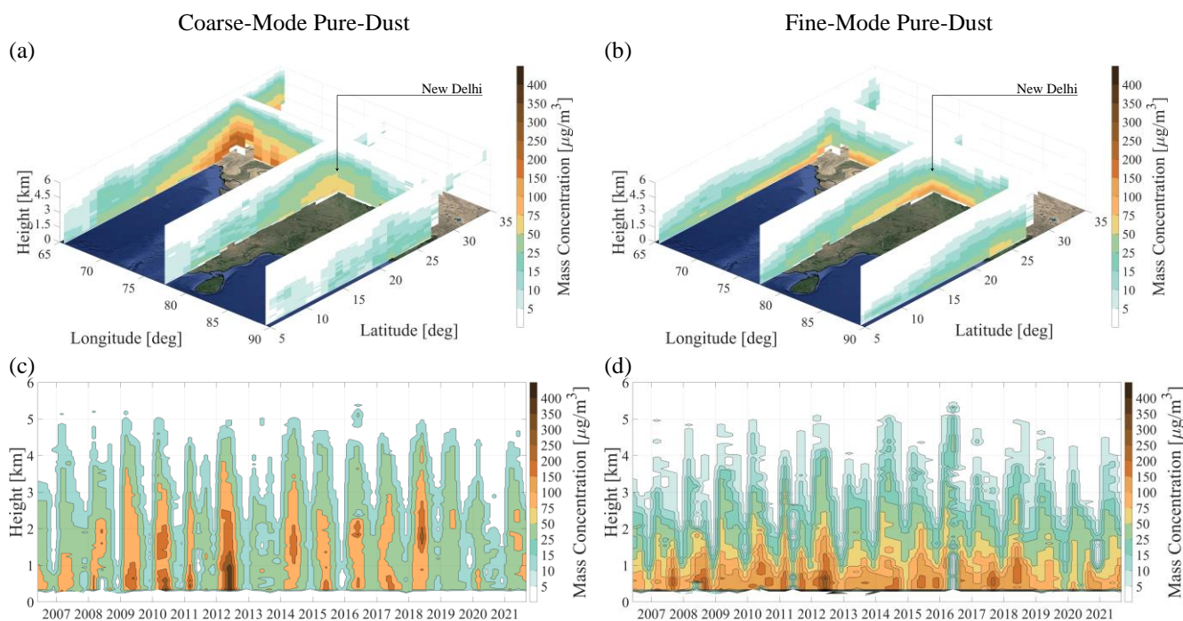
Figure 12: Coarse-mode (a) and fine-mode (b) pure-dust annual-mean mass concentration cross sections over the Indian peninsula (Lat: 28.5^{\circ}\text{N} - Lon: 76.5^{\circ}\text{E} - 06/2006-12/2021), and seasonal-mean mass concentration time-series over the New Delhi megacity area (Lat: 27^{\circ} - 29^{\circ}\text{N} - Lon: 76^{\circ} - 78^{\circ}\text{E} ) for the coarse-mode (c) and fine-mode (d) for New Delhi.
