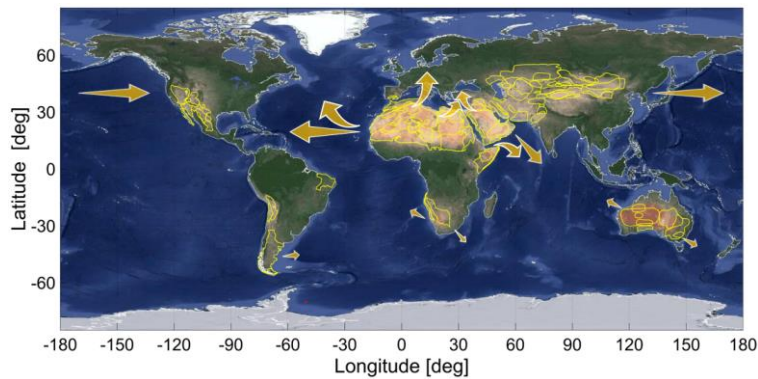
Figure 01: Hyper-arid, arid and semi-arid regions of easily erodible dry soils or areas of little vegetation (areas in yellow colour) and main aeolian dust transport pathways (source: Natural Earth Data: https://www.naturalearthdata.com/ ; last access: 03/07/2023).
