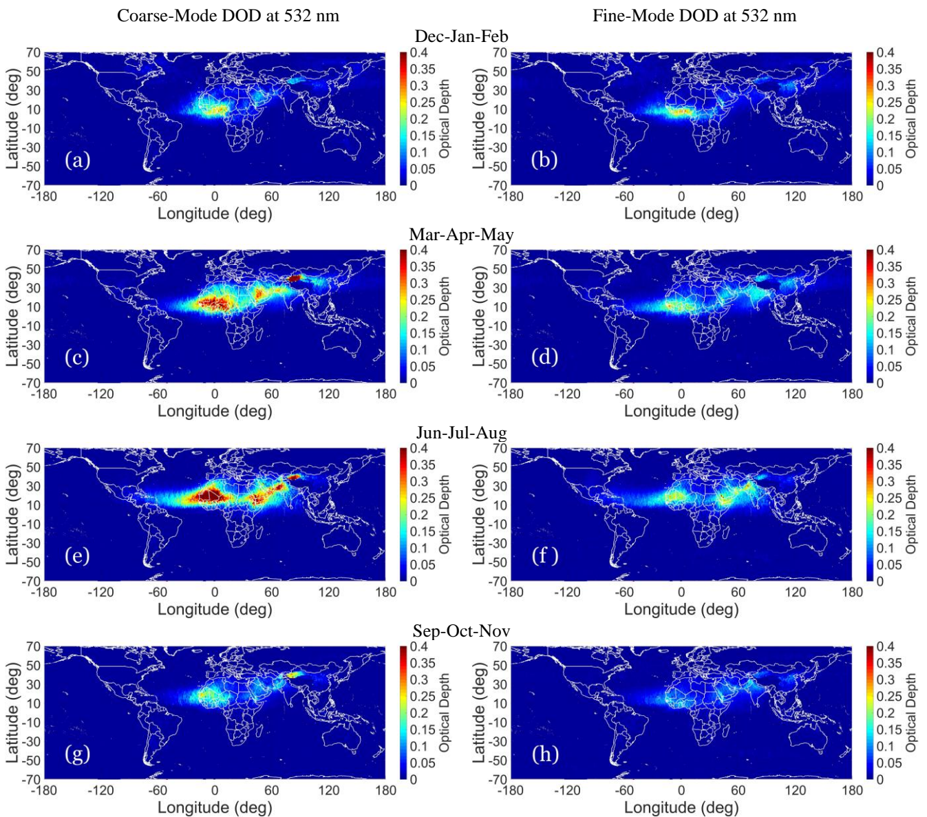
Figure 11: Seasonal coarse-mode (left column) and fine-mode (right column) components of DOD at 532 nm, grouped for “December-January-February (DJF)” (Fig.11a/b), “March-April-May (MAM)” (Fig.11c/d), “June-July-August (JJA)” (Fig.11e/f), and “September-October-November (SON)” (Fig.11g/h).
