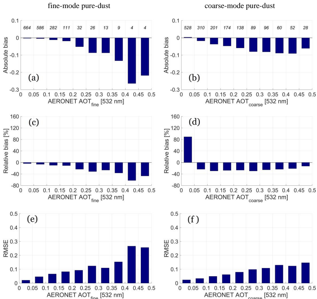
Figure 7: CALIPSO-based fine-mode (left column) and coarse-mode (right column) DOD at 532 nm absolute biases (Fig.7a/b), relative biases (Fig.7c/d), and Root Mean Square Errors - RMSE (Fig.7e/f) by AERONET fine-mode and coarse-mode AOT at 532 nm class of equal increment step of 0.05 for the AOT at 532 nm range extending between 0 and 0.5.
