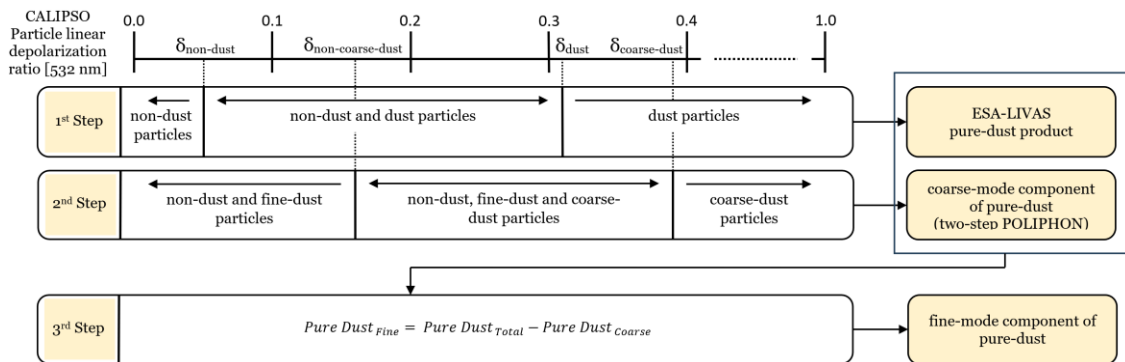
Figure 2: Illustration of the conceptual approach applied towards the derivation of the CALIPSO-based fine-mode and coarse-mode components of the total aerosol load at a near-global scale. Step 1 includes implementation of the CALIPSO-based ESA-LIVAS pure-dust global product. Step 2 provides the coarse-mode pure-dust atmospheric component through implementation of the first step of the two-step POLIPHON method. Step 3 provides the fine-mode pure-dust component as the residual between the ESA-LIVAS pure-dust product and the coarse-mode component of pure-dust. Moreover, the figure reports on " \delta_d ", " \delta_{nd} ", " \delta_{cd} ", and " \delta_{ncd} " depolarization at 532 nm threshold values considered here, equal to 0.31, 0.05, 0.39, and 0.16 respectively.
