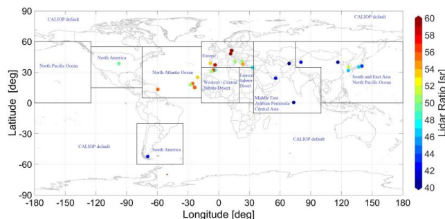
15 Figure 3: Illustration of the regional classification of pure-dust LR values applied in the present study.
