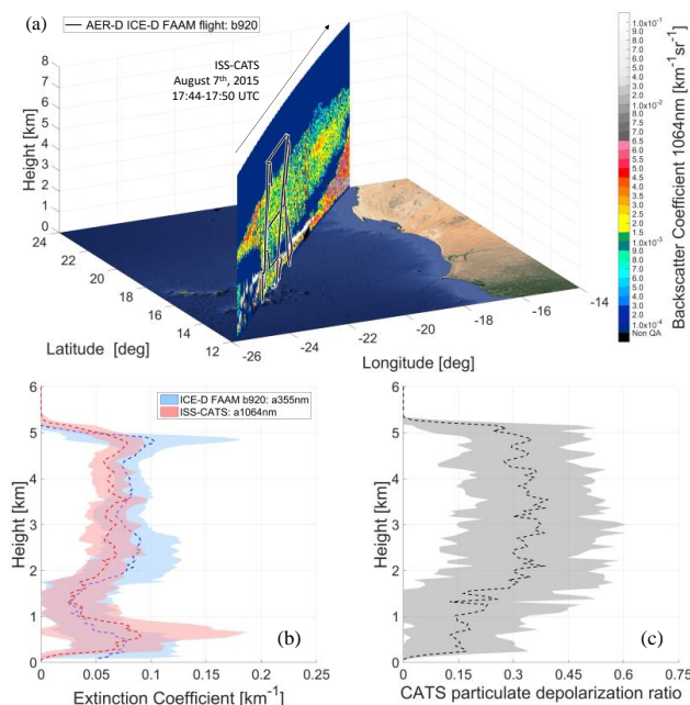
Figure 8: FAAM b920 – ISS-CATS underflight on the 7 th of August 2015 in the proximity of Praia-Cabo Verde (a), FAAM b920 lidar and ISS-CATS mean extinction coefficient profiles at 355nm and 1064nm respectively (b), and ISS-CATS mean particulate depolarization ratio profile at 1064nm (c). In panel (a) the aircraft track is shown in black.
