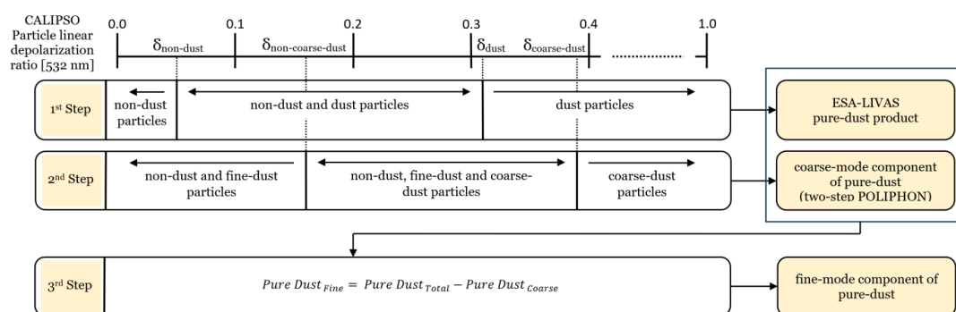
Figure 2: Illustration of the conceptual approach applied towards the derivation of the CALIPSO-based fine-mode and coarse-mode components of the total aerosol load at a near-global scale. Step 1 includes implementation of the CALIPSO-based ESA-LIVAS pure-dust global product. Step 2 provides the coarse-mode pure-dust atmospheric component through implementation of the first step of the two-step POLIPHON method. Step 3 provides the fine-mode pure-dust component as the residual between the ESA-LIVAS pure-dust product and the coarse-mode component of pure-dust. Moreover, the figure reports on " \delta_d ", " \delta_{nd} ", " \delta_{cd} ", and " \delta_{ncd} " depolarization at 532 nm threshold values considered here, equal to 0.31, 0.05, 0.39, and 0.16 respectively.
