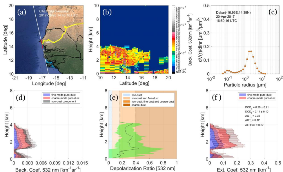
Figure 5: Major Saharan dust outbreak moving westwards over Dakar on the 20 th of April, 2017 at ~14:43 UTC, including the CALIPSO overpass in the proximity of the AERONET-Dakar station (red line) and FLEXPART 6-day back-trajectories at 2 km at the area of interest (Lat: 14.39, Lon: -16.95) denoting the Saharan desert origin of the advected air masses (yellow line) (Fig.5a). CALIPSO L2 5 km backscatter coefficient at 532 nm cross section (Fig.5b). Column-integrated particle volume concentration as a function of particle radius observed with the AERONET sunphotometer over Dakar, Senegal (Fig.5c). Backscatter coefficient at 532 nm profiles of the coarse-mode pure-dust (red shaded area), fine-mode pure-dust (blue shaded area), and non-dust (gray shaded area) components of the total aerosol load (Fig.5d). Particulate depolarization ratio at 532 nm profile used for the decoupling of the coarse-mode pure-dust, fine-mode pure-dust, and non-dust components of the total aerosol load, as provided in Fig.5d (Fig.5e). Extinction coefficient at 532 nm profiles of the coarse-mode pure-dust (red shaded area) and fine-mode pure-dust (blue shaded area) components of the total aerosol load (Fig.5f).
