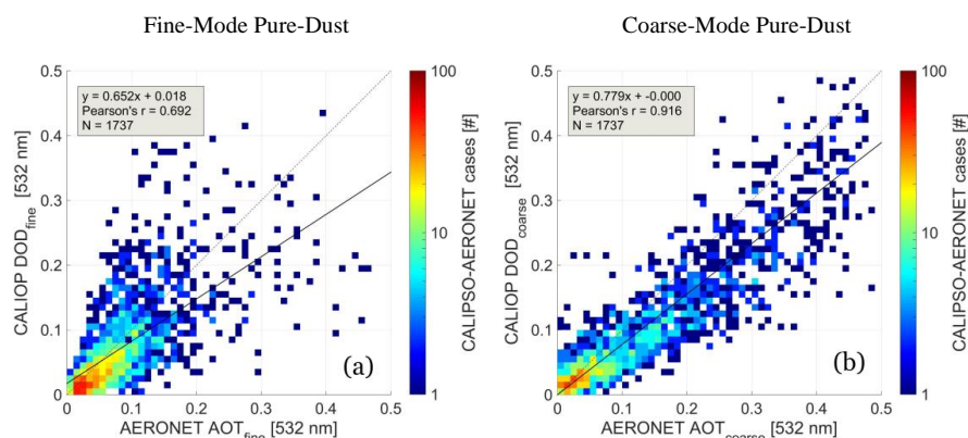
Figure 6: Evaluation of the CALIPSO-based DOD_{fine} and DOD_{coarse} at 532 nm products against AERONET AOT_{fine} and AOT_{coarse} at 532 nm retrievals respectively, in the form of 2D histogram density scatterplots.
