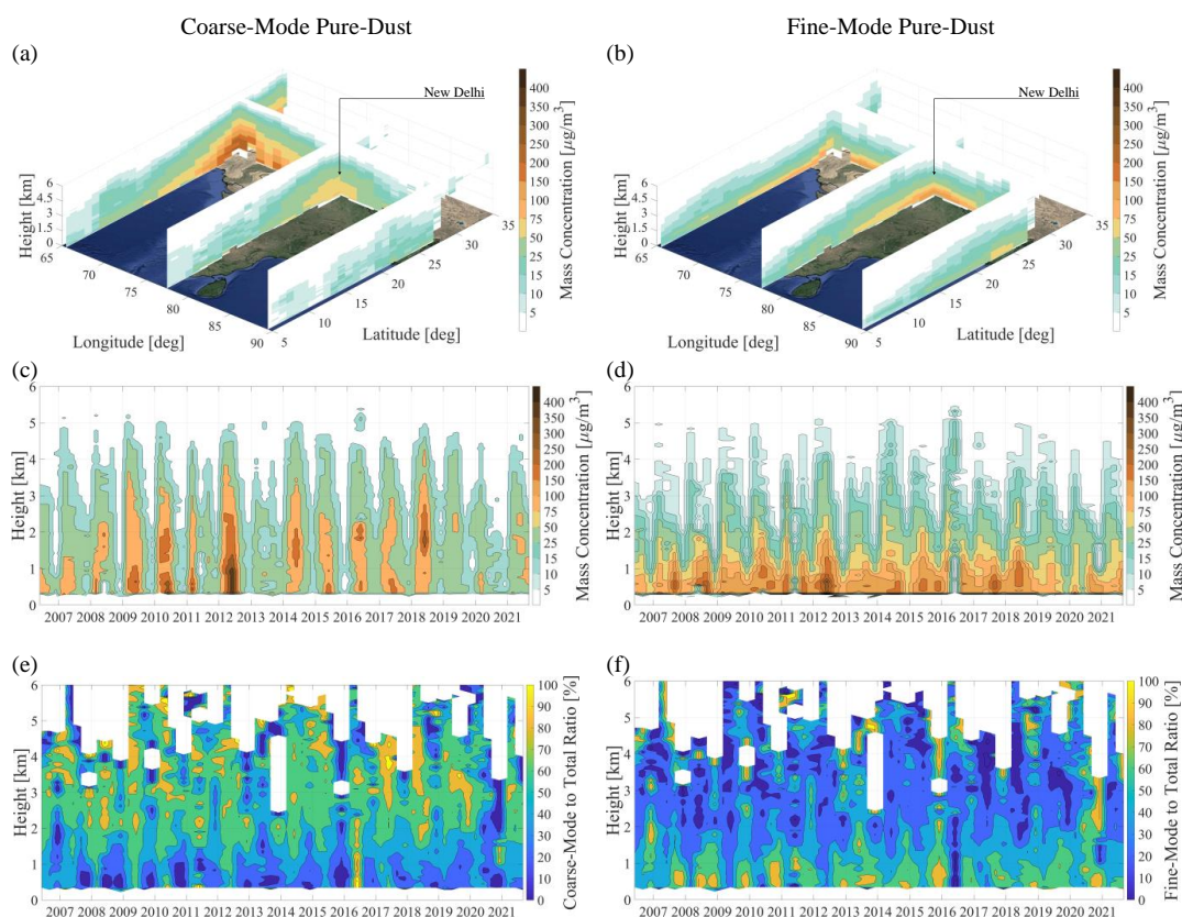
Figure 12: Coarse-mode (a) and fine-mode (b) pure-dust annual-mean mass concentration cross sections over the Indian peninsula (Lat: 28.5^{\circ}\text{N} - Lon: 76.5^{\circ}\text{E} - 06/2006-12/2021), seasonal-mean mass concentration time-series over the New Delhi megacity area (Lat: 27^{\circ} - 29^{\circ}\text{N} - Lon: 76^{\circ} - 78^{\circ}\text{E} ) for the coarse-mode (c) and fine-mode (d), and coarse-mode pure-dust to total pure-dust ratio (e) and the fine-mode pure-dust to total pure-dust ratio (f) for New Delhi.
