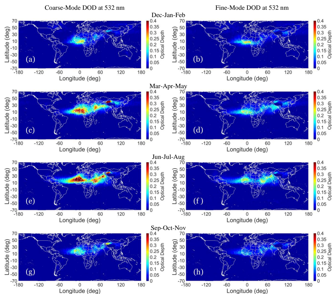
5 Figure 11: Seasonal coarse-mode (left column) and fine-mode (right column) components of DOD at 532 nm, grouped for “December-January-February (DJF)” (Fig.11a/b), “March-April-May (MAM)” (Fig.11c/d), “June-July-August (JJA)” (Fig.11e/f), and “September-October-November (SON)” (Fig.11g/h).
