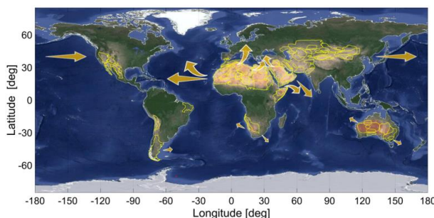
10 Figure 01: Hyper-arid, arid and semi-arid regions of easily erodible dry soils or areas of little vegetation (areas in yellow colour) and main aeolian dust transport pathways (source: Natural Earth Data: https://www.naturalearthdata.com/ ; last access: 03/07/2023).
