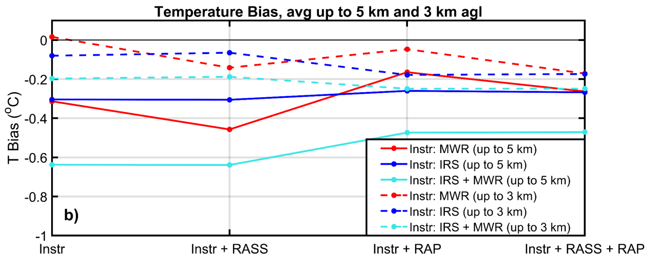
Fig. 7. Panel a: Mean absolute error of the retrieved temperature profiles averaged over the lower 3 (dashed lines) and 5 (solid lines) km agl for each of the 12 TROPoe configurations. Panel b: Same as for panel a, but for bias (TROPoe minus radiosonde temperature).
