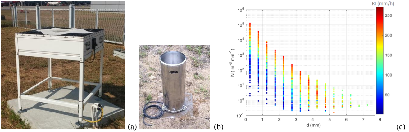
125 Figure 2: (a) The 2DVD instrument installed at the HKO field test site, (b) the SMIF tipping-bucket rain gauge and (c) DSD measurements colour coded (see the lateral colour bar) according to the rainfall intensity (RI) as measured by the 2DVD. N is the number of particles in a cubic meter of air per bin size while d is the drop diameter.
