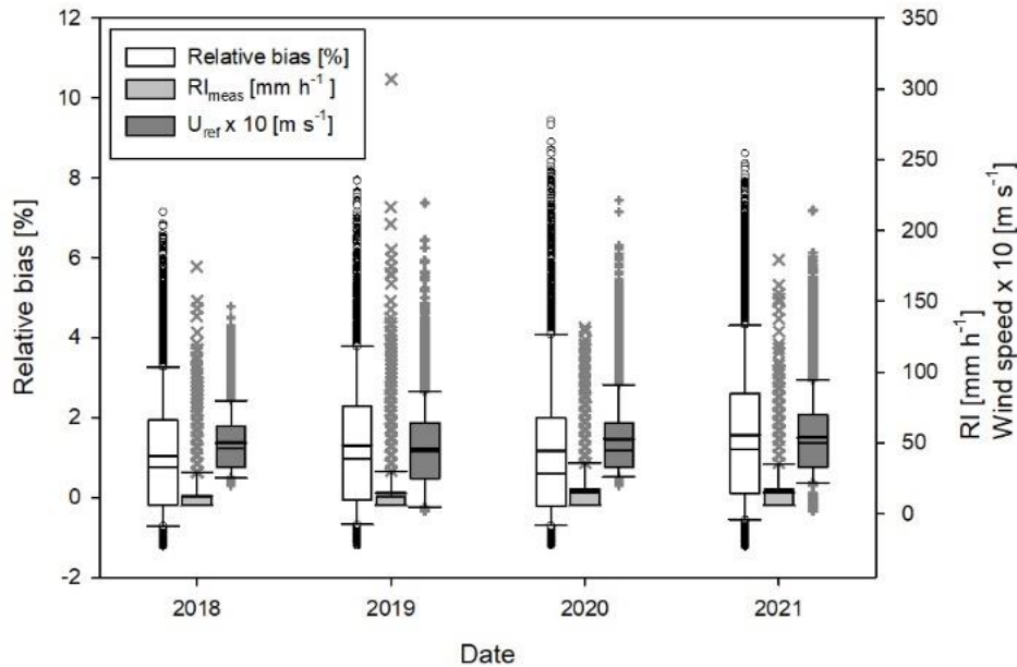
235 Figure 8: Non-parametric distribution of the one-minute percentage relative bias [%] (left-hand axis), measured rainfall intensity ( RI_{\text{meas}} ) and wind speed ( U_{\text{ref}} ) (right-hand axis) for the four investigated years individually. Boxes and whiskers encompass the central 50% and 80% of the dataset, respectively, while markers indicate values out of the 5 th and 95 th percentiles of their non-parametric distribution. The mean and median values are depicted with the thick and thin horizontal lines, respectively.
