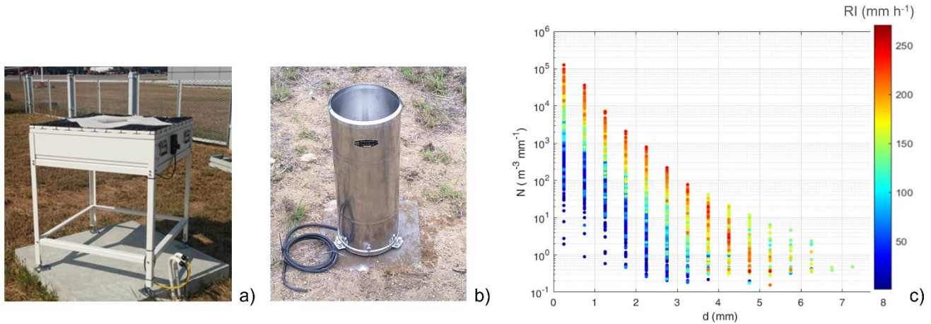
Figure 2: (a) The 2DVD instrument installed at the HKO field test site, (b) the SMIF tipping-bucket rain gauge and (c) DSD measurements colour coded (see the lateral colour bar) according to the rainfall intensity (RI) as measured by the 2DVD. N is the number of particles in a cubic meter of air per bin size while d is the drop diameter.
