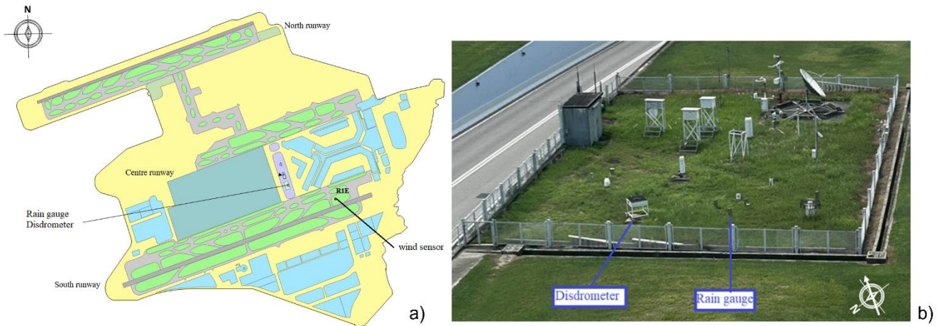
Figure 1: (a) Location of the field test site within the Hong Kong International Airport, (R1E indicates the wind sensor) and (b) picture of the installed rain gauge and 2DVD within the field test site, the white arrow indicates the prevailing wind direction (about 100 degrees).
