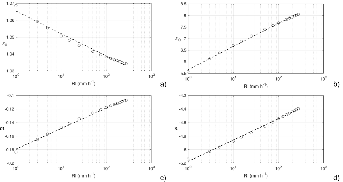
Figure 6: Logarithmic best-fit functional dependency of the sigmoidal Collection Efficiency (CE) coefficients ( \varepsilon_0 , x_0 , m and n ) – see Eq. 6 – on the rainfall intensity (RI).
