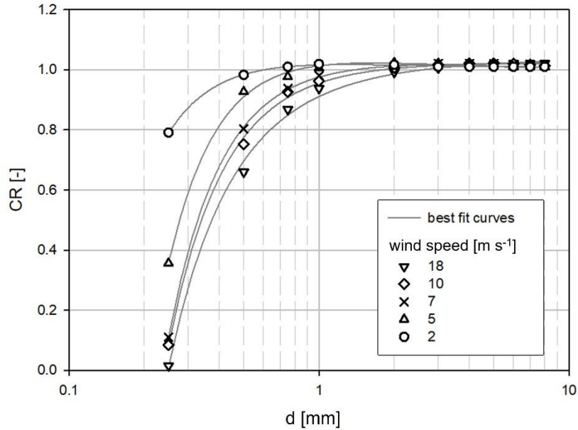
155 Figure 4: Semi-logarithmic plot of the catch ratios (CR) obtained from CFD simulation by Cauteruccio and Lanza (2020) (indicated with markers) for a cylindrical gauge and best-fit inverse polynomials for selected wind speed values (continuous lines) as a function of diameter (d).
