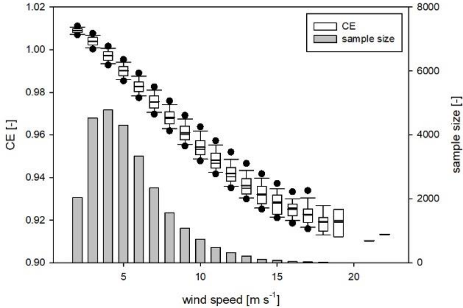
Figure 7: One-minute Collection Efficiency (CE) values (left-hand axis) for wind speed classes with a bin width equal to 1 m s -1 . Boxes and whiskers encompass the central 50% and 80% of the dataset, respectively, while dots indicate the 5 th and 95 th percentiles of their non-parametric distribution. The mean and median values are depicted with the thick and thin horizontal lines, respectively. Wind speed classes are used with a bin width equal to 1 m s -1 . Grey bars indicate the sample size for each wind speed class (values on the right-hand axis).
