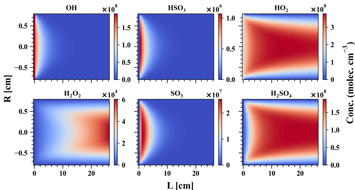
Figure 2. MARFORCE simulation results of a \text{H}_2\text{SO}_4 calibration experiment. The x-axis shows the distance from the UVP pen-ray lamp to the entrance of the chemical ionisation chamber and the y-axis shows the distance in the radial direction. Conditions for the simulation: R = 0.78 cm, L = 26 cm, sample flow = 10.6 slpm, [\text{SO}_2] = 5.78 \times 10^{13} \text{ cm}^{-3} , [\text{O}_2] = 2.42 \times 10^{16} \text{ cm}^{-3} and [\text{H}_2\text{O}] = 2.8 \times 10^{16} \text{ cm}^{-3} .
