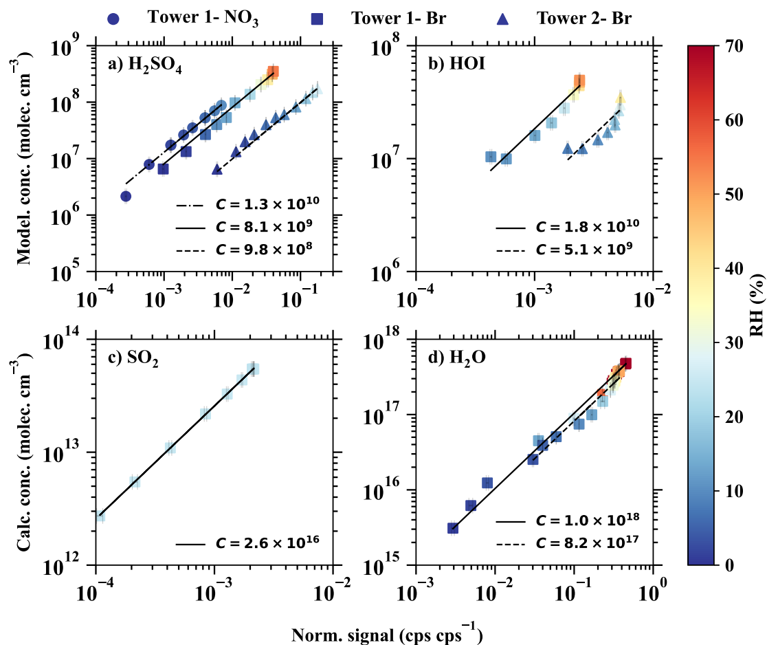
Figure 3. The modelled or calculated vapour concentrations vs. the normalised signals for a) \text{H}_2\text{SO}_4 , b) \text{HOI} , c) \text{SO}_2 , d) \text{H}_2\text{O} . The dashed-dotted, solid, and dashed lines are the linear fits of the results from different inlet modes: 1) tower 1 with the \text{NO}_3^- chemical ionisation method, 2) tower 1 with the \text{Br}^- chemical ionisation method, and tower 2 with the \text{Br}^- chemical ionisation method. The slopes of the fitted lines represent the calibration coefficients, shown in the legend. The colour bar shows the relative humidity in the calibration experiments.
