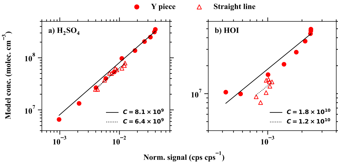
Figure A6. Comparing calibration experiments of a) H 2 SO 4 and HOI with a straight tube (Figure A2) or additionally with a dilution flow (Figure A3). The difference in the calibration coefficients between the two experimental setups is the result of the less accurate representation of fluid dynamics when the dilution flow is added (Figure A3).
