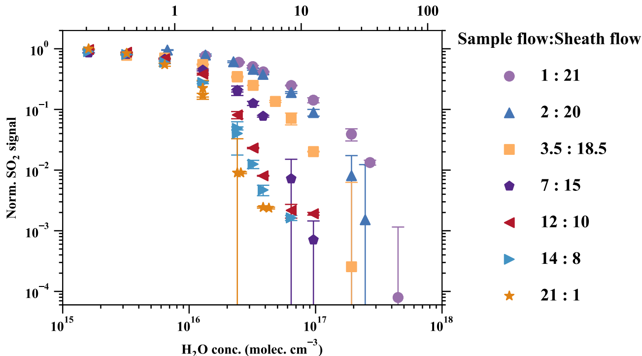
Figure 5. Reducing the detection humidity effect with the core sampling method (Figure A9). This design takes the advantage of the faster diffusion of \text{H}_2\text{O} than \text{SO}_2 from the sample flow to the sheath flow and effectively reduces the RH in the sample flow. Various sample-to-sheath ratios were tested at different \text{H}_2\text{O} concentrations to find the optimal setting. All the data are normalised to the lowest RH data point in the sample-to-sheath = 21:1 experiment. Due to experimental constraints, the sample-to-sheath ratios = a) 3.5:18.5, b) 2:20 and c) 1:21 experiments started only from the second, third and fourth lowest RH points, respectively. All other experiments collected data in all humidity conditions. The error bars represent the standard deviation of the normalised \text{SO}_2 signals.
