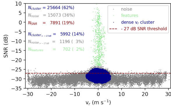
Figure 3. Scatter of v_r against SNR, with a DBSCAN identified cluster of dense scatterers (valid v_r ) marked in blue and rarefied scatterers (noise) marked in grey, and rarefied scatterers corresponding to features marked in mint. The number of points (and the percentage relative to the whole data) which is classified as noise, N_{noise} (grey), features, N_{features} (mint) and as cluster of reasonable points, N_{cluster} (blue) are documented in the upper left corner. The dashed red line indicates the -27 dB SNR threshold. Values of v_r corresponding to SNR values below this line are discarded by the SNR filter. N_{SNR} (red) corresponds to the number of points (and percentage relative to the whole data) recovered by the SNR filter, while N_{SNR} \cdot N_{cluster > -27dB} (grey/blue) and N_{SNR} \cdot N_{noise > -27dB} (blue/grey) correspond to the number of points-scatterers (and percentage relative to the whole data) recovered by the SNR filter, yet attributed to the points corresponding to noise and reasonable values by the DBSCAN filter, respectively
