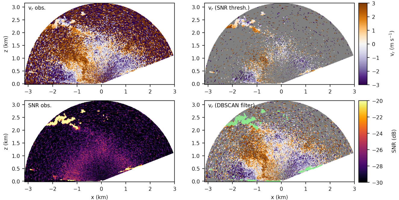
Figure 4. Sample RHI scan from the Stormoen campaign 29 July 2022 at 14:20 UTC with (a) observed v_r , (b) observed SNR, (c) filtered v_r using an SNR threshold, and (d) filtered v_r using the DBSCAN clustering algorithm. Grey areas correspond to filtered values, flagged as NaN by the (c) SNR threshold filter or (d) DBSCAN filter, respectively. Features, also flagged as NaN by the DBSCAN filter are highlighted in mint.
