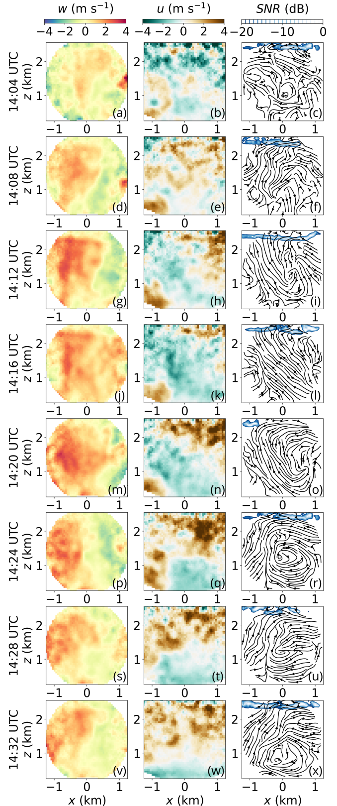
Figure 10. Temporal evolution of convection on 29 July 2022 at Starmoen Airport. 1. column: retrieved w field, 2. column: retrieved u field, 3. column: streamlines and SNR (cloud back-scatter)
