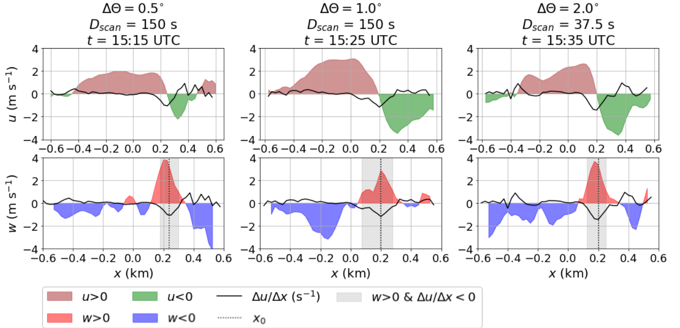
Figure 8. Averaged, near surface ( \leq 150 m) horizontal divergence, 1. row: u and 2. row: w estimates to visualize the identification process for the near-surface updraft location, x_0 . The three columns correspond to the three different scan configurations with configuration specific \Delta\theta , D_{scan} and t (instantaneous cross-section).
