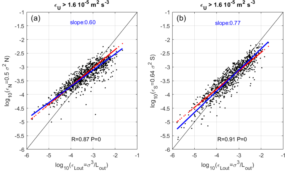
Figure 6: Scatter plots of (a) \log_{10}(\epsilon_{L_{out}}) vs \log_{10}(\epsilon_N) and (b) \log_{10}(\epsilon_{L_{out}}) vs \log_{10}(\epsilon_S) for \epsilon_U > 1.6 \cdot 10^{-5} \text{ m}^2 \text{ s}^{-3} . The red lines show the results for N = \text{cst} (a) and S = \text{cst} (b). The blue lines show the results of a linear regression (whose slope value is indicated in the insert).
