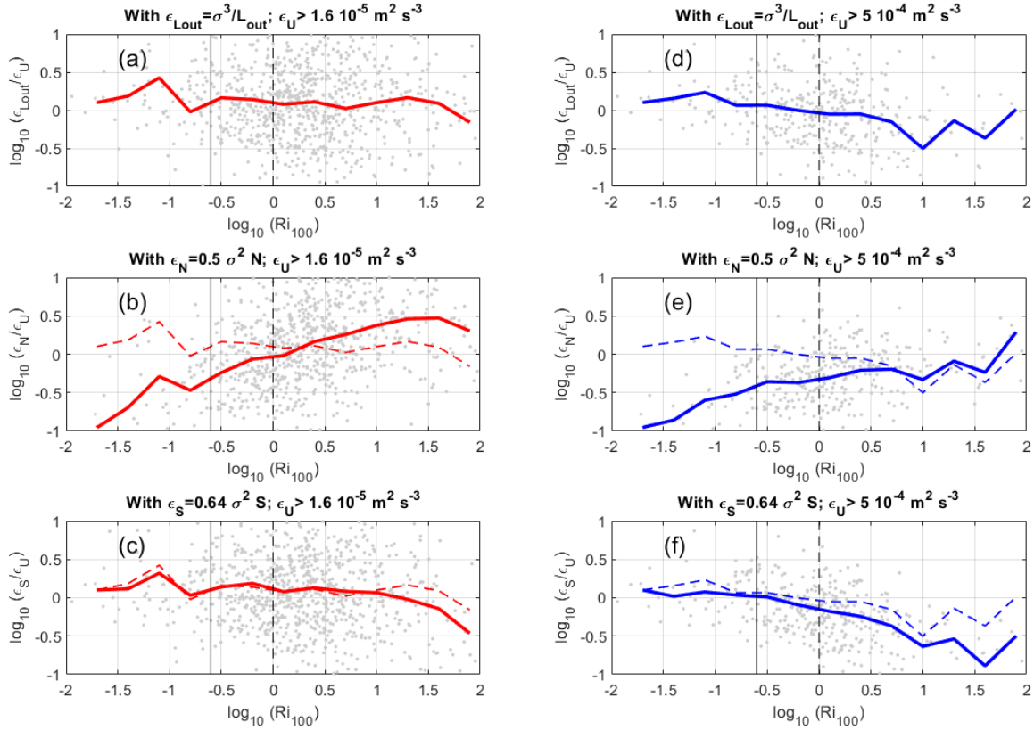
Figure 9: Scatter plots of \log_{10}(\text{Ri}_{100}) vs (a), (d) \log_{10}(\epsilon_{\text{Lout}}/\epsilon_U) , (b),(e) \log_{10}(\epsilon_N/\epsilon_U) , (c), (f) \log_{10}(\epsilon_S/\epsilon_U) for \epsilon_U > 1.6 \cdot 10^{-5} \text{ m}^2 \text{ s}^{-3} and \epsilon_U > 5.0 \cdot 10^{-4} \text{ m}^2 \text{ s}^{-3} , respectively.
