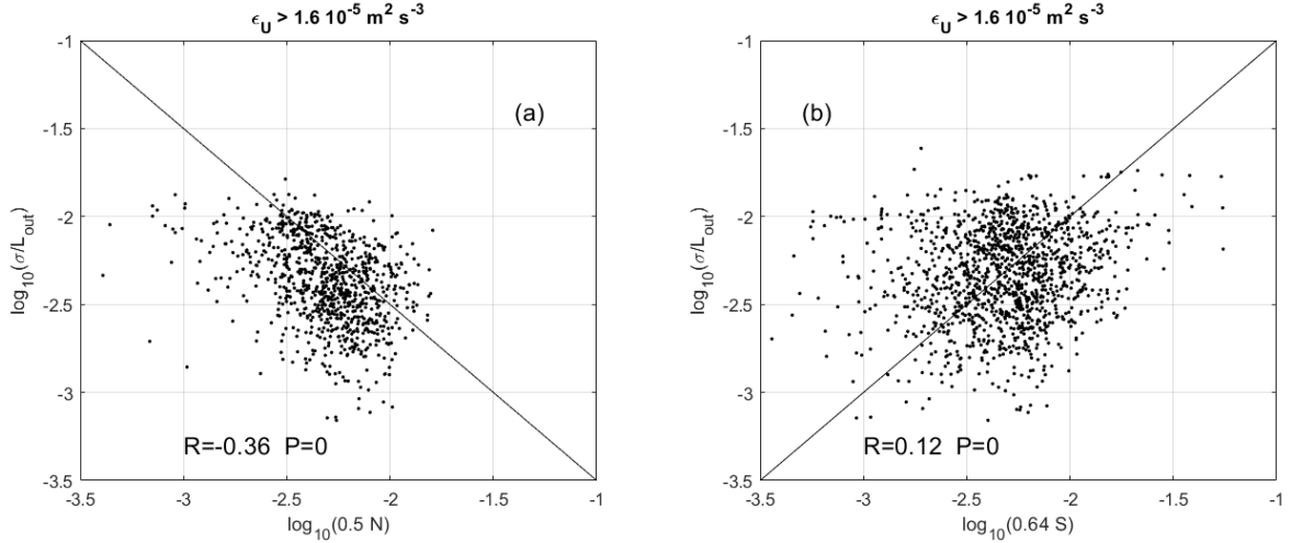
460 Figure 7: Scatter plots of (a) \log_{10}(0.5 N) vs \log_{10}(\sigma/L_{out}) and (b) \log_{10}(0.64 S) vs \log_{10}(\sigma/L_{out}) for \epsilon_U > 1.6 \cdot 10^{-5} \text{ m}^2 \text{ s}^{-3} . R is the correlation coefficient and P is the result of the P test.
