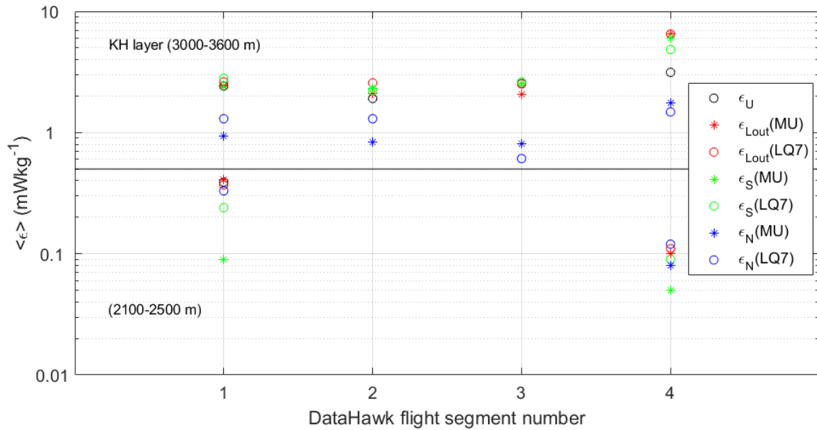
340 Figure 3: Graphical representation of the averaged estimates of TKE dissipation rates ( \text{mWkg}^{-1} ) ( 1 \text{ mWkg}^{-1} = 10^{-3} \text{ m}^2 \text{ s}^{-3} ) shown in Table 3 for the K-H layer (3000-3600 m) sampled 4 times (top) and the layer between 2100 m and 2500 m sampled twice during A1 (segment n° 1) and D2 (segment n°4) (bottom). The horizontal black line at 0.5 \text{ mWkg}^{-1} separates the two cases for clarity.
