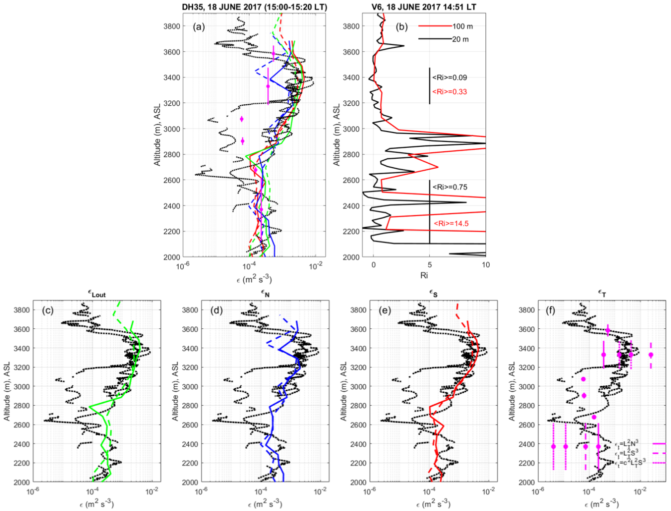
Figure 2: (a) DataHawk-derived \epsilon ( \text{m}^2 \text{s}^{-3} ) profiles in the height range [2000-3900] m during A1, D1, A2 and D2 of DH35 on 18 June 2017 (dotted black), \epsilon_S (LQ7) profile (solid red), \epsilon_{Lout} (LQ7) profile (solid green), \epsilon_N (LQ7) profile (solid blue), \epsilon_S (MU) profile (dashed red), \epsilon_{Lout} (MU) profile (dashed green), \epsilon_S (MU) profile (dashed blue) derived from radar data between 15:00 and 15:20 LT. Magenta dots and lines show \epsilon_T (Eq. 6) with c=1 , the depth and altitude of the Thorpe layers. (b) Richardson number profiles estimated from RS92-SGP Vaisala radiosonde V6 data at a vertical resolution of 20 m (black) and 100 m (red). (c,d,e,f) Same as (a) but with separate plots for each model ( \epsilon_{Lout} , \epsilon_N , \epsilon_S , \epsilon_T ), respectively. (f) shows the results in magenta for \epsilon_T (Eq. 6) with c=1 (solid line), \epsilon'_T (Eq. 7) with c' = 1 (dashed line) and \epsilon''_T (Eq. 7) with c' = 0.41 and c' = 0.24 (dotted line).
