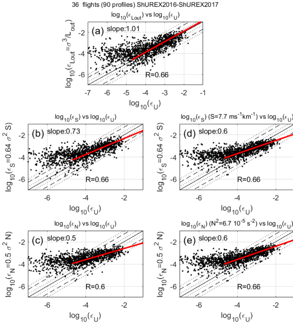
415 Figure 5: Scatter plots of \log_{10}(\epsilon_U) vs (a) \log_{10}(\epsilon_{\text{Lout}}) , (b) \log_{10}(\epsilon_S) , (c) \log_{10}(\epsilon_N) , (d) \log_{10}(\epsilon_S) with S = \text{cst} , (e) \log_{10}(\epsilon_N) with N = \text{cst} . The red lines are the result of a line regression (whose slope value is indicated in the insert) for \epsilon_U > 1.6 \times 10^{-5} \text{ m}^2 \text{ s}^{-3} and R is the correlation coefficient.
