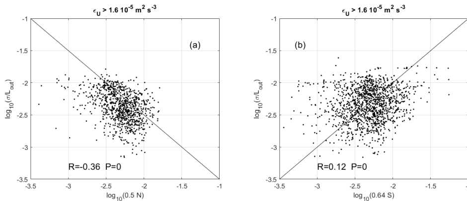
445 Figure 7: Scatter plots of (a) \log_{10}(0.5 N) vs \log_{10}(\sigma/L_{out}) and (b) \log_{10}(0.64 S) vs \log_{10}(\sigma/L_{out}) for \epsilon_U > 1.6 \cdot 10^{-5} \text{ m}^2 \text{ s}^{-3} . R is the correlation coefficient and P is the result of the P test.
