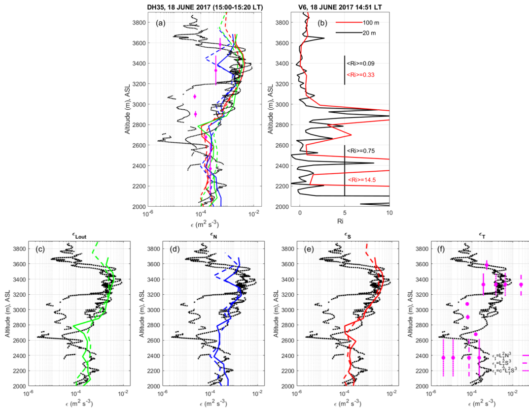
Figure 2: (a) DataHawk-derived \epsilon ( m^2 s^{-3} ) profiles in the height range [2000-3900] m during A1, D1, A2 and D2 of DH35 on 18 June 2017 (dotted black), \epsilon_S(LQ7) profile (solid red), \epsilon_{Lout}(LQ7) profile (solid green), \epsilon_N(LQ7) profile (solid blue), \epsilon_S(MU) profile (dashed red), \epsilon_{Lout}(MU) profile (dashed green), \epsilon_S(MU) profile (dashed blue) derived from radar data between 15:00 and 15:20 LT. Magenta dots and lines show \epsilon_T (Eq. 5) with c=1 , the depth and altitude of the Thorpe layers. (b) Richardson number profiles estimated from RS92-SGP Vaisala radiosonde V6 data at a vertical resolution of 20 m (black) and 100 m (red). (c,d,e,f) Same as (a) but with separate plots for each model ( \epsilon_{Lout} , \epsilon_N , \epsilon_S , \epsilon_T ), respectively. (f) shows the results in magenta for \epsilon_T (Eq. 5) with c=1 (solid line), \epsilon_T' (Eq. 6) with c' = 1 (dashed line) and \epsilon_T' (Eq. 6) with c' = 0.41 and c' = 0.24 (dotted line).
