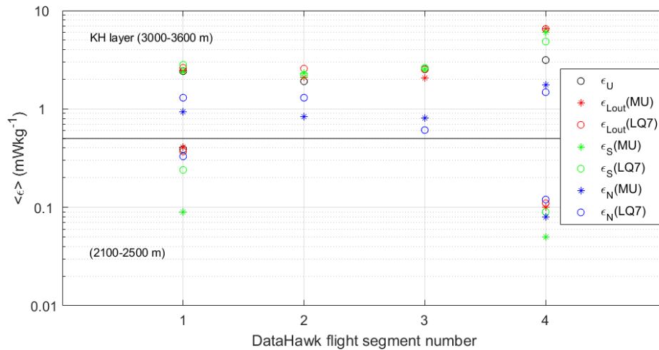
Figure 3: Graphical representation of the averaged estimates of TKE dissipation rates ( mWkg^{-1} ) ( 1 mWkg^{-1} = 10^{-3}m^2s^{-3} ) shown in Table 3 for the K-H layer (3000-3600 m) sampled 4 times (top) and the layer between 2100 and 2500 m sampled twice during A1 (segment n° 1) and D2 (segment n°4) (bottom). The horizontal black line at 0.5 325 mWkg^{-1} separates the two cases for clarity.
