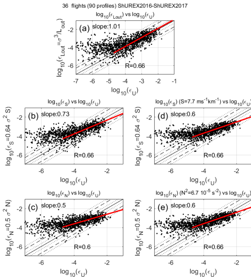
400 Figure 5: Scatter plots of \log_{10}(\epsilon_U) vs (a) \log_{10}(\epsilon_{Lout}) , (b) \log_{10}(\epsilon_S) , (c) \log_{10}(\epsilon_N) , (d) \log_{10}(\epsilon_S) with S = \text{cst} , (e) \log_{10}(\epsilon_N) with N = \text{cst} . The red lines are the result of a line regression (whose slope value is indicated in the insert) for \epsilon_U > 1.6 \cdot 10^{-5} \text{ m}^2 \text{ s}^{-3} and R is the correlation coefficient.
