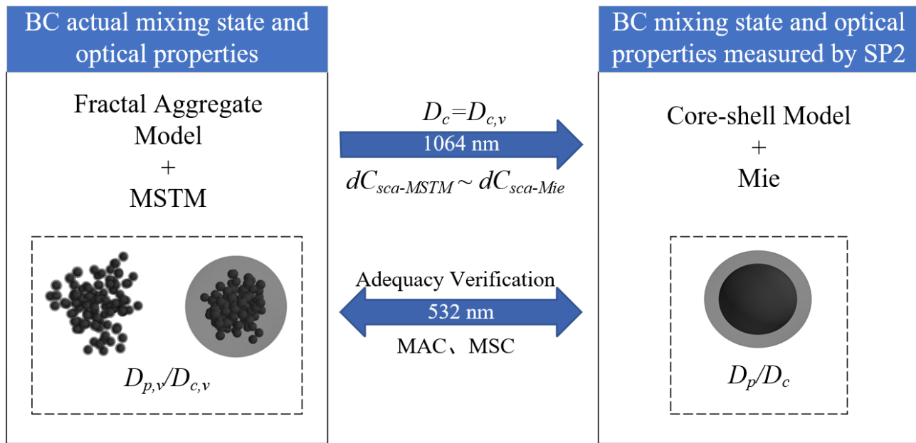
Figure 2. Schematic overview of the methodology of both the BC mixing state retrieval, and the verification of optical property at 532 nm predicted based on SP2 retrieval results.
