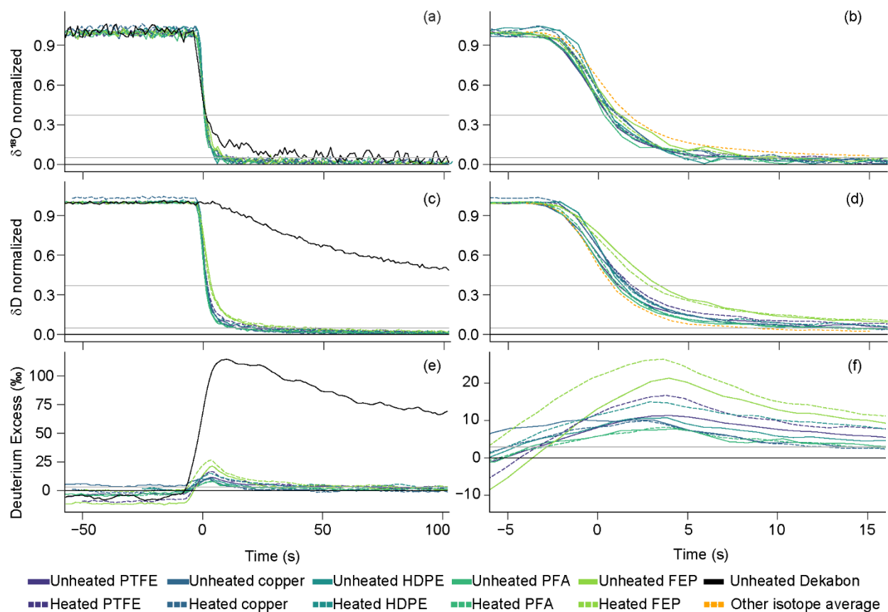
450 Figure 4. Mean attenuation curves for enriched-to-depleted (WVISS-to-DPG) H 2 O matched transitions of each tubing type for \delta^{18}\text{O} (a, b), \delta\text{D} (c, d), and D-excess (e, f) plotted as seconds since the \delta^{18}\text{O} impulse function peak (i.e. \delta^{18}\text{O} location adjusted time). The first column (panels a, c, and e) depicts time from 50 s before the peak of the \delta^{18}\text{O} impulse function for each experiment to 100 s after, while the second column (panels b, d, and f) zooms in on time from -5 to 15 s and excludes the Dekabon results. Solid lines indicate unheated experiments, while dashed lines indicate heated experiments. For \delta\text{D} , \delta^{18}\text{O} , and D-excess, only Dekabon and FEP show clear differences in material type, and only FEP shows clear differences in heated and unheated experiments. The full Dekabon attenuation curve can be found in Fig. S9. An orange curve in panel (b) shows mean \delta\text{D} of all experiments for comparison with \delta^{18}\text{O} and the orange curve in panel (d) shows mean \delta^{18}\text{O} for comparison with \delta\text{D} . These means exclude Dekabon. Here, 460 FEP is long thin-walled as a comparison to the rest of the thin-walled tubings. HDPE is thick-walled and has a smaller ID than the other tubing shown here. Gray horizontal lines indicate thresholds of 95 % and 63 % transition completion for \delta\text{D} and \delta^{18}\text{O} , and 3 % for D-excess, while a black line at zero indicates full equilibrium completion. Depleted-to-enriched results are presented in the supplemental materials.
