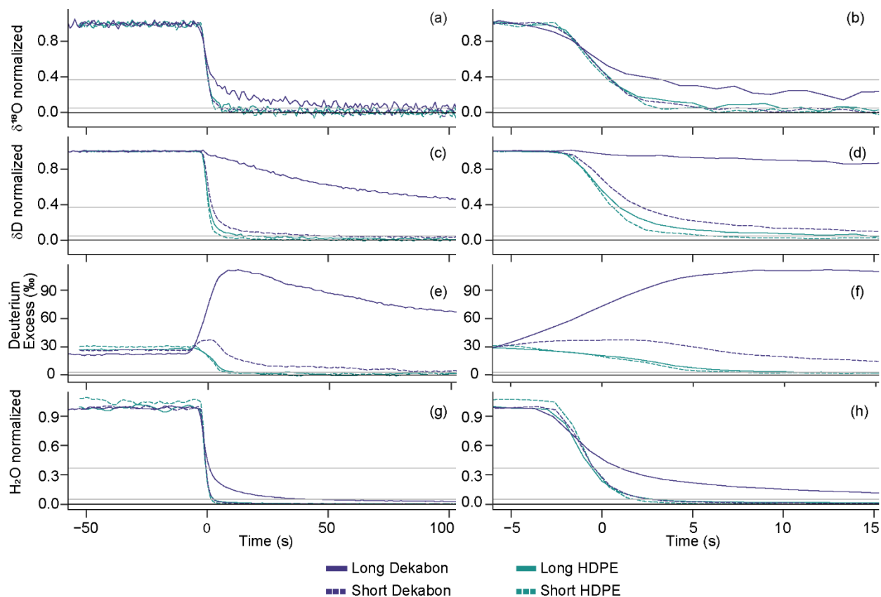
545 Figure 7. Mean attenuation curves comparing length for 2 m (~78.7 in.) and 100 ft (30.48 m) HDPE and Dekabon 550 tubing for enriched-to-depleted (WVISS-to-DPG) transitions for \delta^{18}\text{O} (a, b), \delta\text{D} (c, d), D-excess (e, f), and \text{H}_2\text{O} (g, h) plotted as seconds since the \delta^{18}\text{O} impulse function peak (i.e. \delta^{18}\text{O} location adjusted time). The first column (panels a, c, and e) depicts time from -50 to 100 s, while the second column (panels b, d, and f) zooms in on -5 to 15 s. Solid lines indicate 100 ft (30.48 m) lengths, while dashed lines indicate 2 m (~78.7 in.) lengths. Gray horizontal lines indicate thresholds of 95 % and 63 % transition completion for \delta\text{D} and \delta^{18}\text{O} , and 3 ‰ for D-excess, while the black line at zero indicates full equilibration.
