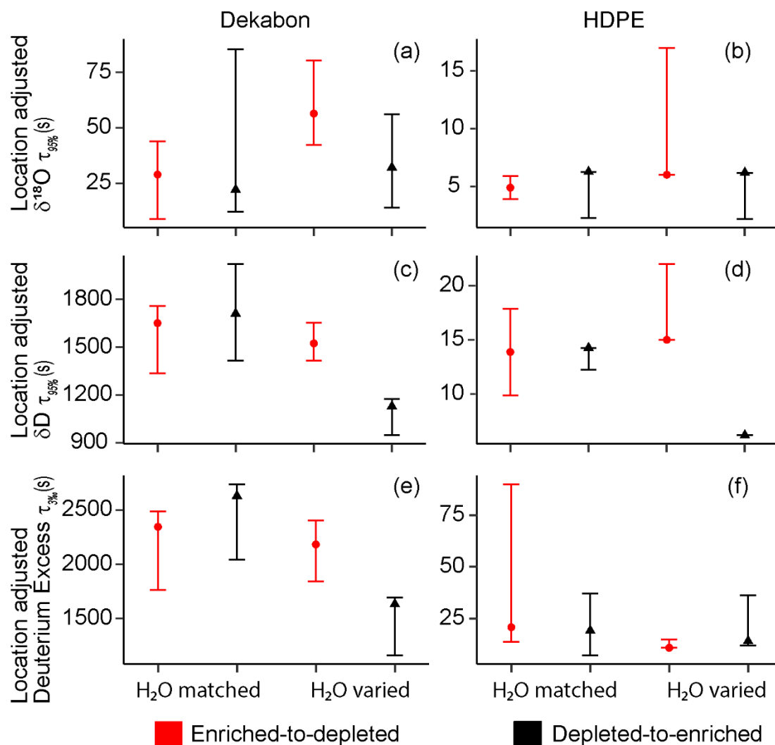
Figure 3. \delta^{18}\text{O} location adjusted t_{95\%} for \delta^{18}\text{O} and \delta\text{D} transitions and t_{3\%} times for D-excess in H 2 O matched and varied experiments of isotopic transition directions for long HDPE and Dekabon. The left panels (a, c, and e) depict Dekabon tests, and the right panels (b, d, and f) depict the HDPE tests. The depleted-to-enriched direction is indicated in black. The enriched-to-depleted direction is in red. Error bars indicate the maximum and minimum threshold times from the standard deviation of the experiment replicates. We saw differences in switch direction only in H 2 O varied experiments.
