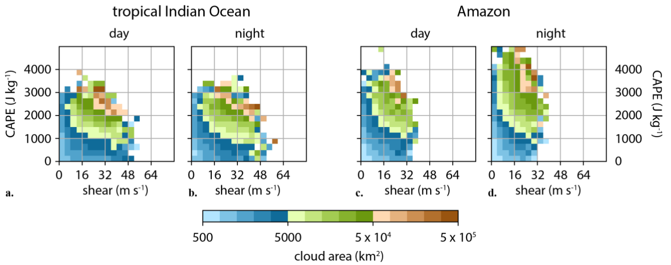
585 Figure 8: The average of cloud area in bins of maximum CAPE and vertical shear of the horizontal wind for all deep convective clouds observed over (a) and (b) the tropical Indian Ocean (10° S – 15° N, 50° E – 100° E; number of clouds N = 910,549), and (c) and (d) the Amazon (10° S – equator, 50° W – 65° W; number of clouds N = 205,757). For both locations data include deep convective clouds observed from all overpasses of the Aqua satellite during the months Nov.-Mar. from the eight years 2004-2011.
