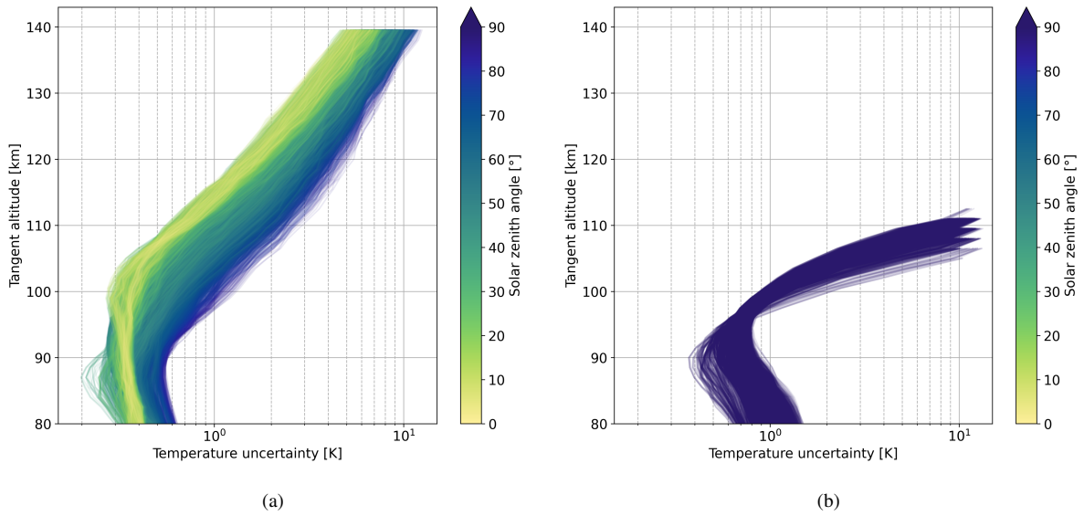
Figure 6. Temperature precision calculated from the expected signal from and input temperature presented in Figure 2e and the temperatures from 2a-2 and using an interpolated temperature precision field presented in Figure 5b assuming a binning of 20 rows; (a) and (b) depict the day- and night-time conditions, respectively ; note that signal counts below 100 counts are not considered which cuts off the night-time simulations around 110km
