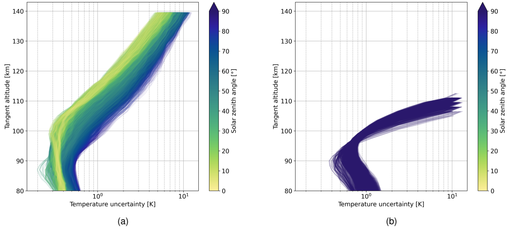
Figure 6. Temperature precision calculated from the expected signal and input temperature presented in Figure 2 and using an interpolated temperature precision field presented in Figure 5b assuming a binning of 20 rows; (a) and (b) depict the day- and night-time conditions, respectively; note that signal counts below 100 counts are not considered which cuts off the night-time simulations around 110km
