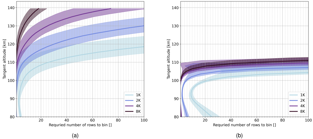
Figure 7. Required binning of rows to achieve a certain temperature precision (a) during day-time and (b) during night-time; the solid line shows the mean and the shaded area the standard deviation of all used samples from Figure 2c and 2f
