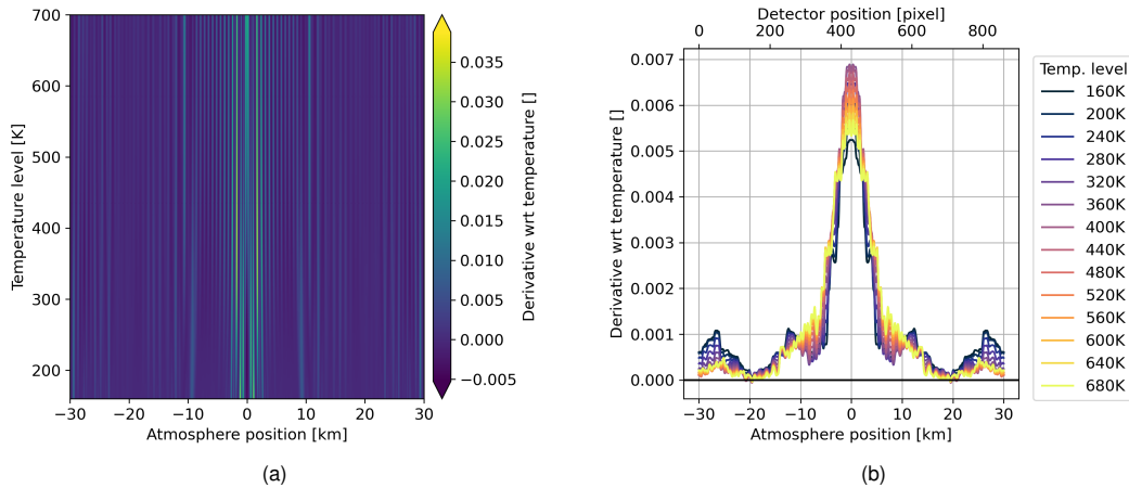
Figure 11. (a) Derivative of temperature at a given horizontal position for multiple temperature levels; (b) Selected rows of (a) and smoothed by a running mean with window size 101
