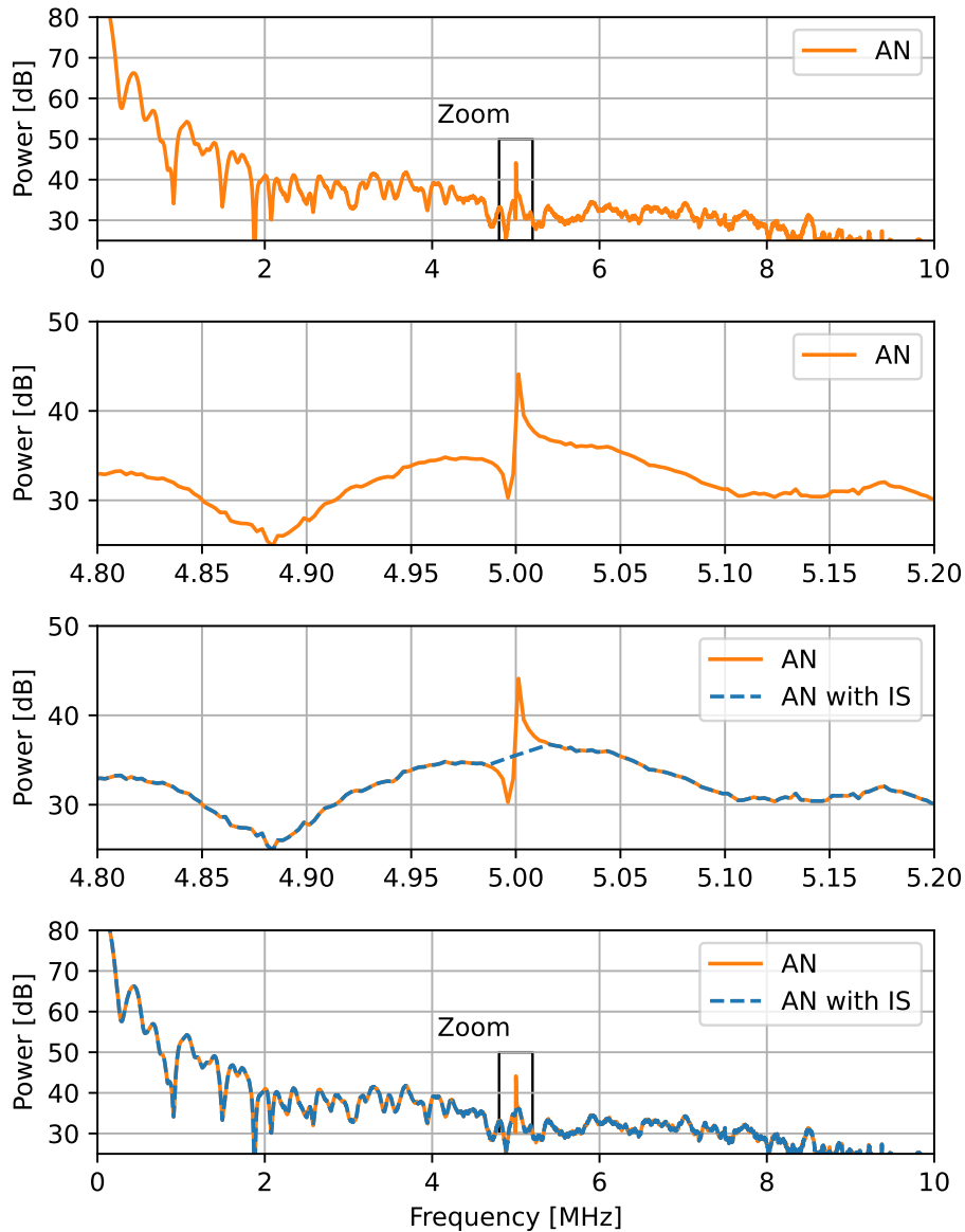
Figure 3. Illustration of the interference suppression (IS) applied to the 532nm AN channel: i) Spectrum with weak interference peak at 5MHz, ii) weak interference peak, iii) with linear interpolation between two samples as an IS method, and iv) the spectrum with IS
