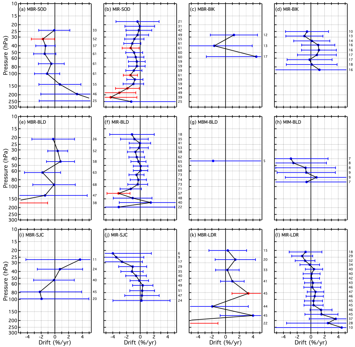
Figure B4. Same as Figure B1 for 12 additional SAT-FP pairings that include MBR, MIR, MBM, and MIM.
