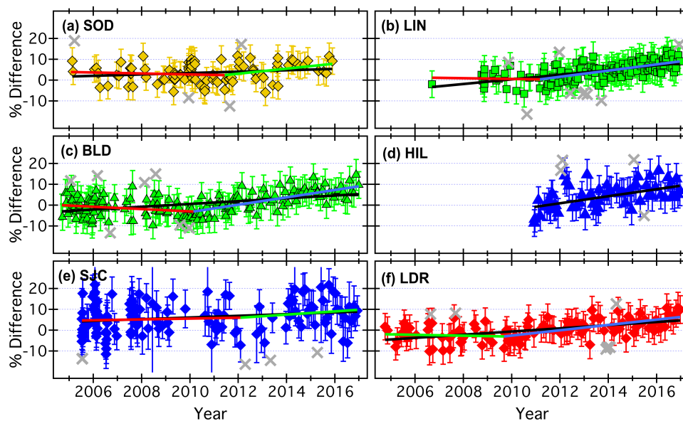
Figure 11. Timeseries-Time series of relative MLS-FP differences at 68 hPa over 6 different FP sites. As in Fig. 9, vertical error bars represent the uncertainties in differences and gray crosses are data points identified as outliers and omitted from the drift analyses. Black lines depict the trends determined by weighted linear regression fits to the entire records of differences. Colored lines show the linear trends in two distinct time periods (except at HIL) that are separated by a statistically significant changepoint, as determined by piecewise continuous weighted linear regression fits (see section 4.2.1).
