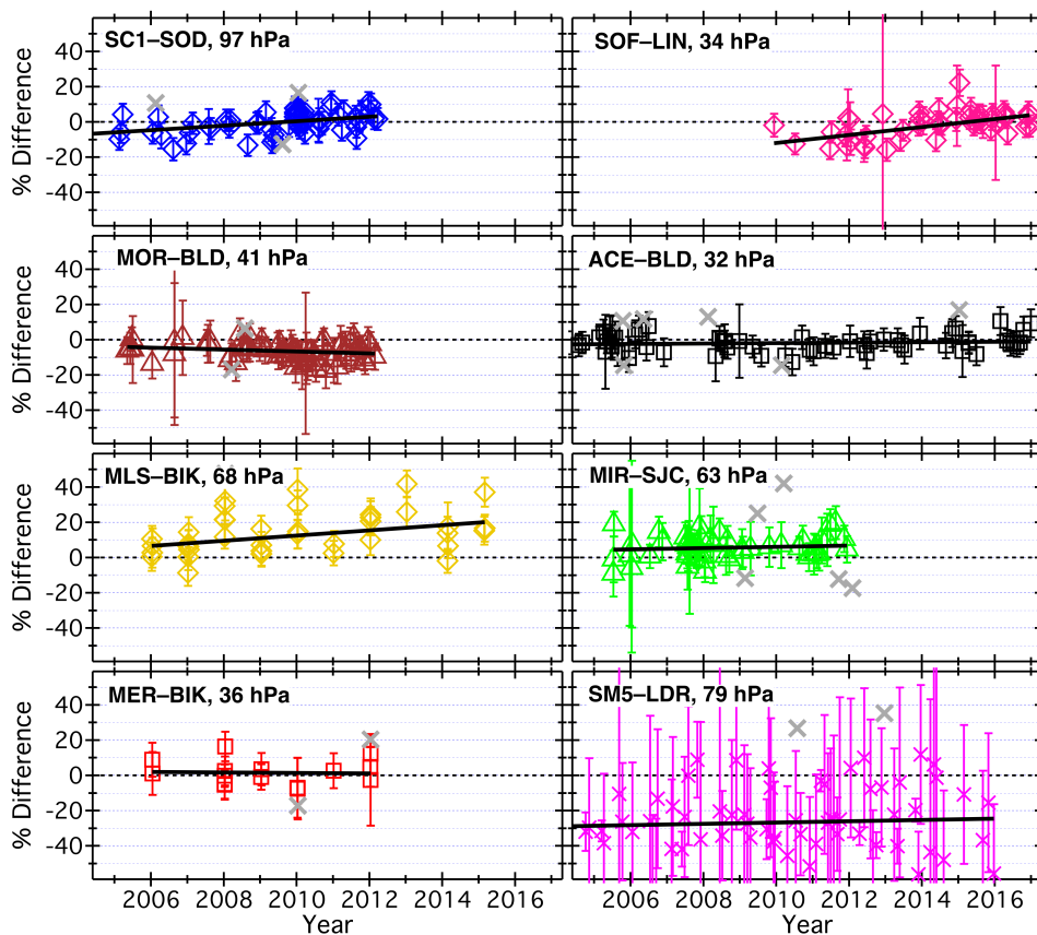
Figure 9. Timeseries-Time series of SAT-FP relative differences for 8 unique pairs of satellite retrievals and FP sites. See Tables 1 and 2 for the 3-letter codes that represent the relevant FP sites and satellite retrievals. The SAT reporting pressure for the timeseries-time series shown is given in each panel. Vertical error bars depict the uncertainties in SAT-FP differences that factor into the weighted linear regressions used to calculate the black trend lines. Gray crosses are data points identified as outliers and omitted from the analyses.
