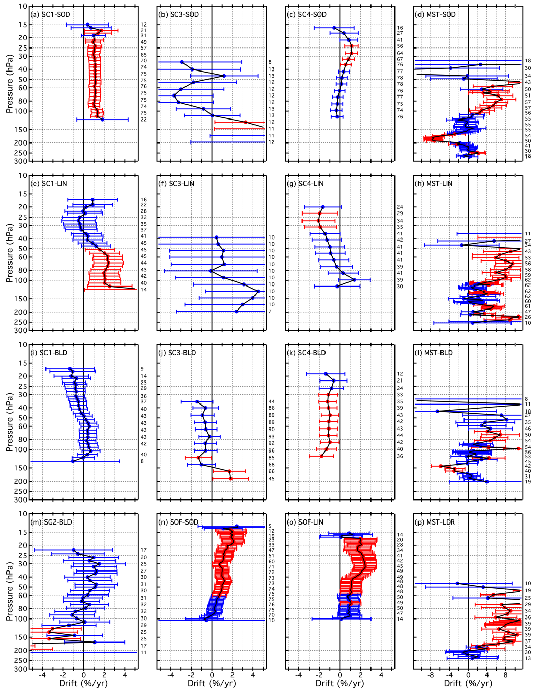
Figure B3. Same as Figure B1 for 16 additional SAT-FP pairings that include SC1, SC3, SC4, SG2, SOF, and MST. Note that the x-axis scale for the far right panels is substantially expanded to better show the drifts.
