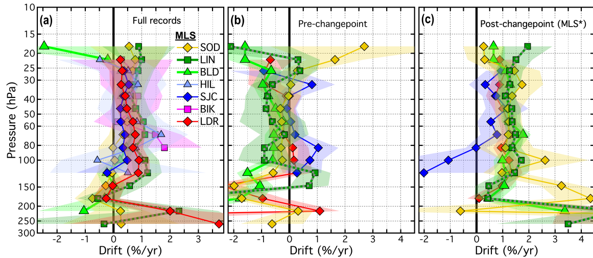
Figure 12. Vertical profiles of drifts in (a) MLS-FP differences spanning the entire records (2004-2016) and, (b) only those MLS-FP differences after for the ~2004 to ~2010 changepoint in each record pre-changepoint period, and (c) for the ~2010 through 2016 post-changepoint period (i.e., MLS*). The legend applies to both all three panels, but drifts at HIL and BIK are not available for MLS* panels (b) or (c). The colored-matched shading surrounding each profile represents the 95 % confidential intervals of the drifts over that site.
