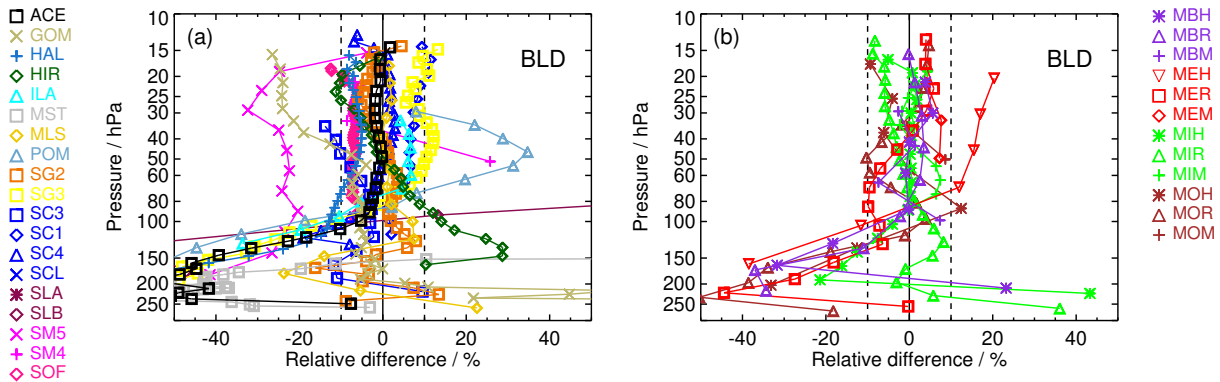
Figure 5. Mean relative differences between satellite and BLD FP profiles ( 40^{\circ} N). left panel a: all data records except MIPAS; right panel b: all MIPAS data records. The Details of color coding and symbols for the satellite records are provided in Fig. 2 and Tab. 2. The profiles were cut at the respective local tropopause before averaging.
