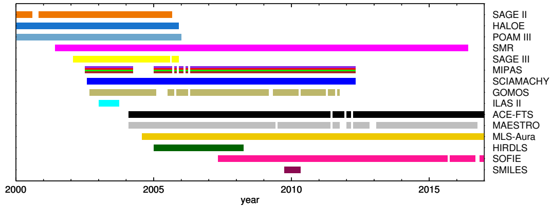
Figure 2. Colors, symbols, and three-letter code codes for the satellite data records used throughout the paper (upper part) and temporal distribution of available data of the respective satellite instruments on a monthly basis until the end of 2016 (lower part, not divided into measurement modes or data versions). Note that three of the SAT data sets began before 2000 (SAGE II 1984, HALOE 1991, POAM III 1998), but only the data from 2000 through 2016 are used here for bias and drift evaluations.
