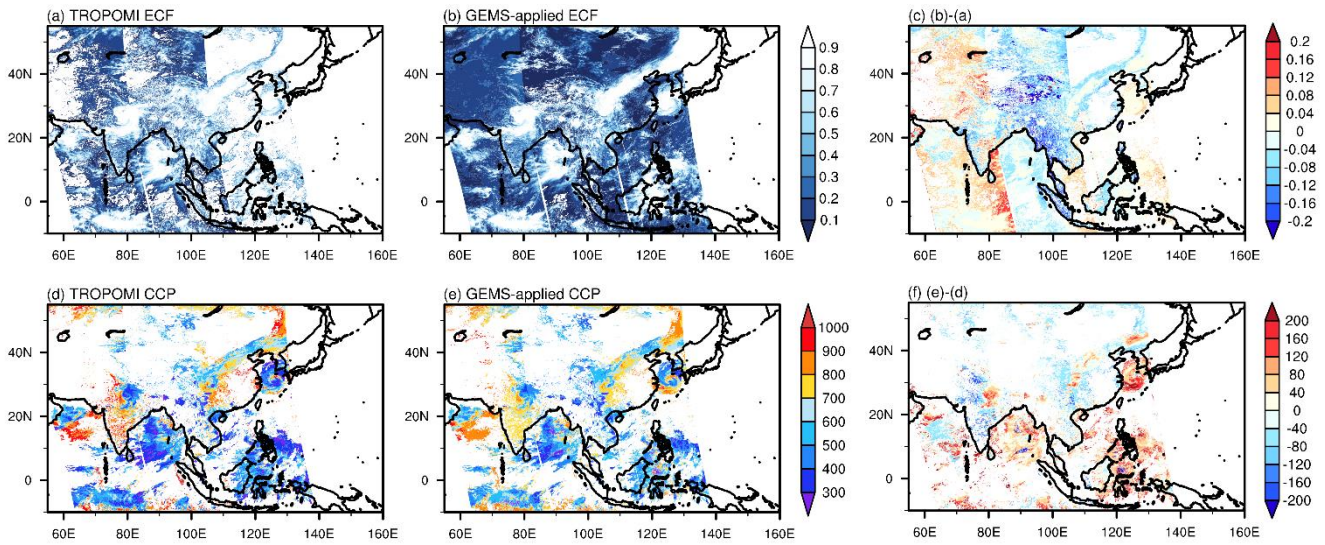
610 Figure 5: This figure, similar to Figure 2, shows the validation of the GEMS cloud retrieval algorithm using TROPOMI data. Cloud retrievals were performed using observations from September 16, 2021, as input. (a) TROPOMI CF converted to ECF. (b) ECF derived from GEMS using TROPOMI L1B as input. (d) CP retrieved from TROPOMI. (e) CCP image retrieved by GEMS cloud retrieval algorithm. (c) and (f) Differences in cloud retrievals between GEMS and TROPOMI algorithms.
