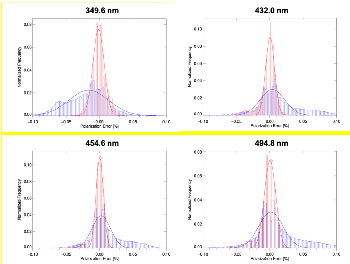
Figure 8: Histograms of the polarization error before (blue) and after (red) polarization correction.
