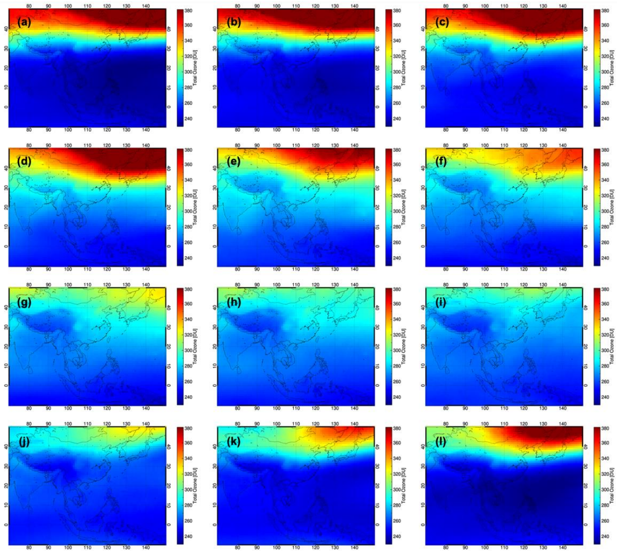
Figure 5: The distribution of the total column ozone climatological data within the GEMS observation domain. The dataset was created based on the OMI L2 product OMT03. (a)-(l) represent the annual variation sequentially from January to December.
