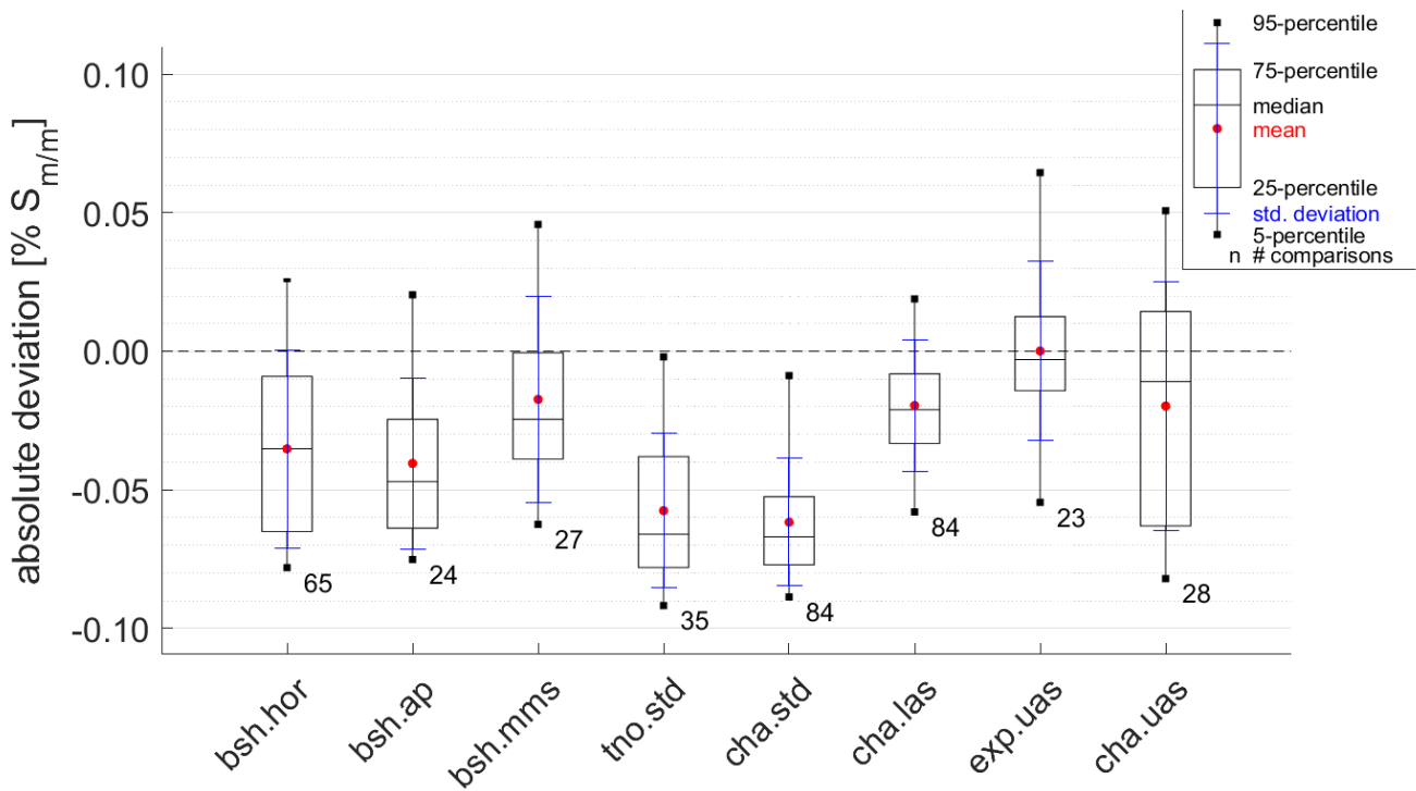
330 Figure 3: Comparison of the deviations per system from the expected FSC determined by fuel sampling or BDN. The number next to each bar corresponds to the number of observations.
