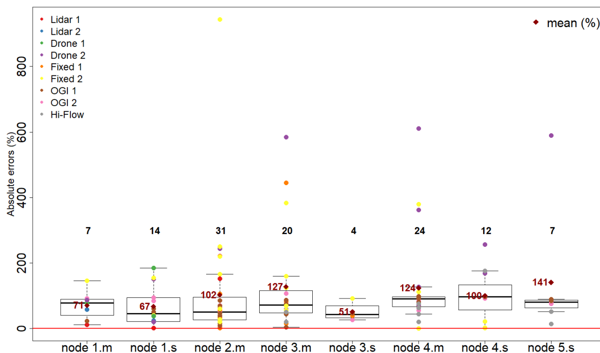
Figure 7: Comparison of absolute errors for single node releases (“.s”) and multiple node releases (“.m”). Excluding the releases of 0.1 kg h -1 or less. Each point is a participant’s node-level estimate.
