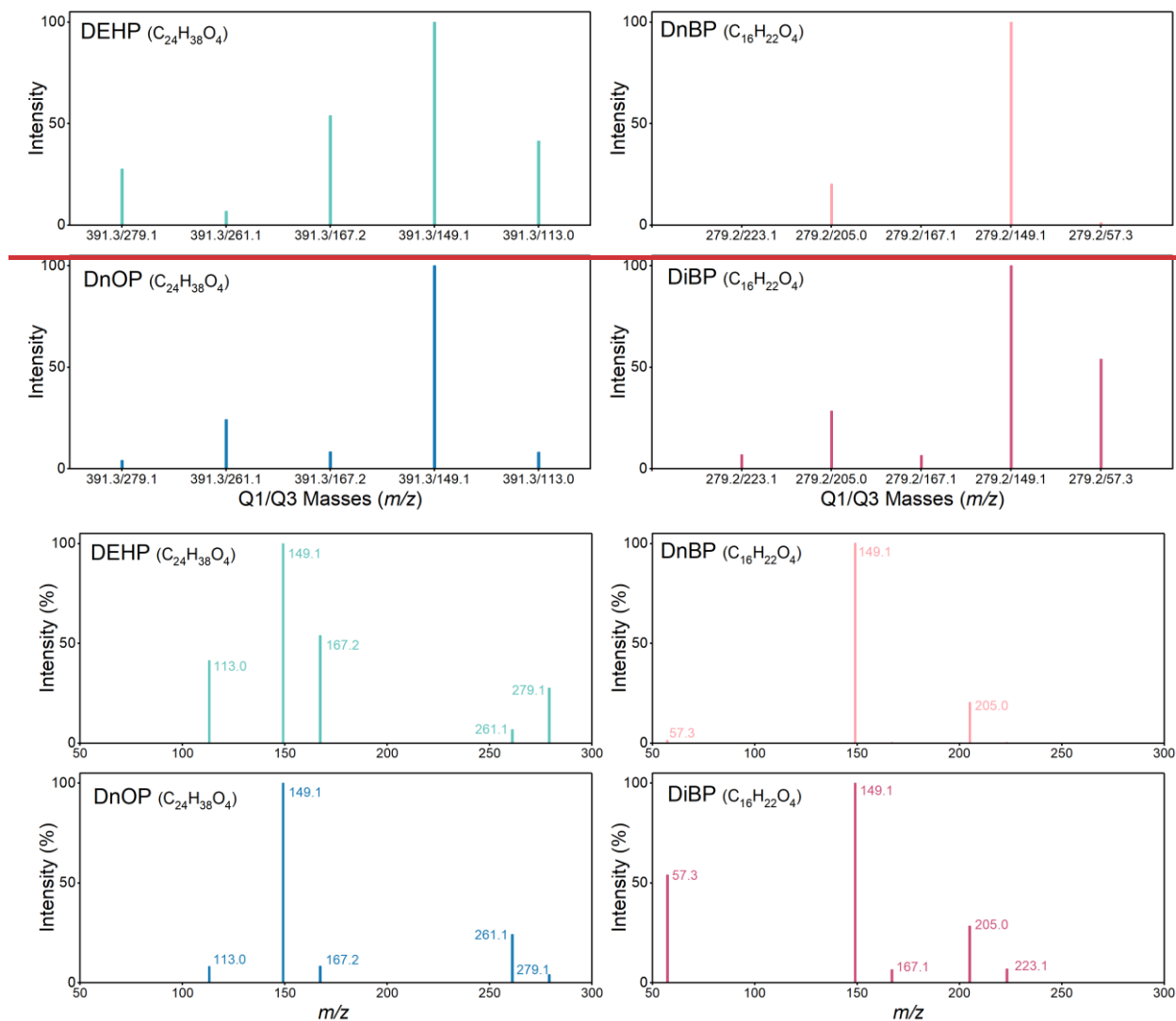
Figure 2: Relative intensity of selected product ions of DEHP/DnOP at m/z 391.3 (left) and DnBP/DiBP at m/z 279.2 (right).
