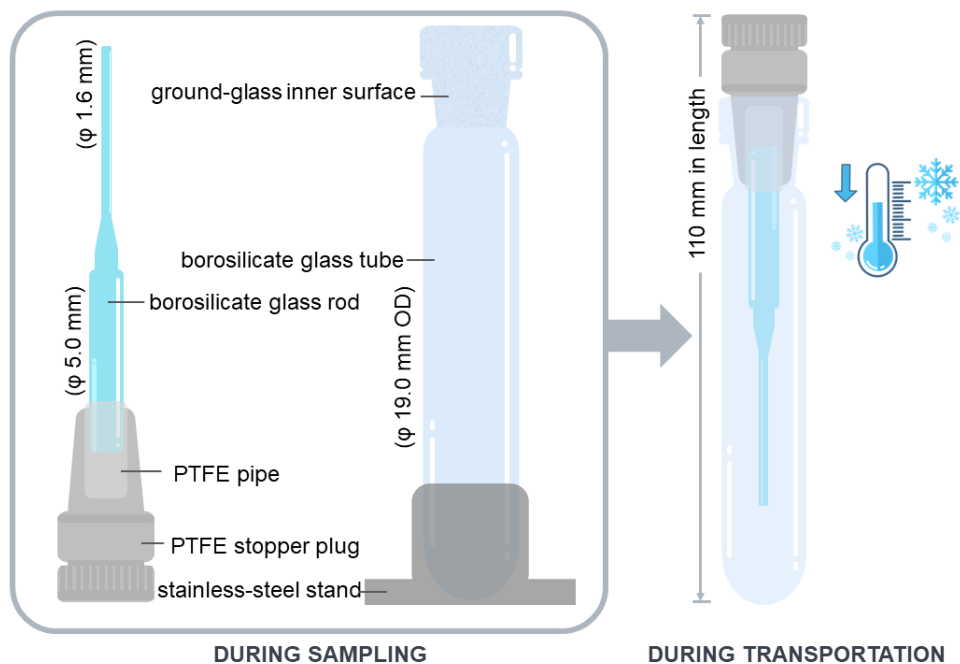
275 Figure 1: Schematic of indoor surface film passive sampling suite.
