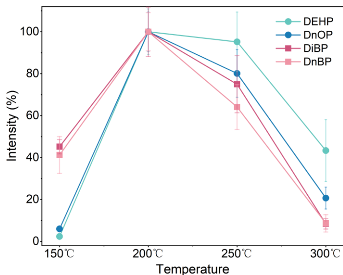
280 Figure 3: Relative intensities for 0.05 ng spiked DEHP, DnOP, DiBP and DnBP at different He flux temperature.
