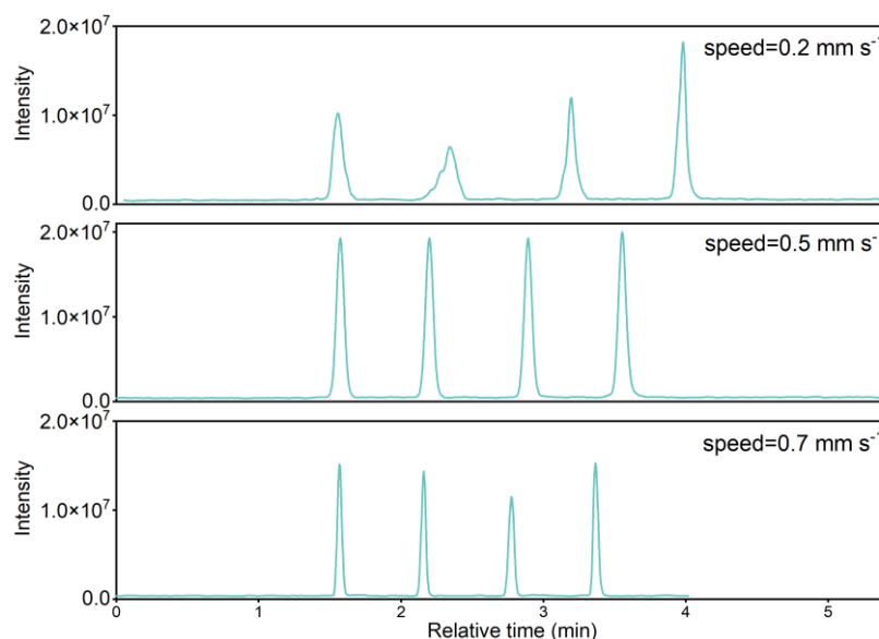
285 Figure 5: The influence of speeds of motorized linear rail on the total ion chromatograms (TIC) for spiked DEHP within 5 minutes. The He flux temperature was set as 200°C. The rod distance was 18 mm.
