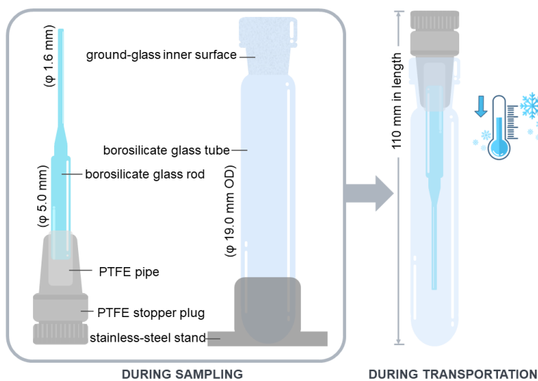
265 Figure 1: Schematic of indoor surface film passive sampling suite.
