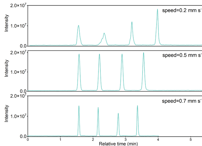
Figure 5: The influence of speeds of motorized linear rail on the total ion chromatograms (TIC) for spiked DEHP within 5 minutes. The He flux temperature was set as 200°C. The rod distance was 18 mm.
