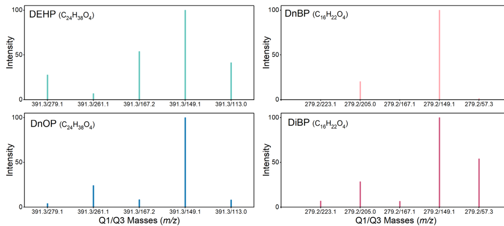
Figure 2: Relative intensity of product ions of DEHP/DnOP at m/z 391.3 (left) and DnBP/DiBP at m/z 279.2 (right).
