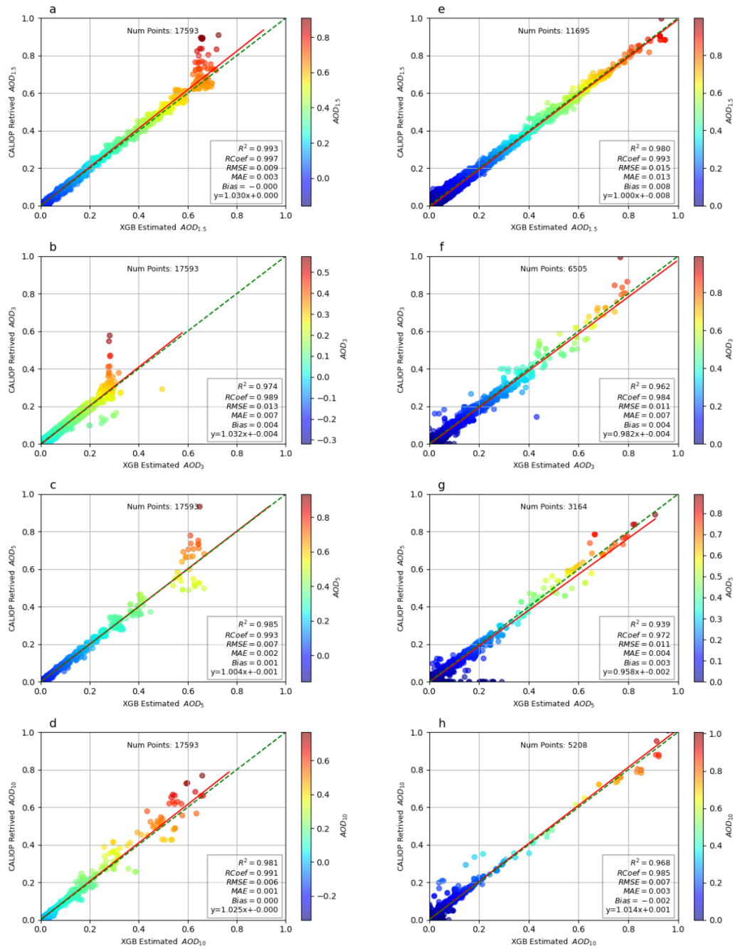
Figure 7. Scatterplots comparing the estimated SEVIRI multi-layer AOD values derived from the proposed machine learning models with the CALIOP AOD profiles for the year 2019. The red line represents the linear fit between the two datasets.
