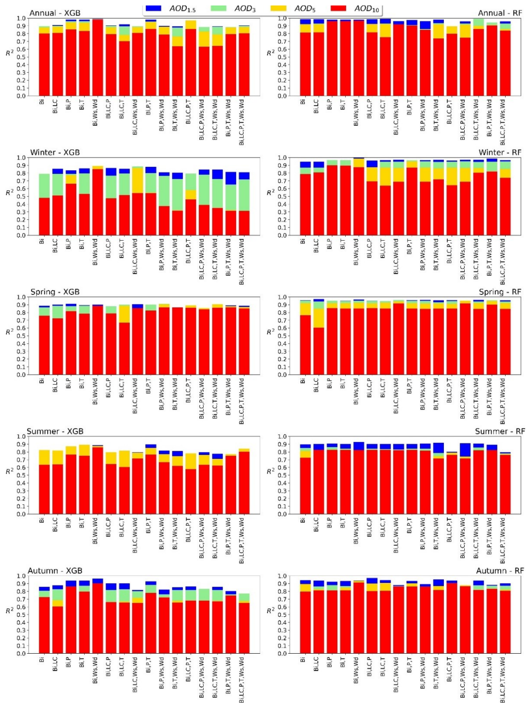
Figure 6. The impacts of input features on the retrieval of SEVIRI multi-layer AOD values, represented as R^2 metrics, for the RF and XGB models. Each row displays the results for the
