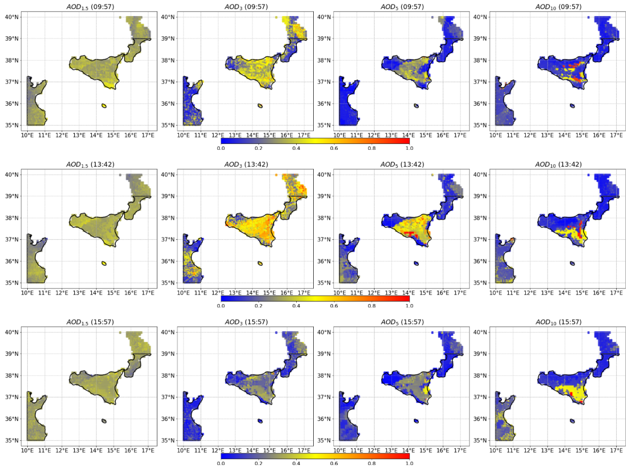
Figure 11. Spatial distributions of estimated multi-layer AOD values during the Volcanic Eruption on August 14, 2023, at selected times.
