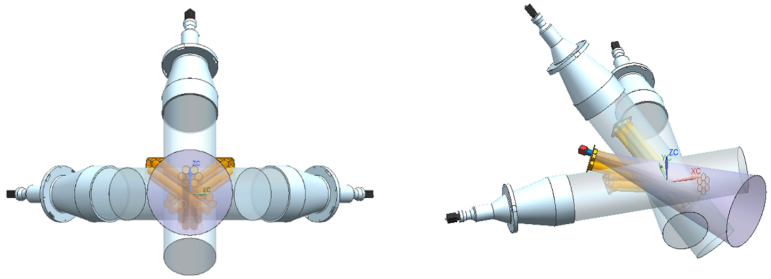
Figure 2. The observation volume of the three telecentric lenses and LED lighting beams.
