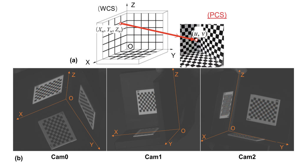
Figure 5. (a) 3D checkerboard calibration principle; (b) World coordinate system WCS with three camera views.
