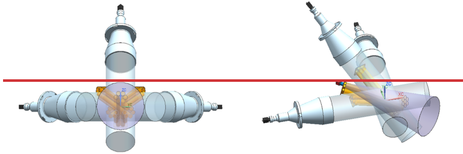
Figure 2. Optical structure of 3D-PPI
