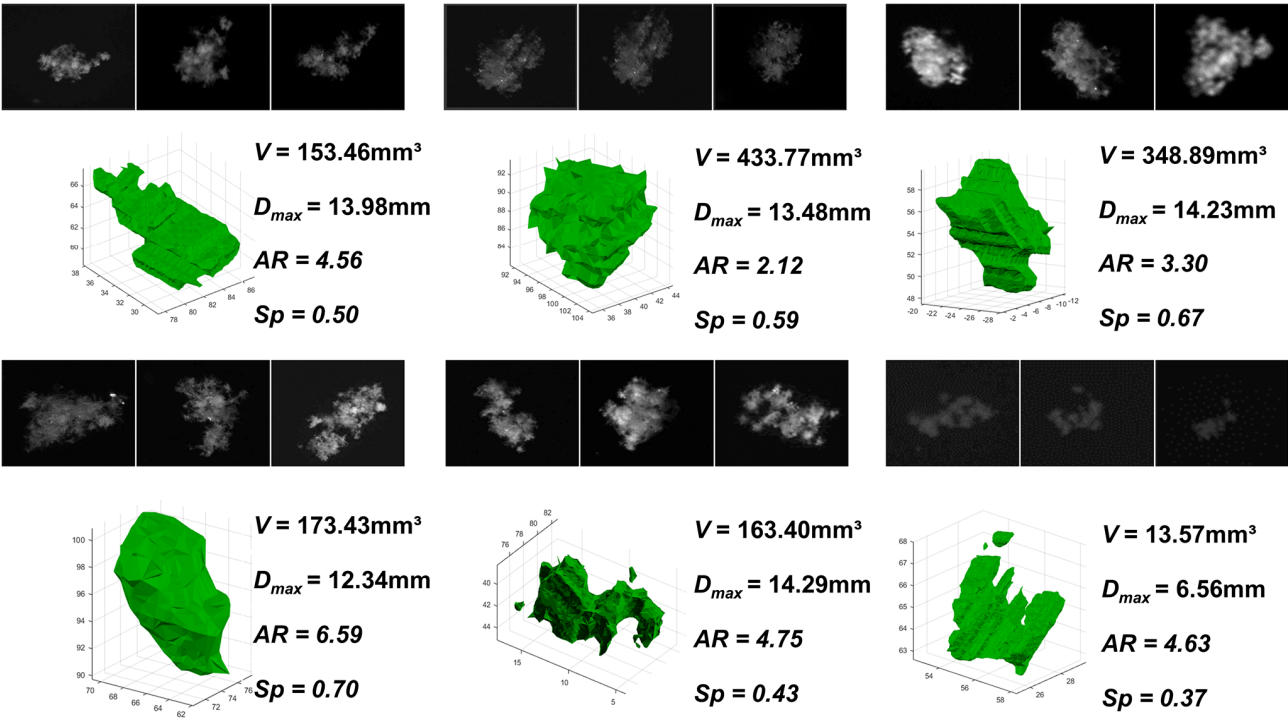
485 Figure 14. Several typical snowflakes captured by 3D-PPI in the field and the corresponding 3D reconstruction results. For each reconstruction, the computed V , D_{max} , AR , and Sp .
