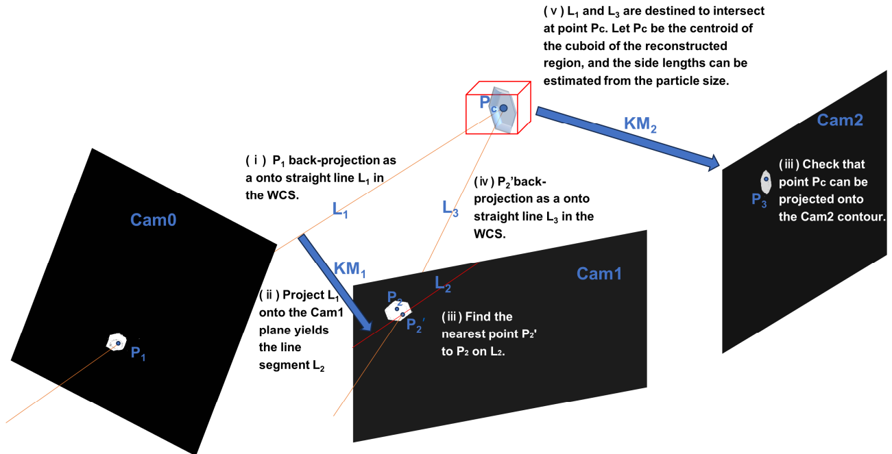
Figure 11. Steps to locate localize the 3D spatial particle position in the WCS according to the image particle contours
