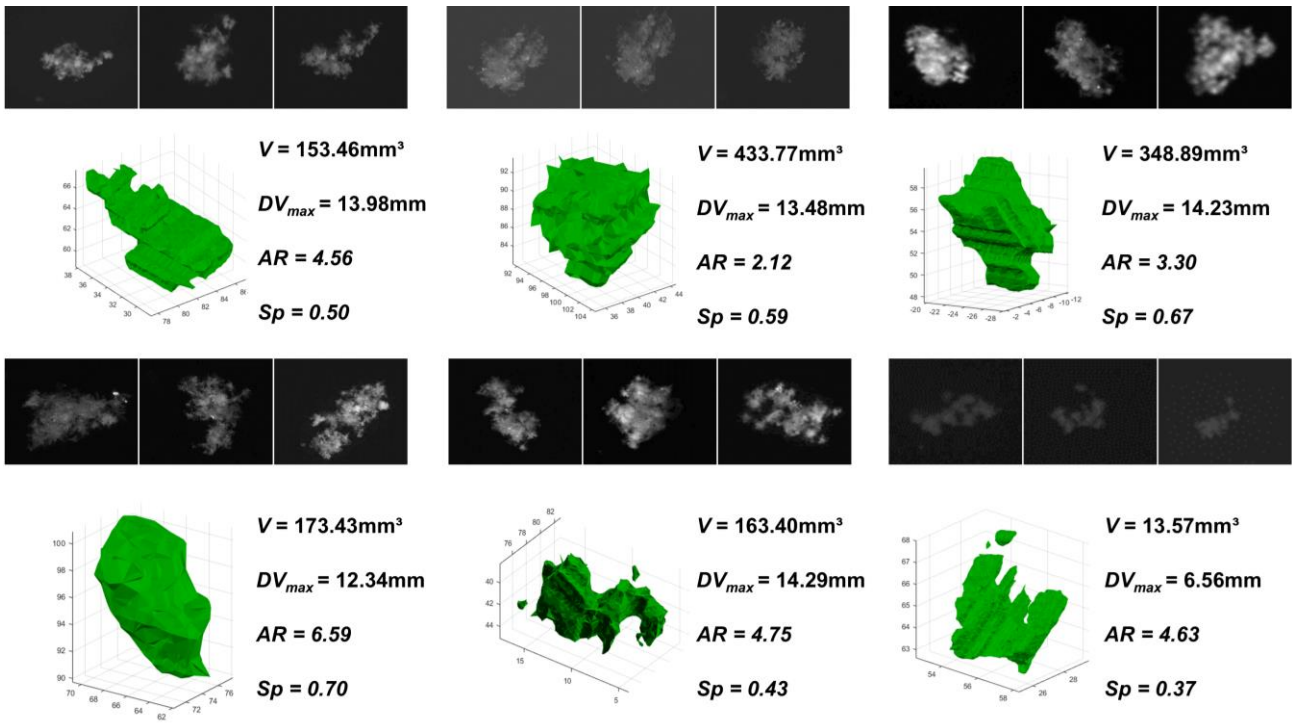
Figure 14.13. Several typical snowflakes captured by 3D-PPI in the field and the corresponding 3D reconstruction results. For each reconstruction, the computed V , D_{max} , DV_{max} , AR , and Sp .
