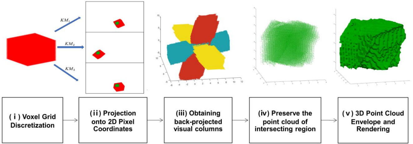
385 Figure 4211. Flowchart of 3D construction algorithm
