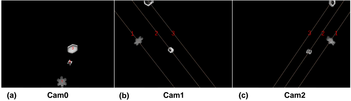
Figure 109. The three particles detected in Cam0 can only appear on the corresponding three line segments in Cam1 and Cam2 respectively
