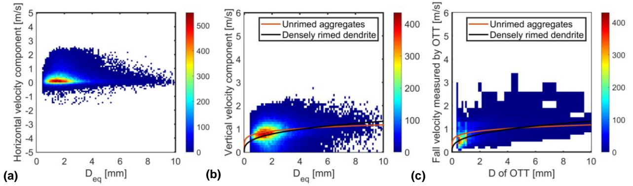
Figure 15. Distribution of horizontal (a), and vertical (b) snowflake velocities with D_{eq} measured by 3D-PPI. Distribution of falling velocity with diameter measured by OTT (c). The color scale denotes the number of snowflakes measured.
