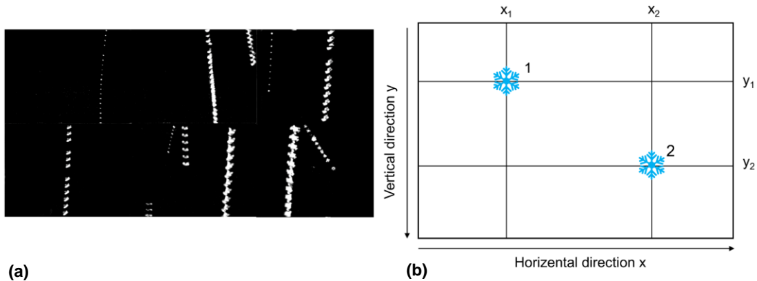
465 Figure 15.14. (a) Processed high-speed camera images, and then the same particles from consecutive frames are merged into a single image (a) ; (b) Speed Measurement Schematic (b) .
