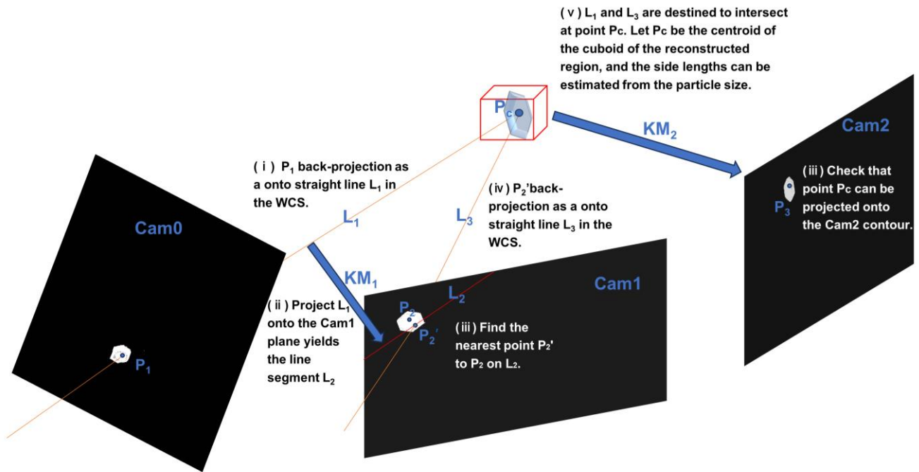
Figure 4.10. Steps to localize the particle position in the WCS according to the image particle contours
