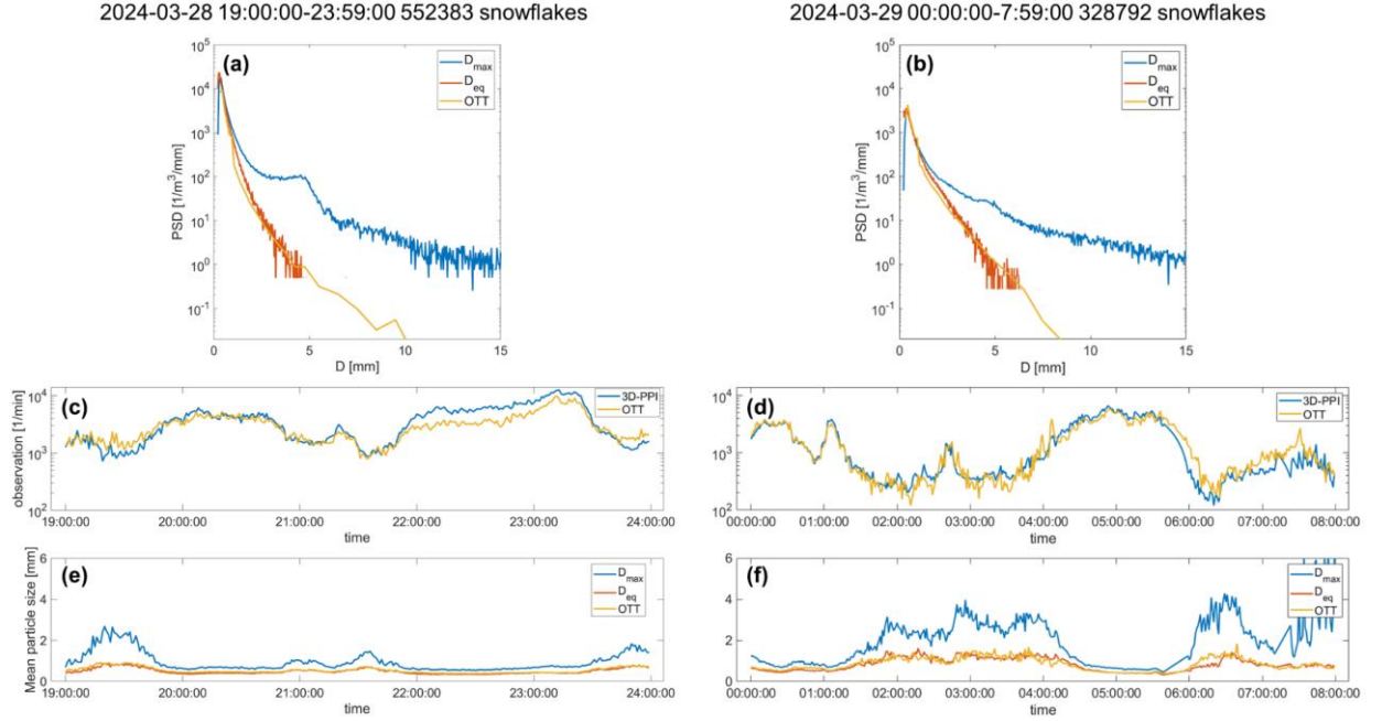
Figure 13.12. This typical continuous snowfall was split into two days and plotted separately (left and right). The 1-minute particle size distribution (PSD) of the D_{max} (blue) and D_{eq} (orange) for 3D-PPI and OTT (yellow) for the snowfall case (first row). Temporal plot of average particle counts per unit volume per minute over two days (second row). Temporal plot of average particle size per minute over time (third row).
