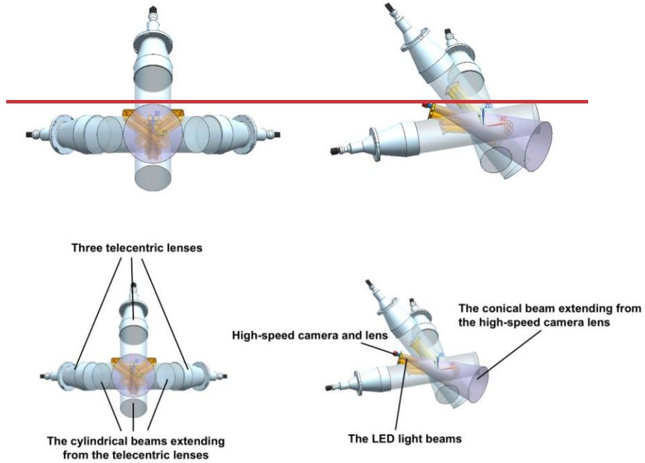
115 Figure 2. The two views of three telecentric four cameras and lenses and , including the additional beams extending from the lenses and the LED light beams.
