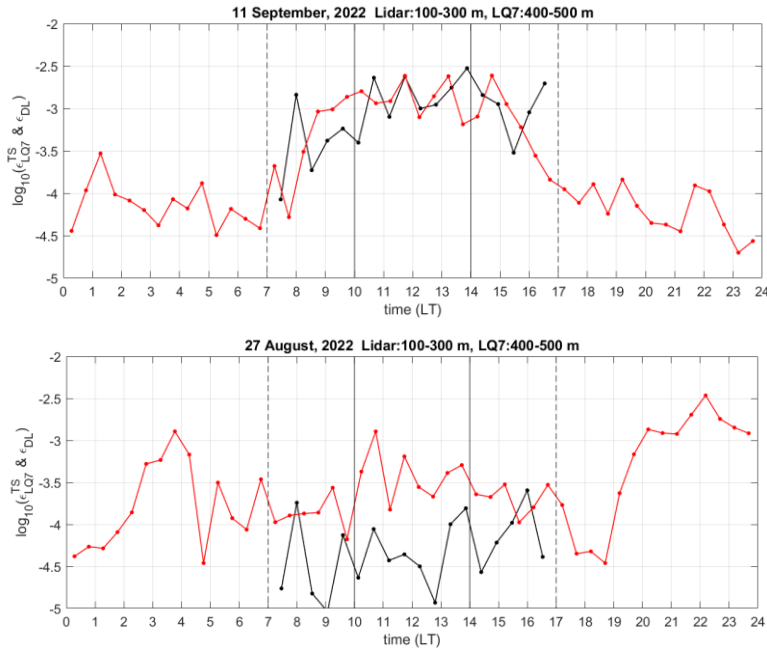
335 Figure 7: Time series of \log_{10}(\varepsilon_{LQ7}^{TS}) (black) in the [400-500] m height range and \log_{10}(\varepsilon_{DL}) (red) in the [100-300] m height range on 11 September, 2022 (top) and 27 August, 2022 (bottom) at a time resolution of 1 hour sampled every 30 min. The vertical solid black lines show the [10:00-14:00] LT time range used to compute the mean spectra shown in Fig. 6. The vertical dashed black lines show the [07:00-17:00] LT time range shown in Fig. 5. \varepsilon_{LQ7}^{TS} before 07:00 LT and after 17:00 LT is not shown because the raw LQ7 data are strongly corrupted by biological targets (birds and/or bats).
