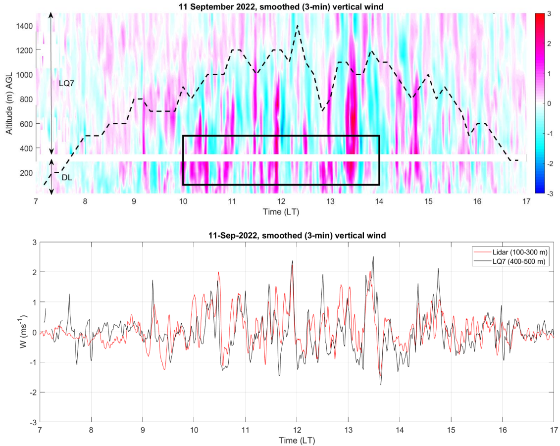
Figure 5a: (top) Time-height cross-section of smoothed (3-min) values of vertical winds from LQ7 (400~) and DL (20-300 m) on 11 September, 2022 and from 07:00 LT to 17:00 LT. The proxy for the CBL top height is given by the dashed line. The black rectangle shows the time-height domain used to estimate W spectra shown in Figure 6. (Bottom) The corresponding time series of W for DL (red) averaged in the [100-300] m height range and for LQ7 (black) averaged over two consecutive sampled heights (400 and 500 m).
