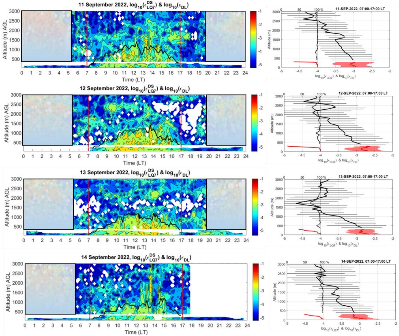
Figure 9a: (Left) Time-height cross-section of \log_{10}(\epsilon_{LQ7}^{DS}) estimated from eq. 2 and \log_{10}(\epsilon_{DL}) for 4 successive days from 11 September to 14 September 2022 up to the height of 3000 m. The translucent rectangles in \log_{10}(\epsilon_{LQ7}^{DS}) cover areas strongly affected by biological targets. The bold solid line shows the CBL top height from LQ7 echo power data. The two vertical red lines mark 07:00 and 17:00 LT. (Right) The corresponding profiles of \log_{10}(\epsilon_{LQ7}^{DS}) (black) and \log_{10}(\epsilon_{DL}) (red) averaged over 10 hours between 07:00 and 17:00 LT. The horizontal lines show the standard deviation. The thick dotted black and red curves show the data availability between 0 and 100 % for LQ7 and DL, respectively.
