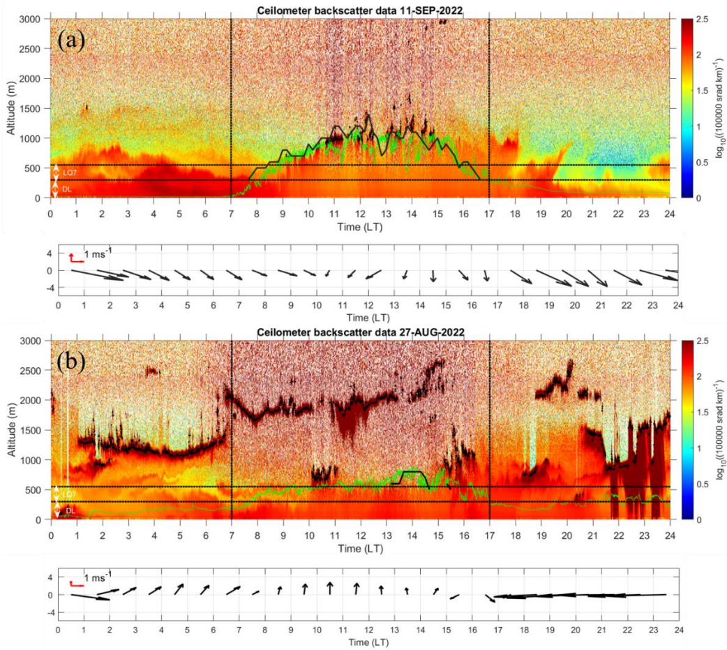
230 Figure 4. Time-height cross-sections of Vaisala ceilometer CL31 (910 nm) backscatter data (in \log_{10}(10^5 \text{ srad km}^{-1}) ) at a time and range resolution of 15 s and 20 m, respectively, from the ground to the height of 3000 m for 11 September, 2022 (Fig. 4a) and 27 August, 2022 (Fig. 4b). The black arrows indicate the hourly winds measured by the DL in the 40-300 m height range. The blue curve shows the height of the lifting condensation level (LCL) calculated from the surface meteorological data from the Automatic Weather Station (AWS). The thick black curve shows the height of the CBL top estimated from the identification of the maximum of the LQ7 echo power. The double arrows and horizontal lines indicate the range used to calculate the TKE dissipation rates from LQ7 and DL. 235
