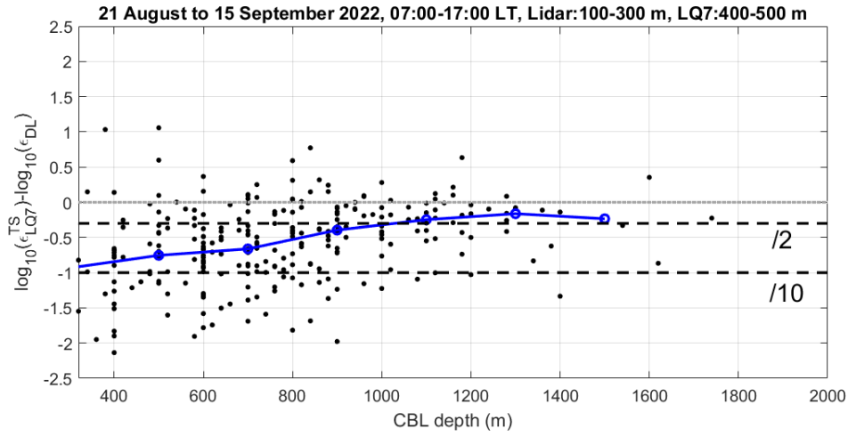
340 Figure 8: Scatter plot of 1-hour averaged \log_{10}(\epsilon_{LQ7}^{TS}/\epsilon_{DL}) vs CBL depth (m) for 23 days during the period 21 August to 15 September, 2022 excluding periods of precipitations. The blue curve shows the trend obtained by averaging \log_{10}(\epsilon_{LQ7}^{TS}/\epsilon_{DL}) over segments of 200 m.
