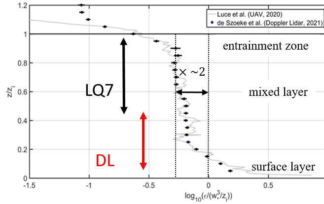
Figure 13: Vertical mean profiles of normalized TKE dissipation rates measured by DataHawk UAVs (Luce et al., 2020) and by a Doppler lidar (De Szoeko et al., 2021). The range of observations from DL and LQ7 are indicative.
