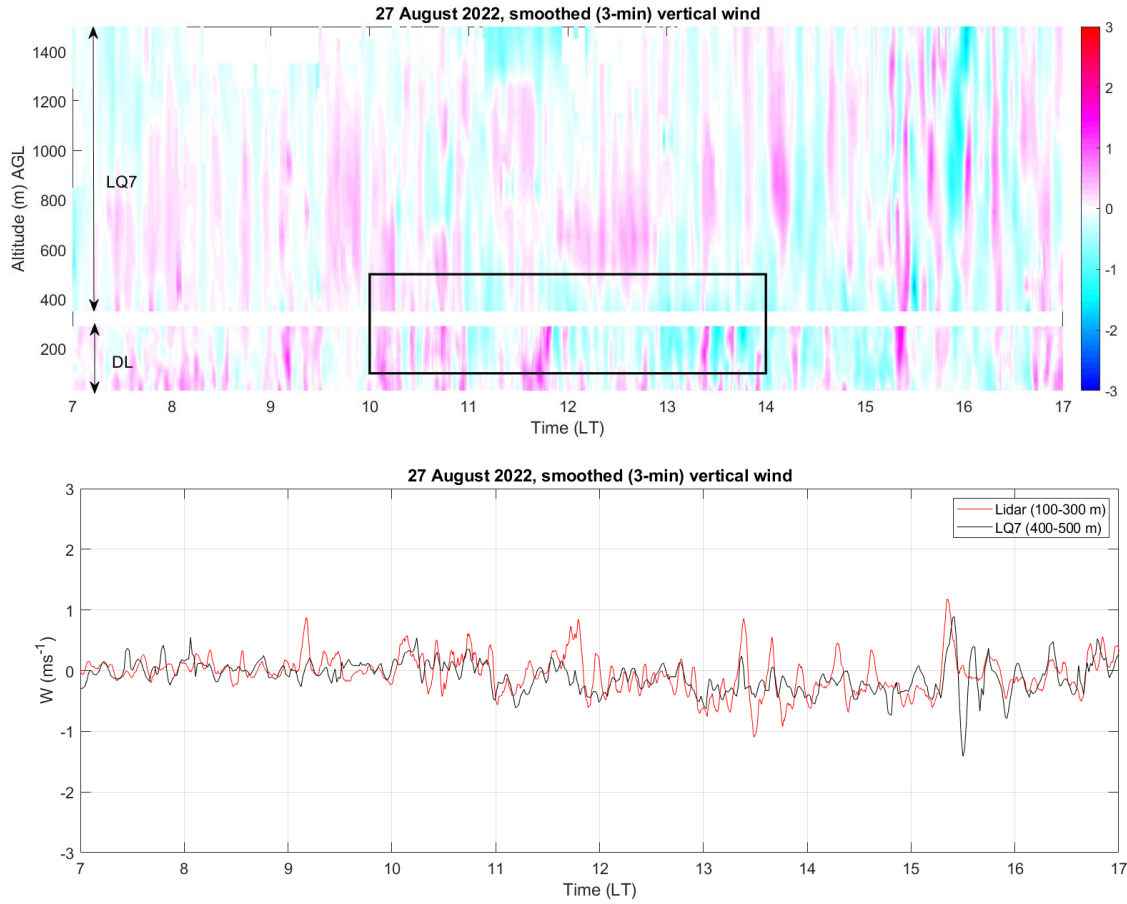
270 Figure 5b: Same as Fig. 5a on 27 August, 2022.
