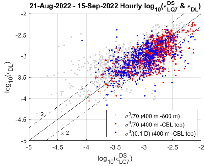
390 Figure 10: Scatter plot of range (100-300 m) and hourly mean \log_{10}(\epsilon_{DL}) using the TS method vs hourly mean \log_{10}(\epsilon_{LQ7}^{DS}) averaged between 400 m and 800 m with L = 70 m (grey dots), between 400 m and the (variable) altitude of the CBL top (red dots) and between 400 m and the (variable) altitude of the CBL top with L = 0.1 D (blue dots) in the [07:00-17:00] LT time range and for 23 days between 21 August and 15 September 2022, excluding rain periods.
