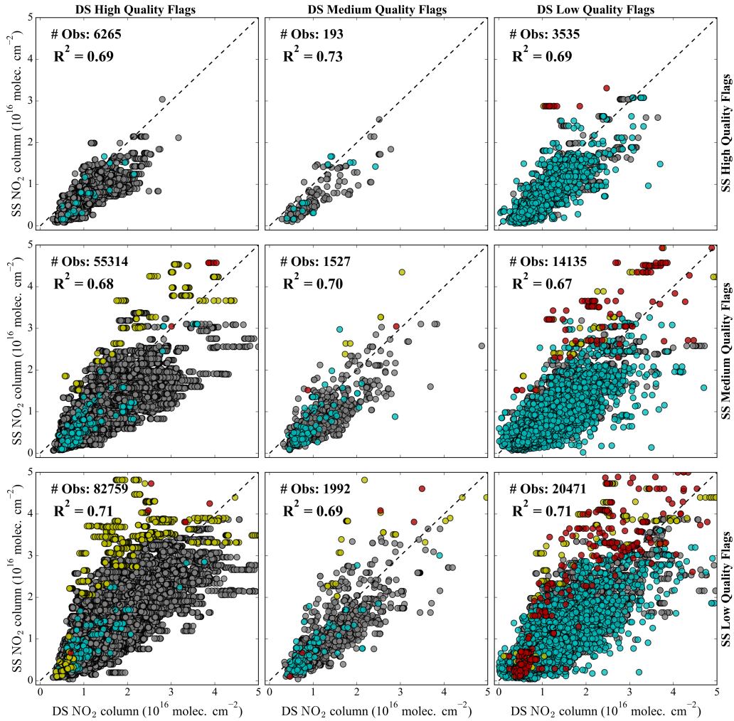
315 Figure 8. Correlation of contemporaneous DS and SS observations of \text{NO}_2 column for different quality flag combinations at the University of Houston Pandora site for 2021 – 2022. Data points are colored by cutoff values used for \text{NO}_2 column independent uncertainty values. Gray indicates points for which both DS and SS uncertainties are less than the cut-off, other colors indicate points for which only DS (cyan), only the SS (yellow), or both DS and SS (red) uncertainties exceed the cut-off value.
