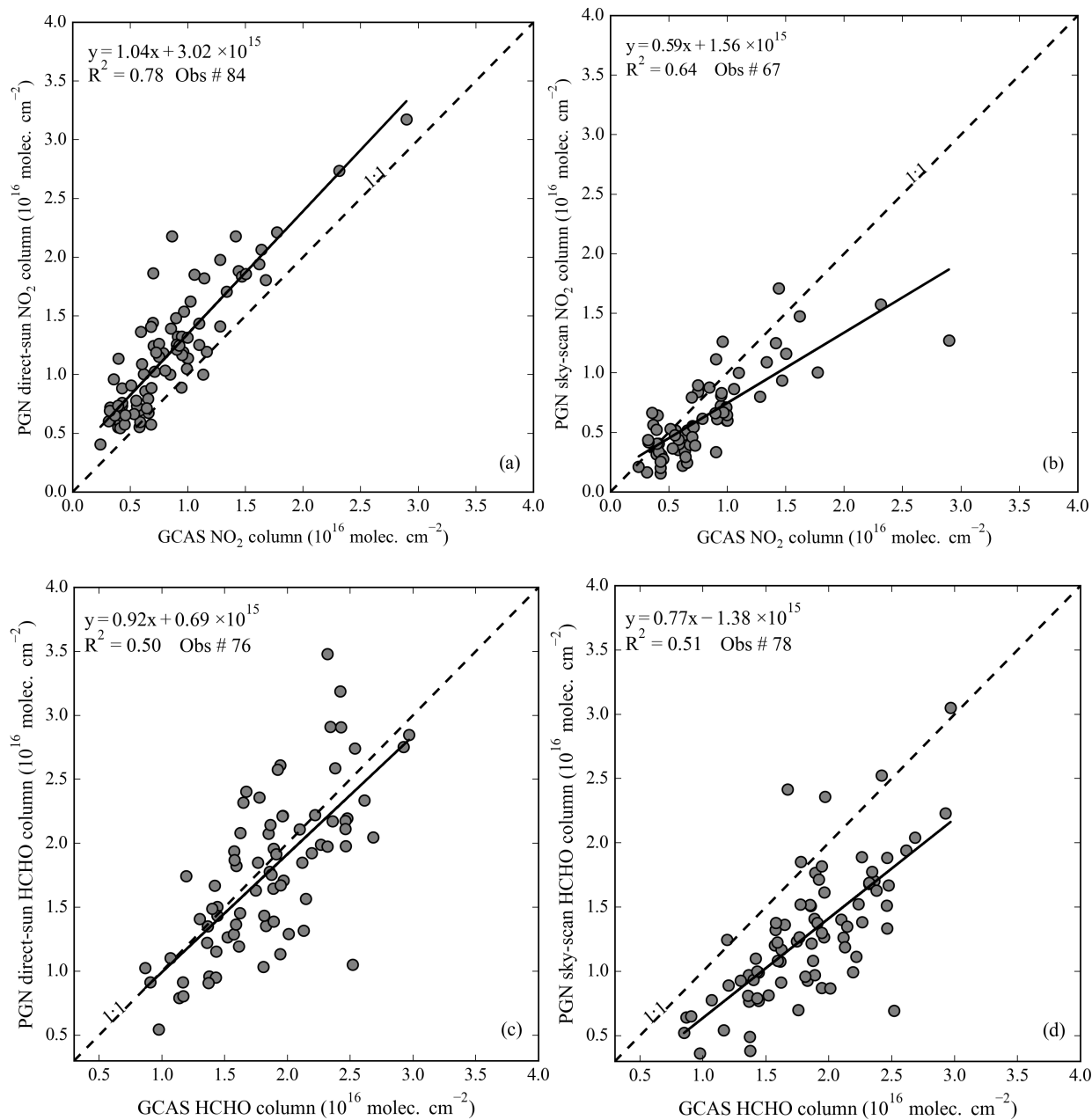
Figure 13. Comparison of airborne GCAS trace gas columns with and Pandora columns of \text{NO}_2 (panels a and b) and HCHO (panels c and d) during TRACER-AQ for Houston Pandora sites (Aldine, La Porte, and University of Houston). Comparisons are shown for both direct-sun (panels a and c) and sky-scan (panels b and d) modes.
