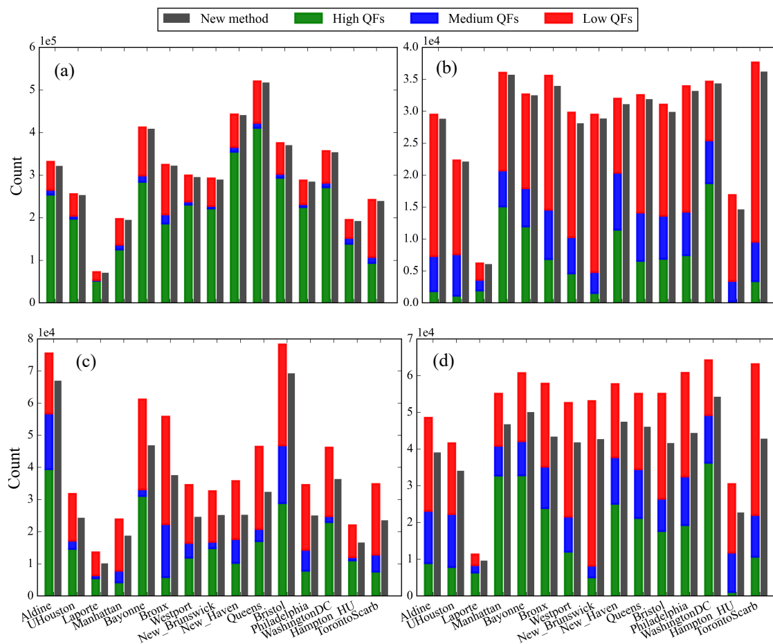
370 Figure 11. Quality flags (QFs) for each Pandora site in 2021-2022 (left bars) colored by green (high), blue (medium), and red (low) for (a) NO 2 DS, (b) NO 2 SS, (c) HCHO DS, and (d) HCHO SS. Adjacent grey bars show total observation counts after applying the new filtering method.
