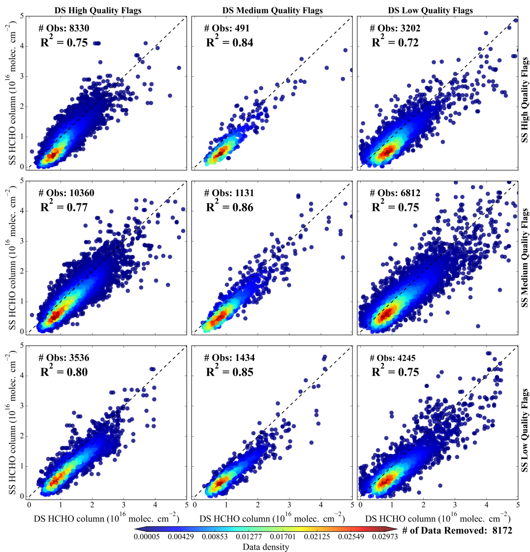
310 Figure 7. Correlation of contemporaneous DS and SS observations of HCHO column for different quality flag combinations after applying new filtering method to the University of Houston Pandora site for 2021-2022. Data points are colored by normalized gaussian kernel density of data.
