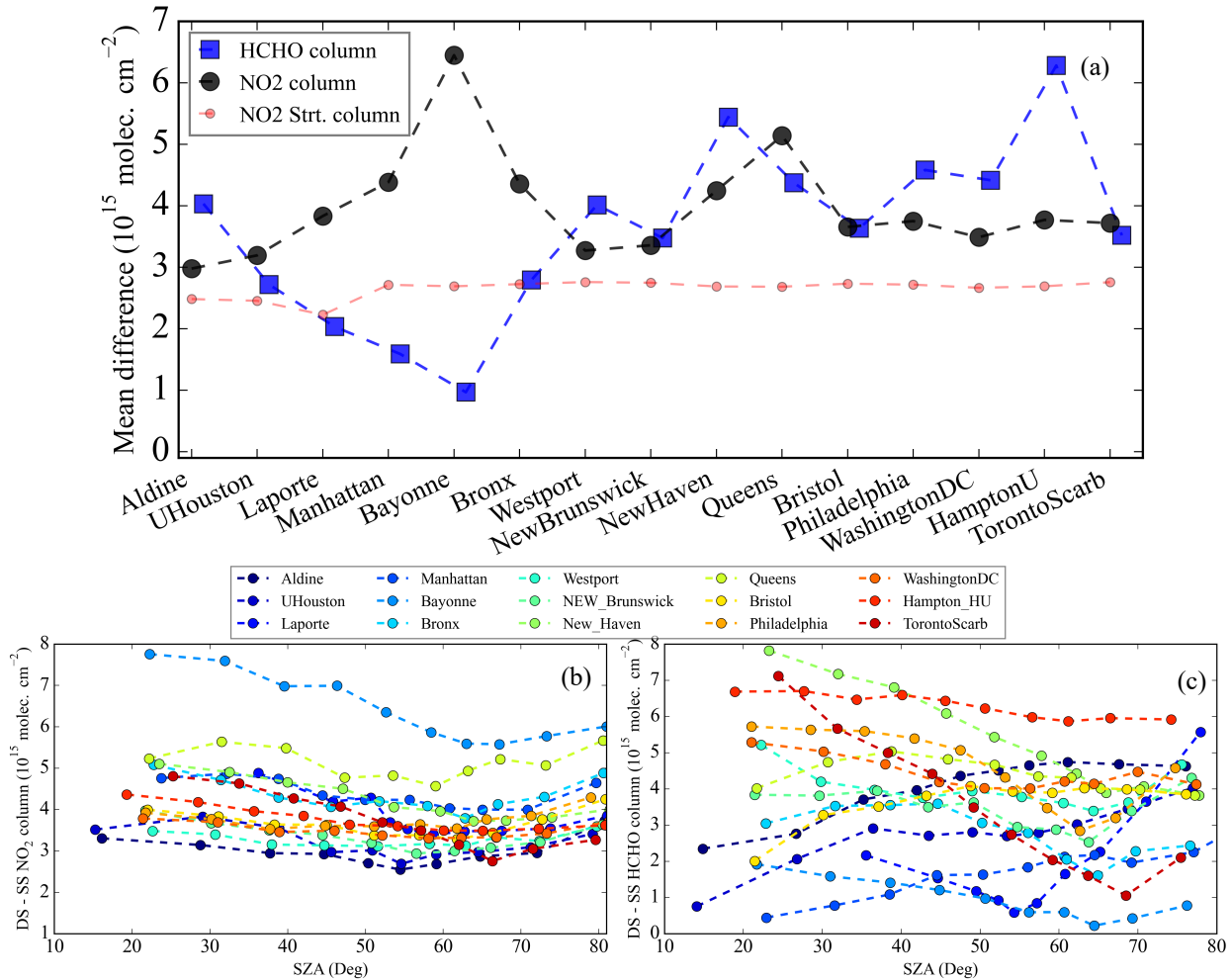
540 Figure 14. (a) Mean differences between the DS and SS column for HCHO and NO 2 over the 15 Pandora sites for 2021-2022. The NO 2 stratospheric column for each site is also provided. Bottom panels show the variation of mean column difference with SZA for NO 2 column (b) and HCHO columns (c), respectively.
