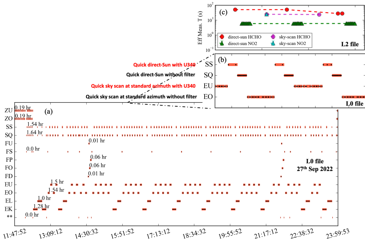
170 Figure 2. (a) Pandora standard schedule of operations (UTC hour) on a clear sky day on 27 Sep 175 2022 at the University of Houston site for different observing modes with a zoomed-in, 18-minute window for both L0 (b) and L2 (c) file information. The black points in the L0 schedule show the start of each measurement time and underlying red line is the total time in that respective mode. The L2 data (c) shows the alternating retrieval of NO 2 (without filter) and HCHO (with U340 filter) column from direct-sun and sky-scan modes.
