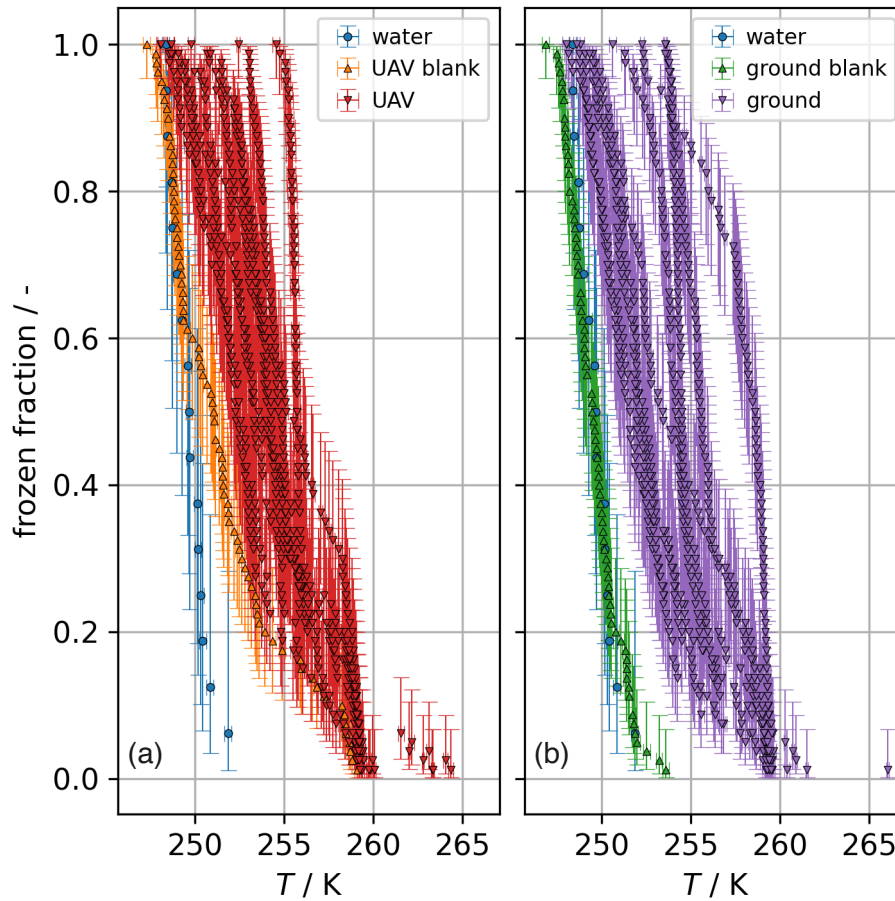
Figure 6. The frozen fraction as a function of the freezing temperature T is shown for the UAV filter suspensions from campaign 2 in comparison to its blank filter suspension and the Nanopure water background (left-panel (a)). The right-panel Panel (b) shows the equivalent for the ground filters. The blanks were handled the same way as the filter, but the pump was not turned on, and the UAV was not flying (see Sect. 2.4). The errorbars represent the 95% confidence interval.
