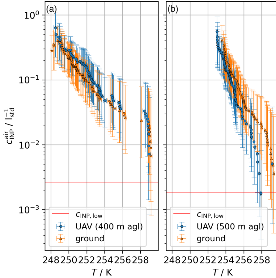
Figure 7. The left panel (a) shows the INP concentration in air, c_{\text{INP}}^{\text{air}} , at 400 m agl as a function of the freezing temperature, T , for a UAV and a ground (GR) filter during campaign 2. Both filters agree very well with each other. On the right panel (b), the same is shown for two filters one day after at 500 m agl. This filter was flown two times, doubling its sampling time and therefore increasing the amount of air sampled (note also the decreased lower detection limit as a red horizontal line, Eq. (3)). It can be seen that lower INP concentrations can be detected, as well as a steeper freezing curve due to the increased sampling time. The freezing curve does not reach the water background on the right panel (b). This is due to the fact that no dilution was prepared, and therefore the water background was not reached with the higher amount of INPs that can freeze a well. The errorbars represent the 95 % confidence interval.
