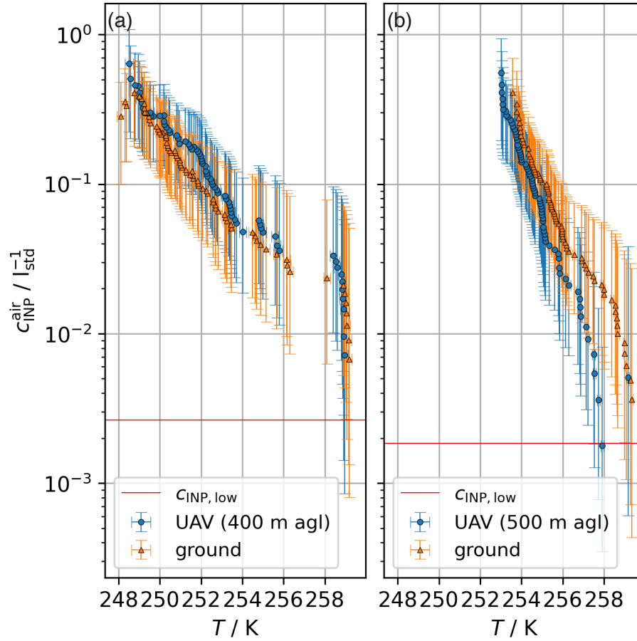
Figure 7. Panel (a) shows the INP concentration in air, c_{\text{INP}}^{\text{air}} , at 400 m agl as a function of the freezing temperature, T , for a UAV and a ground (GR) filter during campaign 2. Both filters agree very well with each other. On panel (b), the same is shown for two filters one day after at 500 m agl. This filter was flown two times, doubling its sampling time and therefore increasing the amount of air sampled (note also the decreased lower detection limit as a red horizontal line, Eq. (3)). It can be seen that lower INP concentrations can be detected due to the increased sampling time. The freezing curve does not reach the water background on panel (b). This is due to the fact that no dilution was prepared, and therefore the water background was not reached with the higher amount of INPs that can freeze well. The errorbars represent the 95 % confidence interval.
