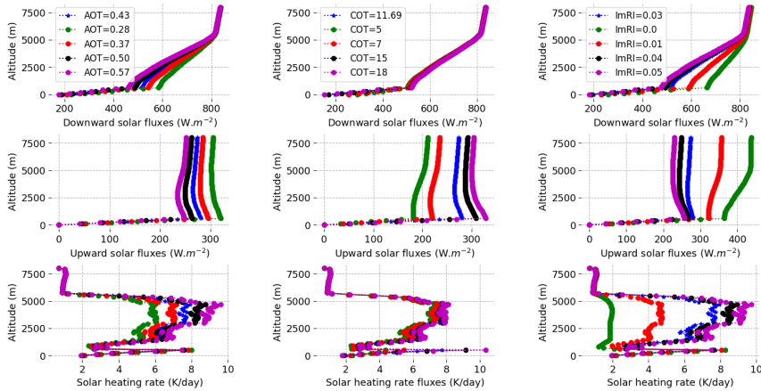
Figure 2: Impact of aerosol and cloud parameter changes on simulated solar radiation: downward (top row), upward irradiances (middle row), and heating/cooling rates (bottom row). Figures a, c and g show the impact of AOT variations. Figures b, e and h show the impact of COT variations. Figures c, f and i show the impact of aerosol absorption variations evaluated by changes in in the aerosol imaginary refractive index referred as “ImRI”. The blue curve represents the reference case. The imaginary part of the complex refractive index (see Figure c) of 0., 0.01, 0.03, 0.04 and 0.05 respectively correspond to aerosol single scattering albedo values of 1.00, 0.95, 0.85, 0.81 and 0.78 at 550 nm.
