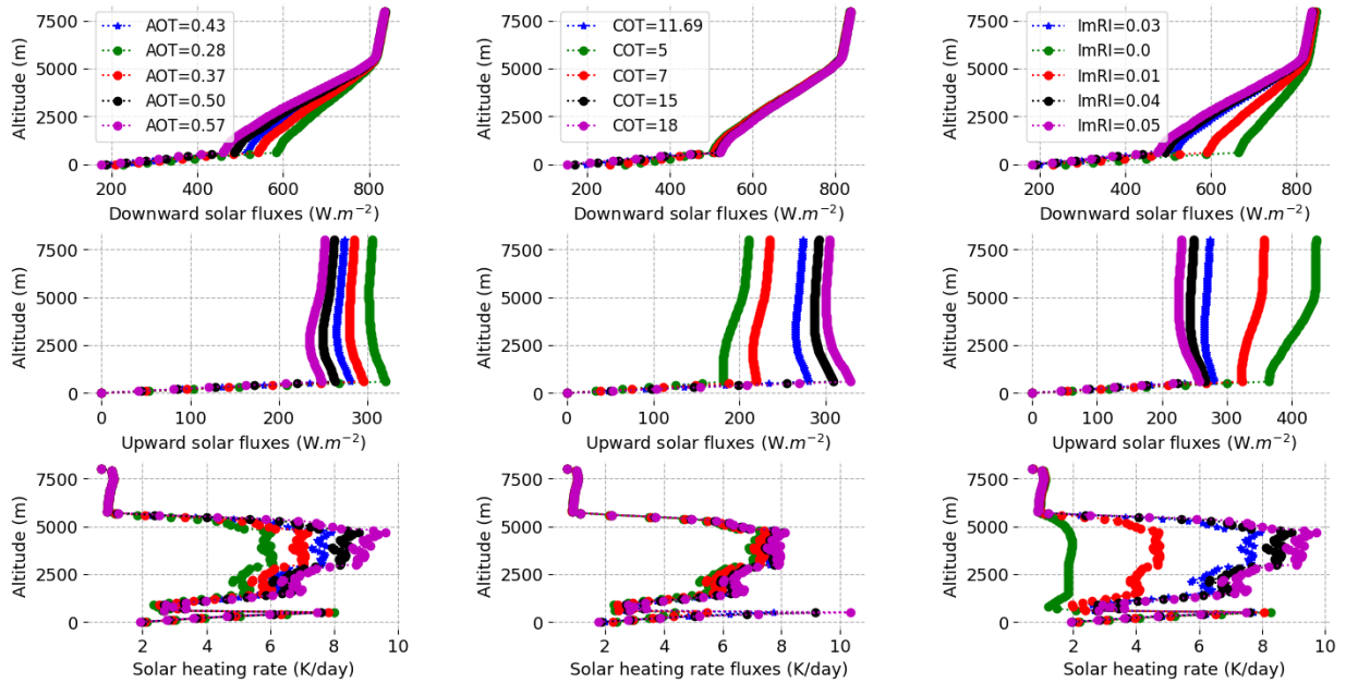
Figure 2: Impact of aerosol and cloud parameter changes on simulated solar radiation: downward (top row), upward 375 irradiances (middle row), and heating/cooling rates (bottom row). Figures a, c and g show the impact of AOT variations. Figures b, e and h show the impact of COT variations. Figures c, f and i show the impact of aerosol absorption variations evaluated by changes in the aerosol imaginary refractive index referred as “ImRI”. The blue curve represents the reference case. The imaginary part of the complex refractive index (see Figure c) of 0., 0.01, 0.03, 0.04 and 0.05 respectively correspond to aerosol single scattering albedo values of 1.00, 0.95, 0.85, 0.81 and 0.78 at 550 nm.
