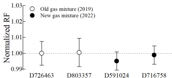
240 Figure 6. Long-term stability of the 10 μmol mol -1 acetonitrile in the Performax cylinders. Note that the y-axis and x-axis represents the normalized response factor (RF) and cylinder numbers, respectively, and the error bars show expanded uncertainties ( k = 2 ).
