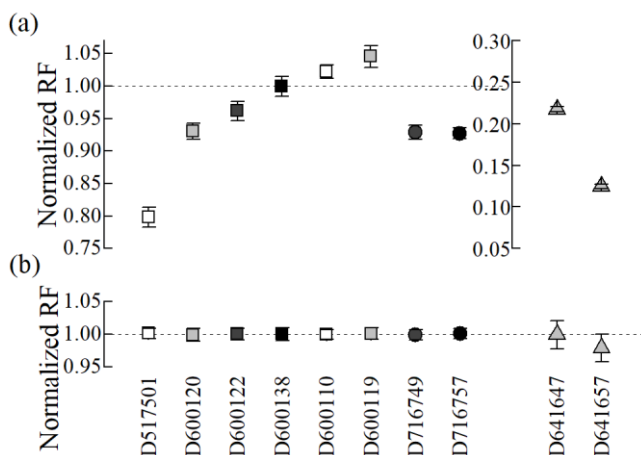
160 Figure 2. Verification results of (a) acetonitrile and (b) hexane gas mixtures at 1 \text{ nmol mol}^{-1} (white), 3 \text{ nmol mol}^{-1} (grey), 5 \text{ nmol mol}^{-1} (dark grey), and 10 \text{ nmol mol}^{-1} (black) in the Experis (rectangle), Performax (circle), and Untreated (triangle) cylinders. Note that
