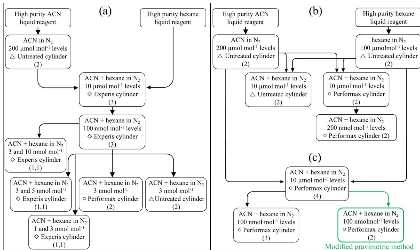
105 Figure 1. Schematic diagram of the preparation of the acetonitrile gas mixtures with the target amount fractions in specified cylinders (a) by conventional gravimetric method, (b) by conventional gravimetric method for adsorption loss evaluation and (c) by 110 modified gravimetric method. The number in parentheses indicates the number of cylinders prepared at each level.
