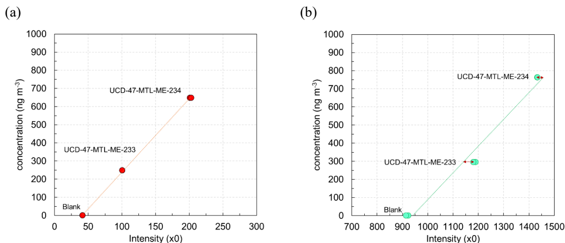
245 Figure 3: Example calibration curves (a) for Fe showing a strong linear relationship ( r^2 = 0.99 ) and (b) for K indicating the deviation of the linear curve fit for the data points. Residuals in (b) are indicated by red arrows (+24 % for ME-233 and -5 % for ME-234), standard error of the slope and intercept are 7 % and 10 %, respectively ( r^2 = 0.97 ). Instrument response data (intensity x0) is plotted on the x-axis and elemental loadings (scaled with sample spot area and the sampled air volume) on the y-axis because standard 250 uncertainty of the ME-233 and ME-234 is larger than the precision (random variation) of the instrument (see text below).
