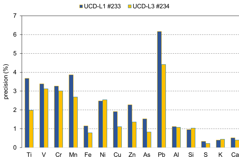
Figure 4: Average relative precision (standard deviation divided by mean) of 30 replicate check standard measurements using two different ME-RMs produced by UCD for 15 elements.
