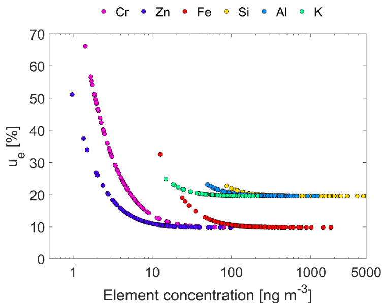
320 Figure 6: Relative expanded uncertainty ( u_e ) of the PX-375 exemplarily for Cr, Zn, Fe, Si, Al and K as a function of the element concentration measured during the Remich field campaign in Luxembourg in 2023 (scale of x-axis is logarithmic, time resolution of the instrument was two hours).
