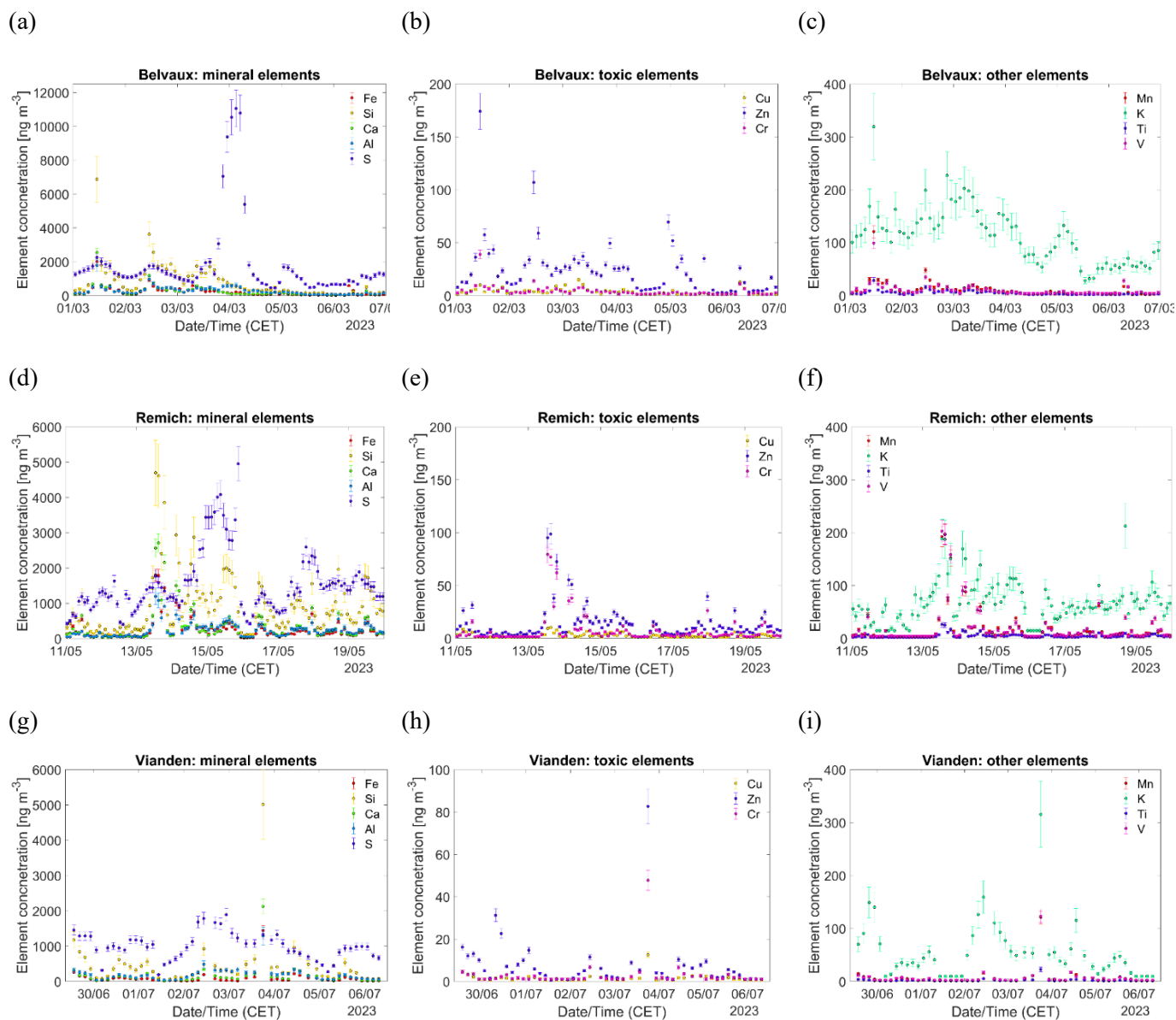
370 Figure 7: Measured timeseries of MAEs, HAEs and OEs by the PX-375 during the three field campaigns at (a-c) Belvaux, (d-f) Remich and (g-i) Vianden in Luxembourg during spring and summer 2023. The error bars denote expanded measurement uncertainties u_{e_i} derived for each data point.
