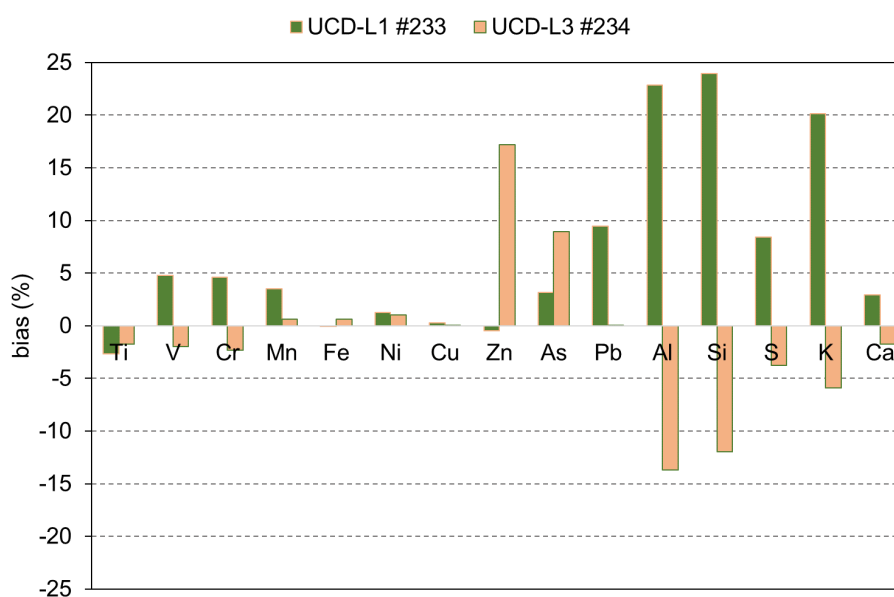
Figure 2: Instrumental bias (relative average deviation) derived from 30 replicate check standard measurements using two different ME-RMs produced by UCD for 15 elements.
