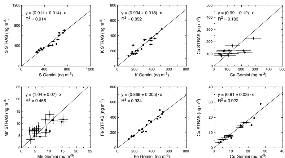
Figure 5: Scatterplots of elemental concentrations of main elements detected by PIXE in PM_{2.5} samples simultaneously collected by STRAS and Gemini on polycarbonate (pore size: 0.8 \mu m ). In each plot the fitted correlation line, together with the correlation coefficient, is also shown.
