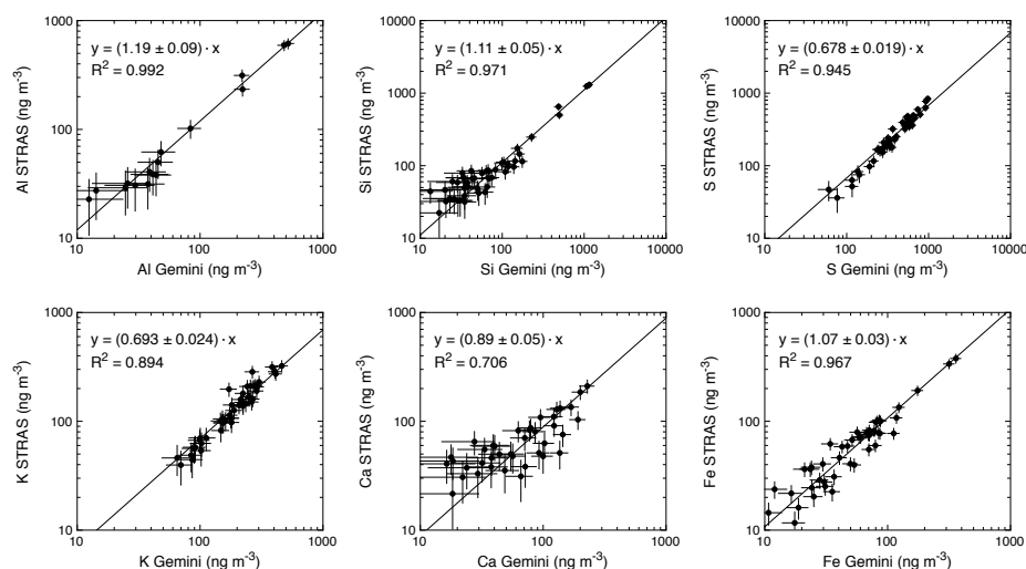
Figure 7: Scatterplots of elemental concentrations of main elements detected by PIXE in PM 1 samples collected in parallel by STRAS (on polycarbonate 0.8 μm membranes) and by Gemini (on ring supported Teflon filters). STRAS concentrations are daily averaged to match the Gemini time resolution. In each plot the fitted correlation line, together with the correlation coefficient, is also shown.
