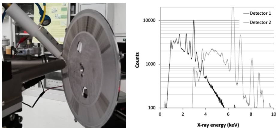
Figure 2: The STRAS sampler during PIXE analysis at the INFN LABEC external beam setup (on the left). PIXE spectra of a 1-h PM 10 STRAS sample, simultaneously obtained using a 3 MeV proton beam in 100 s at 150 nA (on the right).
