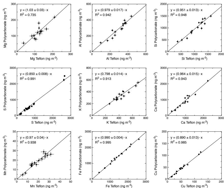
Figure 3: Scatterplots of elemental concentrations of main elements detected by PIXE in PM 10 , simultaneously collected by the dual channel Gemini sampler on Polycarbonate 0.8 and Teflon membranes. In each plot the fitted correlation line, together with the correlation coefficient, is also shown.
