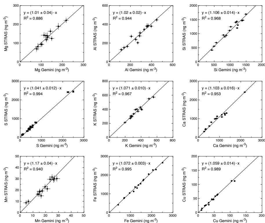
Figure 4: Scatterplots of elemental concentrations of main elements detected by PIXE in PM 10 samples simultaneously collected by STRAS and Gemini on polycarbonate (pore size: 0.8 μm). In each plot the fitted correlation line, together with the correlation coefficient, is also shown.
