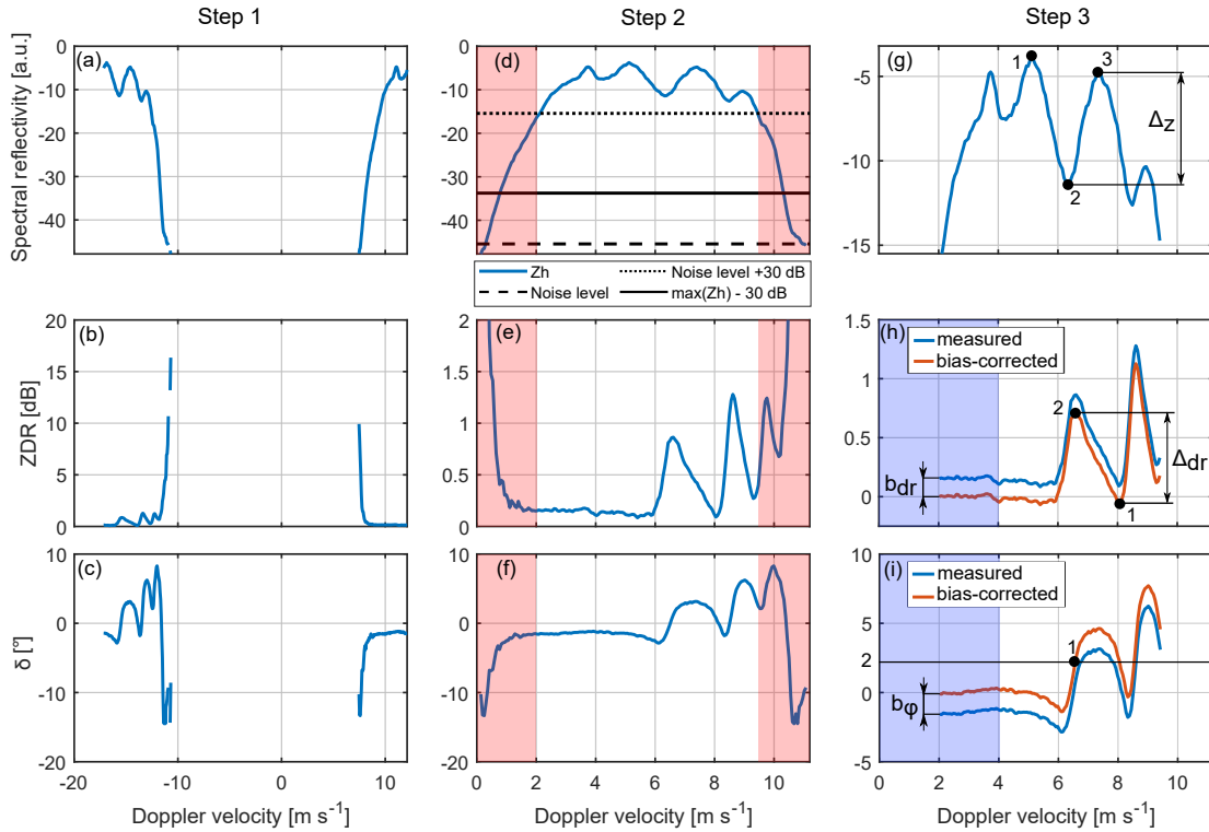
Figure 1. Processing of an individual spectral set. The case was arbitrary chosen from the dataset from location 1. This figure is provided only to illustrate the processing steps. Upper, middle, and lower rows correspond to spectral reflectivity, spectral differential reflectivity, and spectral backscattering differential phase shift, respectively. The left column shows spectra after the thresholding. The middle column shows alias-corrected spectra. This column also shows the selection of spectral lines based on SNR (Sec. 3.1). The red-shaded areas mark spectral lines non-fulfilling the requirements and therefore excluded from the analysis. The dashed line shows the noise level. The dotted line shows the 30 dB SNR level. The solid line shows the level 30 dB lower than the maximum spectral line. The right-most column illustrates the bias correction (Sec. 3.2) and the utilization of resonance effects as explained in Sec. 3.3. The blue solid lines in the right-most column corresponds to spectra after the SNR selection. Red lines show bias corrected backscattering polarimetric variables.
