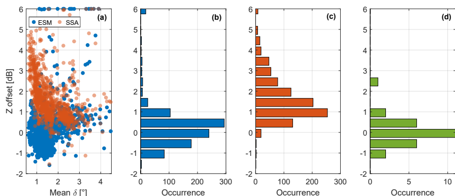
Figure 11. Reflectivity offsets derived using different evaluation approaches. The data from 28 rain events observed at location 1 were used. Panels (a)–(c) show results of the self-consistency method. 975 profiles were used for this method. The results in (c) and red dots in (a) correspond to the self-consistency method with the SSA while the results in (b) and blue dots in (a) were derived using the self-consistency method with the ESM. The panel (d) shows results of the disdrometer-based evaluation. Each dot in (a) and each unit in (b) and (c) corresponds to an offset derived from a single profile. A unit in (d) results from a rain event with at least 2 h duration.
