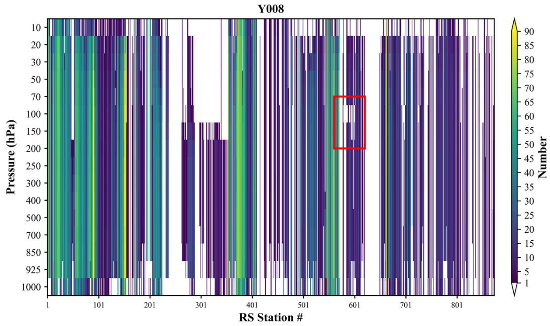
Figure S1: The number of Y008 RO observations matched to each of the 873 RS stations.
