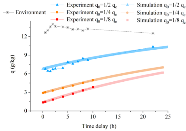
Figure S2-A2 Comparison of humidity variation within the air bag over time in laboratory permeability Experiments No.3 (markers) and diffusion model simulations (lines) for Figures 4 and 5. The experiments cover a range of initial humidities at t = 0 ( q_0 ), from approximately 1/8 * q_e to 1/2 q_e , where q_e denotes environmental humidity.
