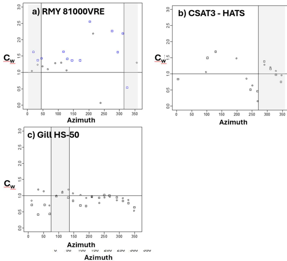
225 Figure 2: Correction factor C_w for a) the RM Young 81000VRE's as a function of azimuthal angle relative to North (upper left), HATS CSAT3's (upper right), and the Gill HS-50's (lower left). The vertical lines and gray shading represent the optimum angles between 315^\circ and 45^\circ as assessed during the experimental design phase (upper left), 270^\circ and 360^\circ (upper right), and between 97^\circ - 187^\circ for the circles, and 277^\circ - 7^\circ for the square symbols (lower left) 270^\circ and 360^\circ (upper right), and 60^\circ and 150^\circ (lower left). For the RM Young 81000's, the circles represent data from the Roberts Island site, and the squares, Union Island. For the CSAT3's, the circles represent the median for 5 sonic anemometers at the 3.45 m height and the squares, 5 sonic anemometers at the 6.90 m height. For the Gill HS-50, the circles represent a sonic on the arm oriented to the East, and the squares, the sonic on an arm oriented to the West, with block medians taken for the correction factors spanning 20^\circ intervals.
