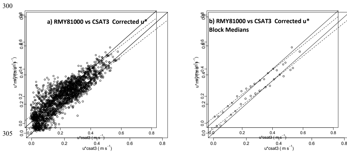
Figure 5: a) Corrected RMY81000 u^* plotted against corrected CSAT3 u^* , Y=0.9384X - 0.03225 m s^{-1} b) Block medians of corrected RMY81000 u^* plotted against corrected CSAT3 u^* , Y=0.9345X + 0.0302 m s^{-1} , Y=0.9138X + 0.0285 .
