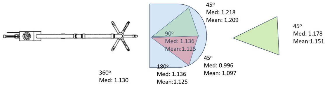
Figure 3: Correction factor C_w as a function of azimuthal angle sectors, for the HATSs CSAT3 data.
