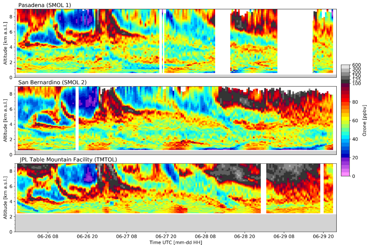
Figure 5. SMOL-1 (top), SMOL-2 (middle), and TMTOL (bottom) measurements during IOP 1.
