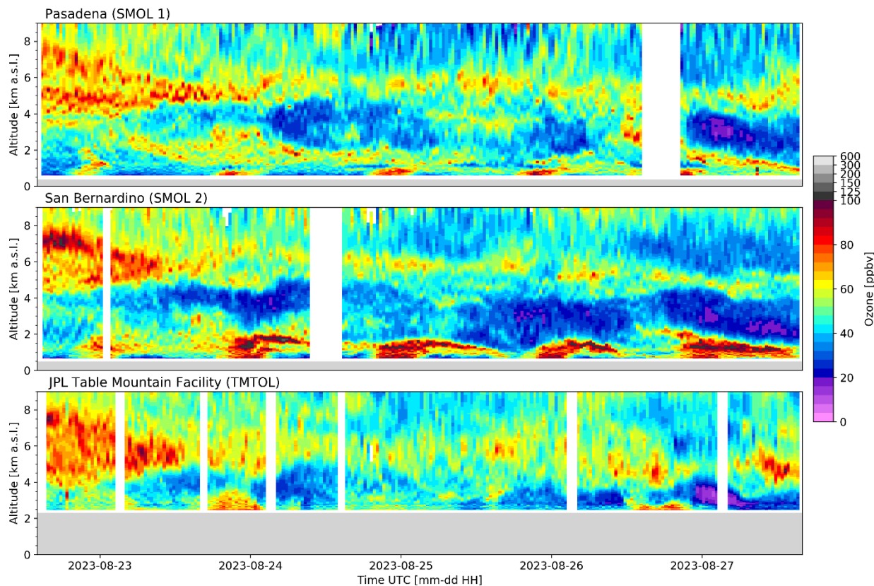
Figure 6. SMOL-1 (top), SMOL-2 (middle), and TMTOL (bottom) measurements during IOP 2.
