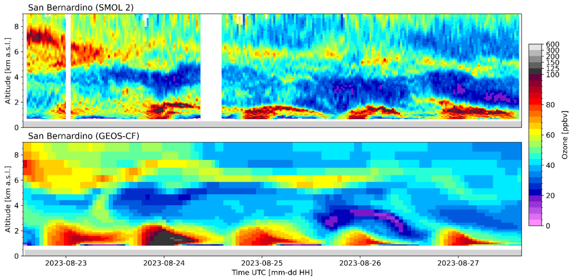
360 Figure 9. Comparison of the results from SMOL-2 during IOP 2 and GEOS-CF. The upper panel shows the measurements by SMOL 2 during IOP 2, while the bottom panel shows the GEOS-CF replay results.
