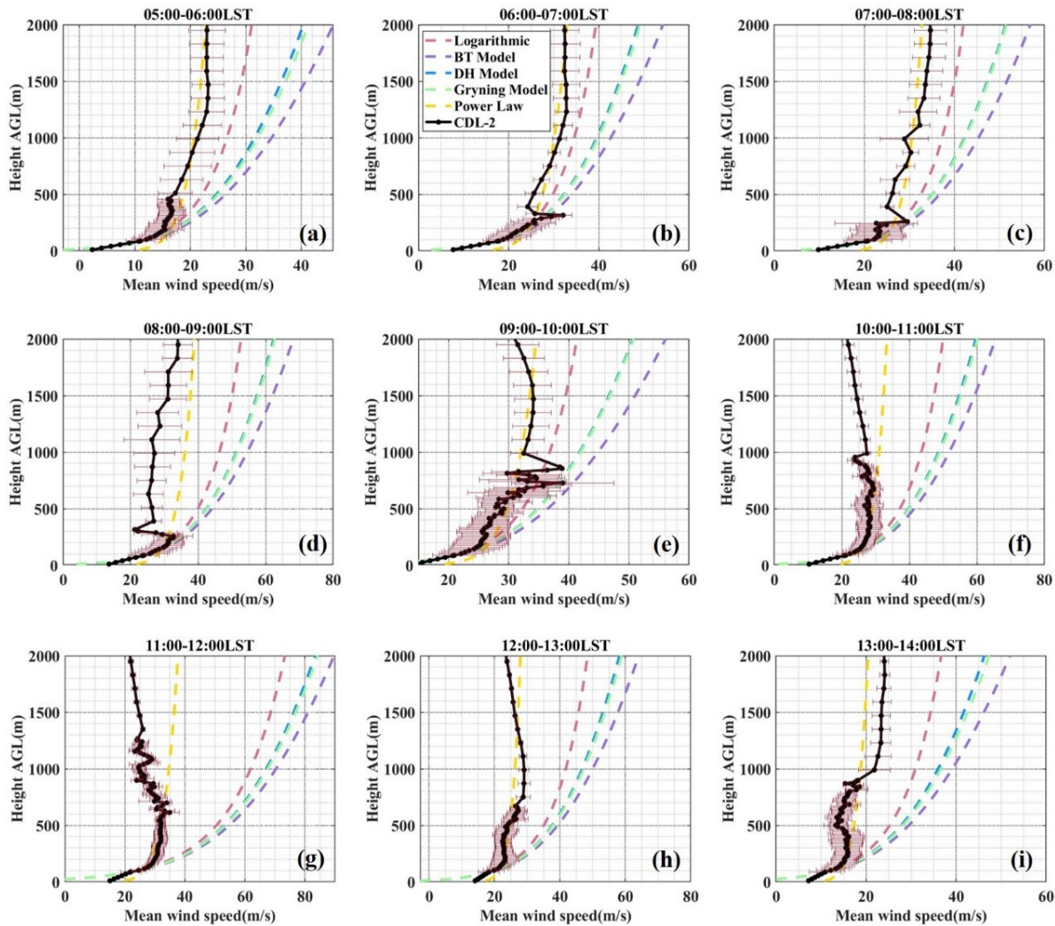
260 Figure 8: No-blind zone wind speed profiles at Position-2 using data fusion method (black dots) and fitted by the logarithmic law (pink dotted line), BT model (purple dotted line), DH model (blue dotted line), Gryning model (green dotted line) and power law (yellow dotted line). The error bars represent the standard deviation of the wind speed in the mean time period shown above.
