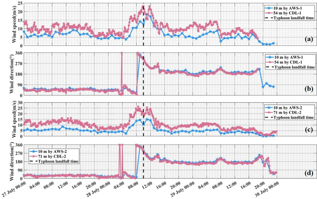
220 Figure 4: Wind speed (a, c) and wind direction (b, d) variation of the CDL lowest detection height (pink squares) and 10 m (blue stars) at Position-1 (a, b) and Position-2 (c, d).
