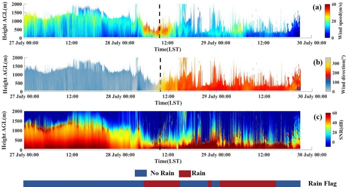
Figure 10: The variation of (a) wind speed, (b) wind direction and (c) SNR measured by CDL-1 during the passage of the Typhoon.
