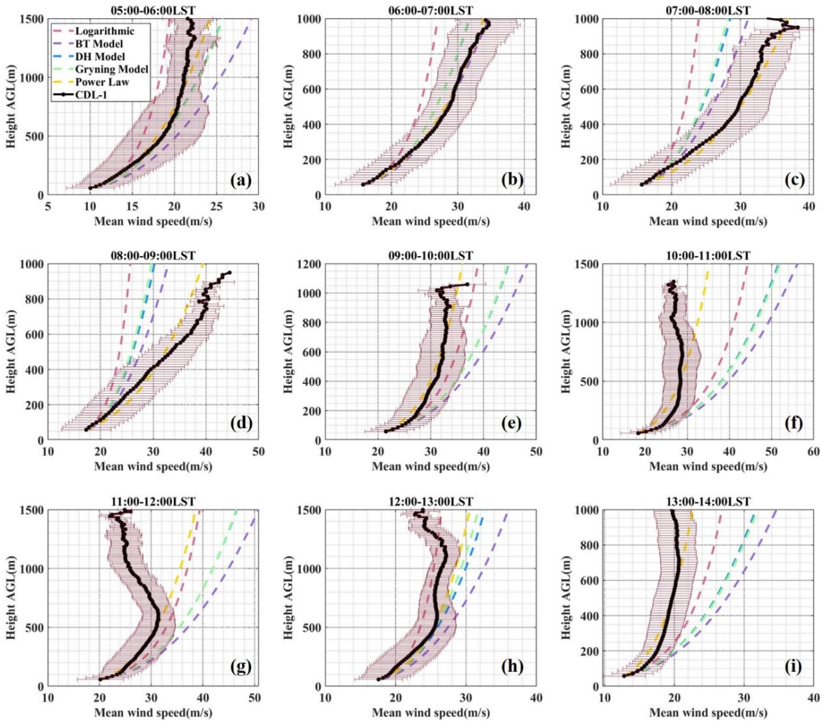
250 Figure 7: Mean wind speed profiles measured by CDL-1 (black dots) and fitted by the logarithmic law (pink dotted line), BT model (purple dotted line), DH model (blue dotted line), Gryning model (green dotted line) and power law (yellow dotted line). The error bars represent the standard deviation of the wind speed in the mean time period shown above.
