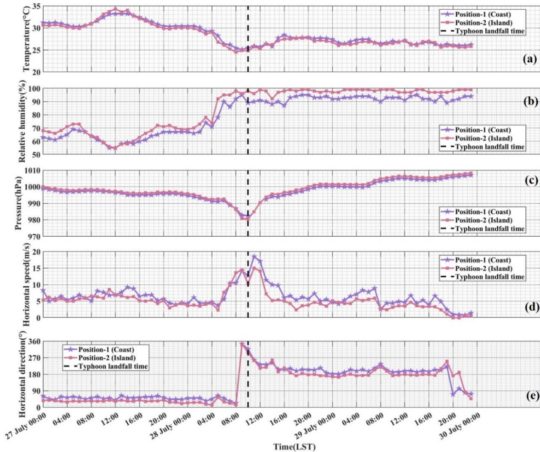
Figure 3: The variation of (a) air temperature, (b) relative humidity, (c) air pressure, 10-min mean (d) wind speed and (e) wind direction measured by AWS at two locations.
