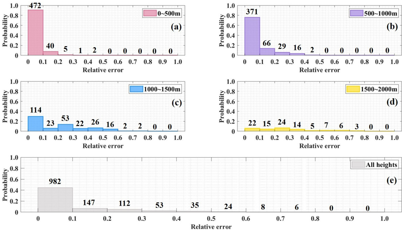
275 Figure 9: The probability distribution of relative errors at (a) 0 ~ 500 m, (b) 500 ~ 1000 m, (c) 1000 ~ 1500 m, (d) 1500 ~ 2000 m 280 and (e) all heights estimated by the power law model. And the probabilistic frequencies of each group are labelled with black 285 numbers on the histogram.
