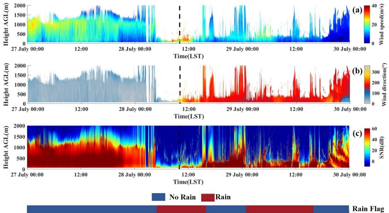
300 Figure 11: The variation of (a) wind speed, (b) wind direction and (c) SNR measured by CDL-2 during the passage of the Typhoon.
