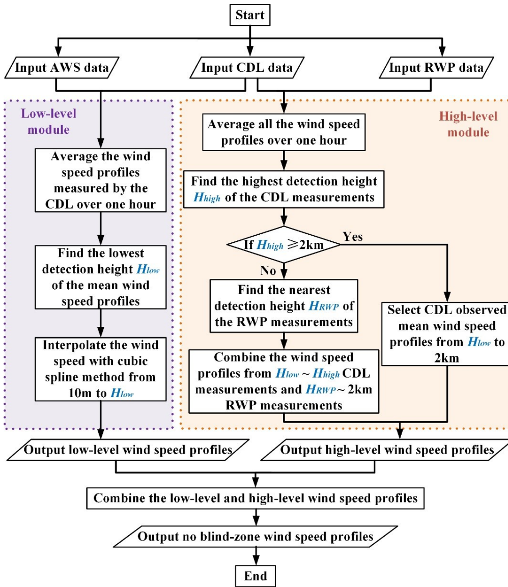
185 Figure 2: The flowchart of the no-blind zone wind speed profile retrieval.
