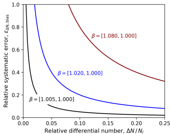
335 Figure 4: Relative error in the differential number measurement due to systematic bias, \beta , as a function of the relative differential number ( \Delta N/N ), for 0.5%, 2%, and 8% bias in the first channel and no bias on the second.
