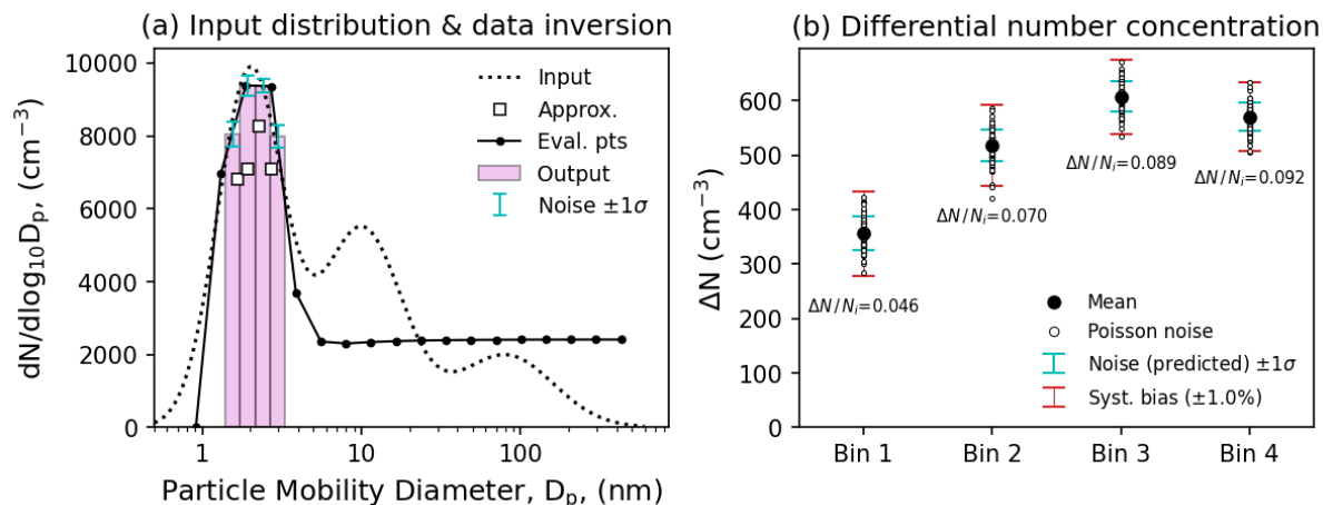
Figure 5: Simulated data inversion example with a 3-mode lognormal distribution. a) Output (numerical data inversion, bars) and 385 approx. (approximate data inversion, square points) vs. input size distribution (dots) for noisy CPC FARM signals. Blue error bars represent 1\sigma of instrument noise. Black points are the 20 evaluation points used in the particle size vector used in the kernel matrix Eq. (5). b) The resulting differential number across the instrument channels (mean values and noise due to random Poisson counting error), as well as systematic error due to \pm 1\% bias in the signal of the first channel of each bin. \Delta N/N_i values indicate the relative 390 differential number concentration in each bin. A sample flow rate of 0.3 \text{ L min}^{-1} and a sampling time interval of 5 s were used in this example.
