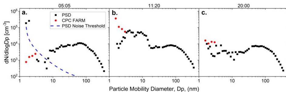
Figure 7: Size distribution of a single five-minute PSD scan and five-minute CPC FARM averaged from (a) 5:05 – 5:10, (b) 11:20 – 11:25, and (c) 20:00 – 20:05
