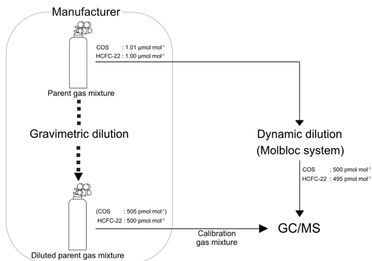
1 2 Figure 6: Scheme for validating the dilution accuracy of our dynamic dilution method.
