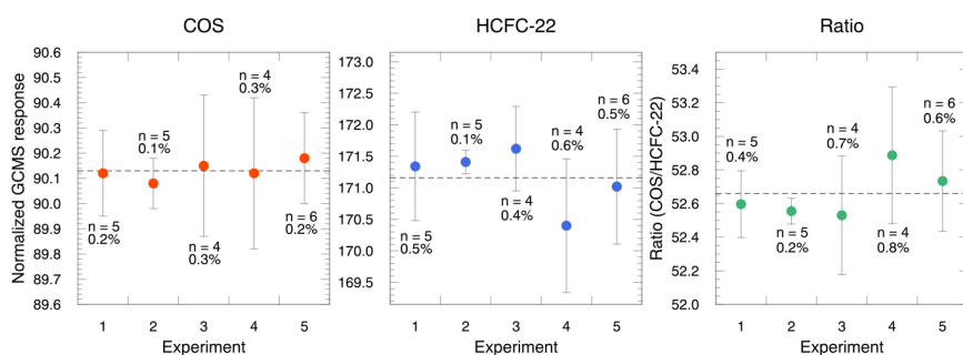
3 Figure 4: Repeatability and reproducibility of our dynamic dilution method for generating gas 4 mixtures containing COS and HCFC-22. Vertical error bars indicate the standard deviation of the 5 normalised values obtained in each experiment. The number of measurements and relative 6 standard deviation are shown for each average plot.
