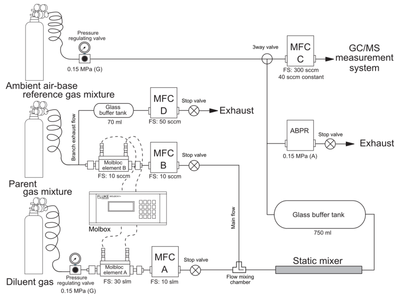
2 Figure 1: Schematic of the dynamic dilution system. The thermal-based mass flow controllers and 3 automatic back-pressure regulator are denoted as MFC and ABPR, respectively. Full-scale 4 volume flow rates (FS) that determine the flow precision are provided for each Molbloc element 5 and thermal-based mass flow controller. The ambient-air-base reference gas mixture was used to 6 calibrate the GC/MS system (see details in Section 2.4).
