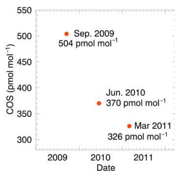
Figure 3: Time-series variation of the COS mole fraction in a dry reference gas mixture balanced with high-purity nitrogen during long-term storage in a non-passivated high-pressure aluminium cylinder.
