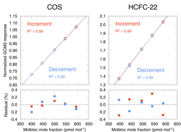
11 12 Figure 5: Dilution linearity of the dynamic dilution method for COS and HCFC-22 in response to 13 increases or decreases in the generated target gas mole fractions. The normalised GC/MS 14 responses (upper) and residuals from the fitting line determined by linear least squares (bottom) 15 are shown as a function of the mole fraction calculated from the average mass flow rates during 16 the sample concentration process measured by the Molbloc system.
